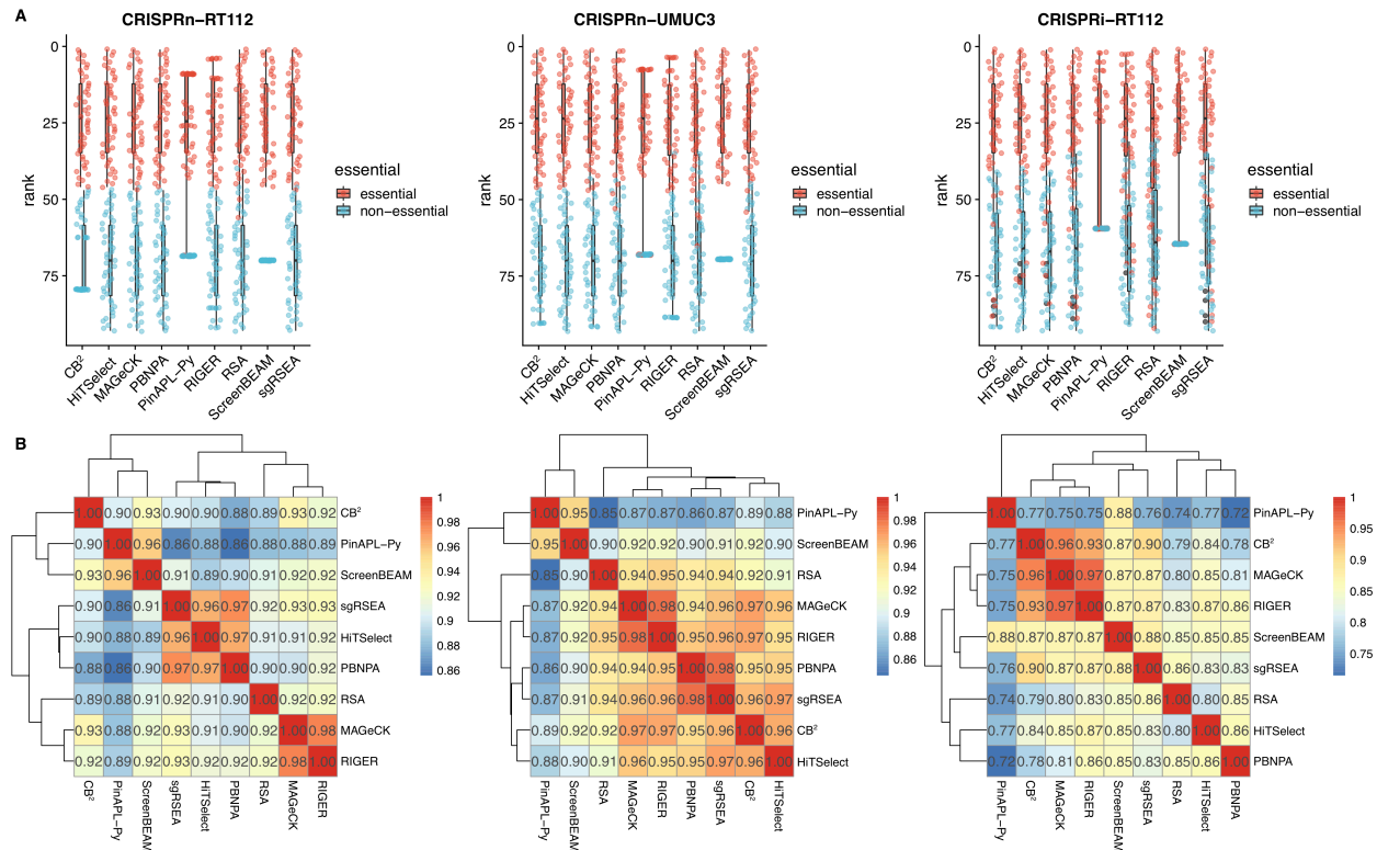
Supplemental Figure 3. Rank Comparison of different methods using three benchmark datasets. (A) boxplots indicate distinction between essential genes and non-essential genes by ranks for each dataset. (B) heatmaps indicate correlations of gene-rankings between analysis methods for each dataset.
