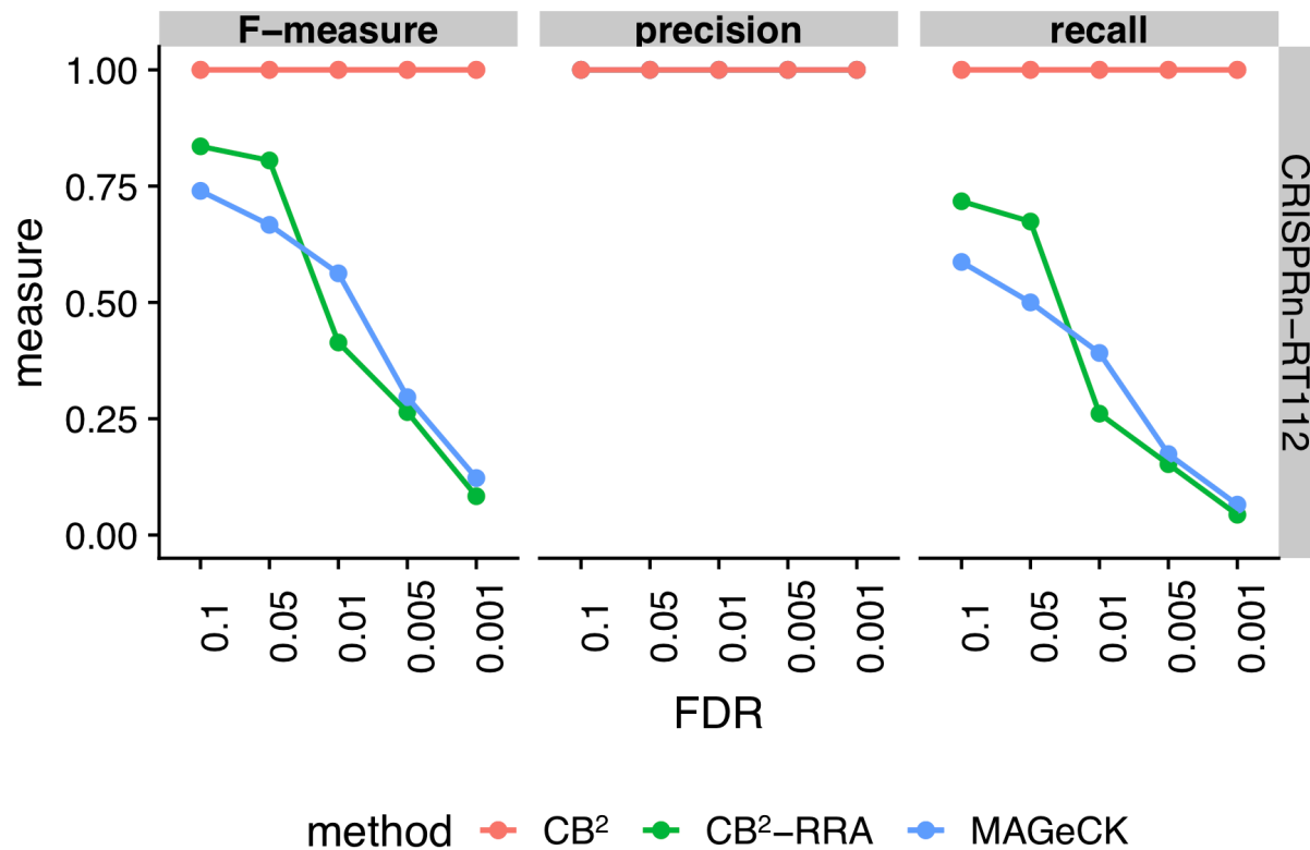
Supplemental Figure 2. F1-score, precision, and recall measurements at different FDR cut-offs across CB 2 -Fisher, CB 2 -RRA, and MAGeCK (RRA). At commonly used FDR cut-offs, CB 2 can identify most of the essential genes with high rates of recall.
