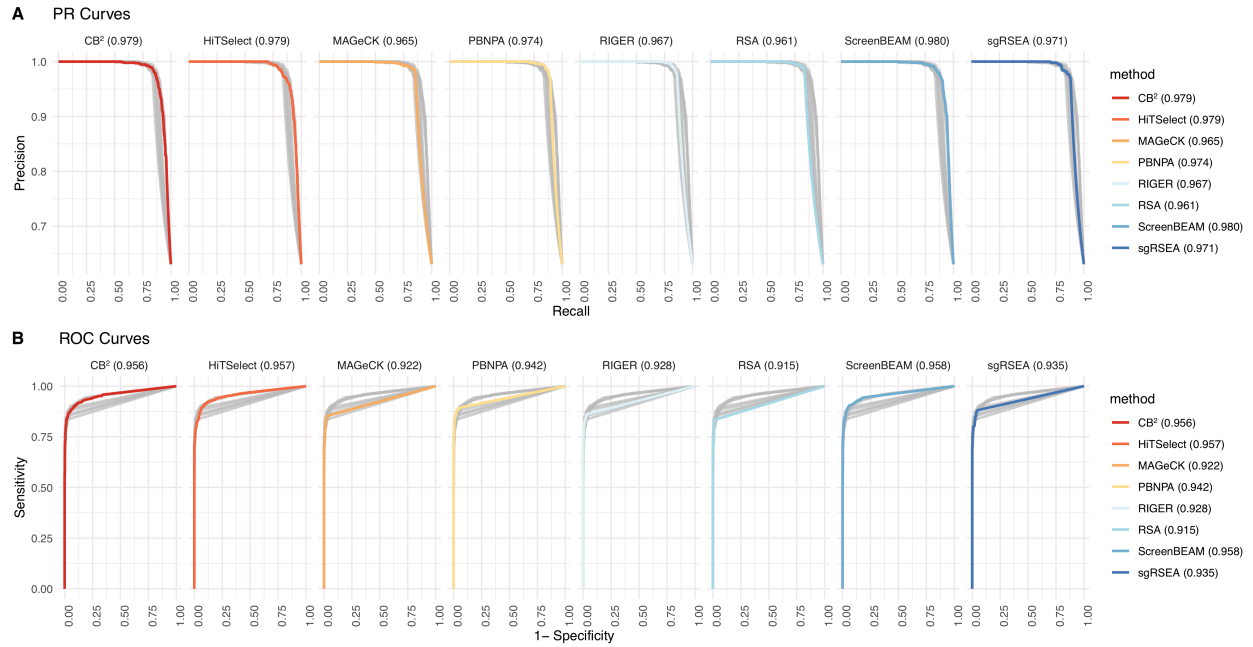
Supplemental Figure 11. PR curve and ROC curve comparison of different methods using CRISPRi-A375 dataset from Sanson et al. (2018). (A) PR curves for each method. A bracket-surrounded number right to a name of the method indicates AUC of the corresponded PR curve of the method. (B) ROC curves for each method. A bracket-surrounded number right to a name of the method indicates AUC of the corresponded PR curve of the method.
