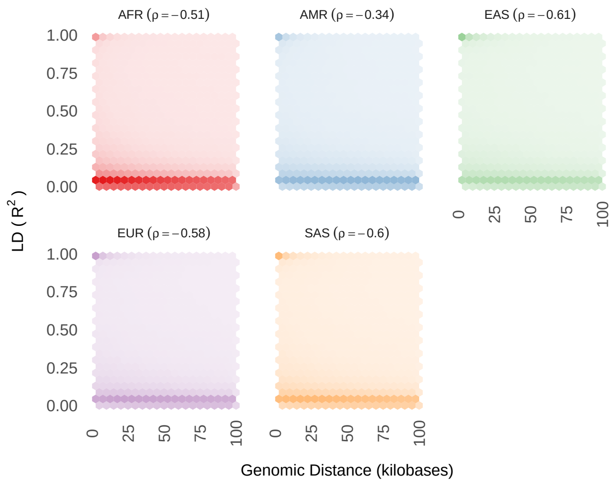
Supplemental Figure 4. Scaling of LD with genomic distance shows moderate anti-correlation for all super-populations. Figure 3 shows combined LD scaling and observed Hi-C contact frequency scaling by cell line.
