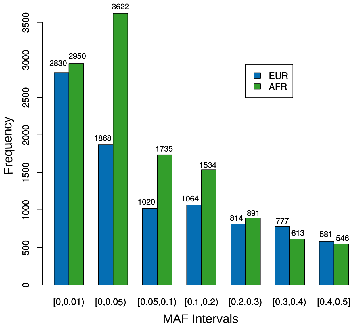
Supplemental Figure S7: MAF distribution for European and African populations in the simulated data.
