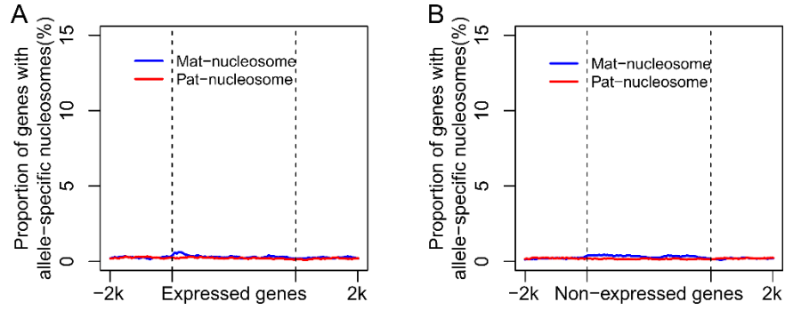
Figure S8. The distribution of parent-of-origin nucleosomes at expressed genes/non-expressed genes in endosperm and its up and down 2kb regions. Blue line represents the maternal specifically positioned nucleosome (mat-nucleosome) and red line represents the paternal specifically positioned nucleosome (pat-nucleosome). Expressed genes in endosperm ( \text{FPKM} \geq 1 ), Non-expressed genes in endosperm ( \text{FPKM} < 1 ).
