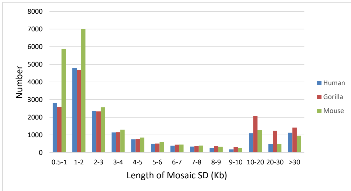
Figure S6: The length distribution of mosaic SDs identified by SDquest in human (hg19 assembly), gorilla (gorGor5 assembly), and mouse (mm8 assembly) genomes.
