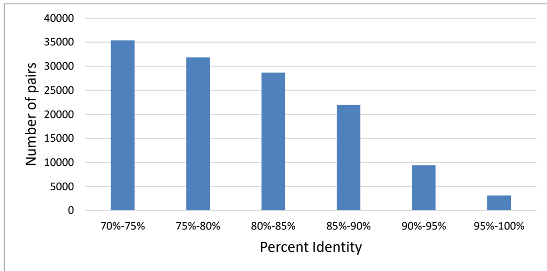
Figure S1: Number of pairwise alignments (depending on the percent identity) for 130,405 pairwise alignments among putative SDs in the human genome (hg19 version) identified by SDquest.
