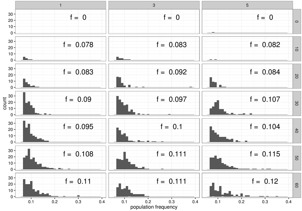
Supplementary Fig. 8: Population frequencies of P-element insertions during the hot invasion. Histograms show the population frequencies of P-element insertions during the invasion. Generations are in the right panel and replicates in the top panel. Note that the average population frequency ( f ) increases during the hot invasion.
