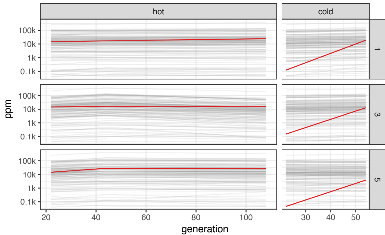
Supplementary Fig. 20: Abundance of piRNAs for 121 TE families (23 TIR, 60 LTR, 37 non-LTR and 1 Foldback) during the hot and the cold invasion. Solely P-element piRNAs (red) show a marked increase at cold conditions. Families with fewer than 40 piRNAs per million miRNAs are not shown.
