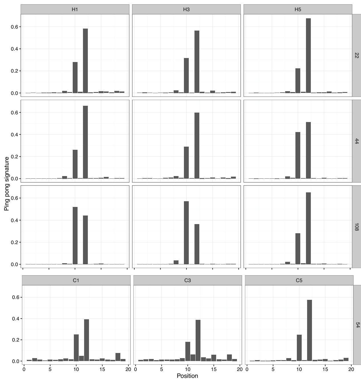
Supplementary Fig. 18: Ping-pong signature of P-element piRNAs in hot and cold evolved populations. Data are shown for all three replicates of the hot (H1, H3 and H5) and cold (C1, C3, C5) evolved populations. Due to a low number of piRNAs we could not compute ping-pong signatures for any replicate of the cold invasion at generation 22.
