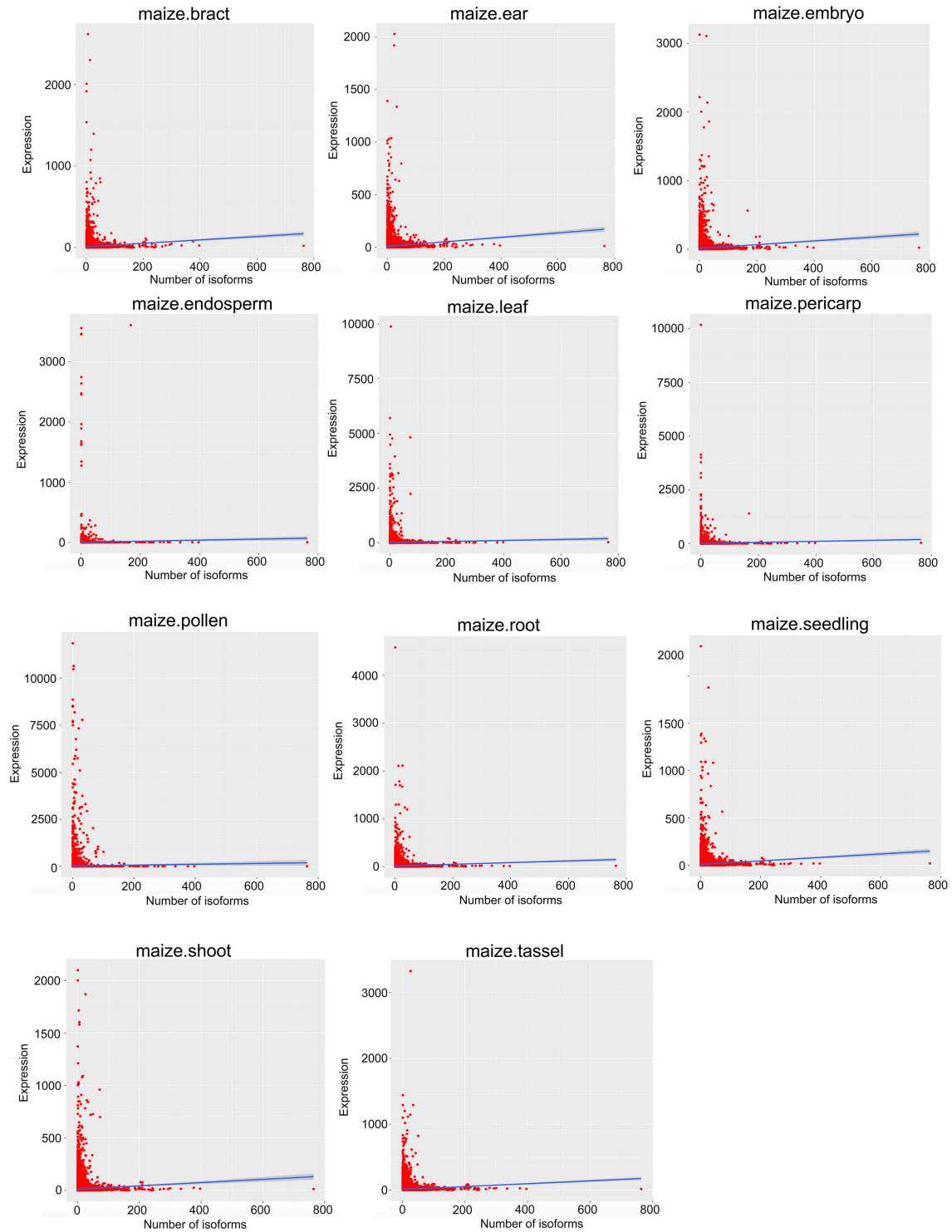
Supplemental Figure S32: Correlation between expression value and number of isoforms among different tissues in maize.
