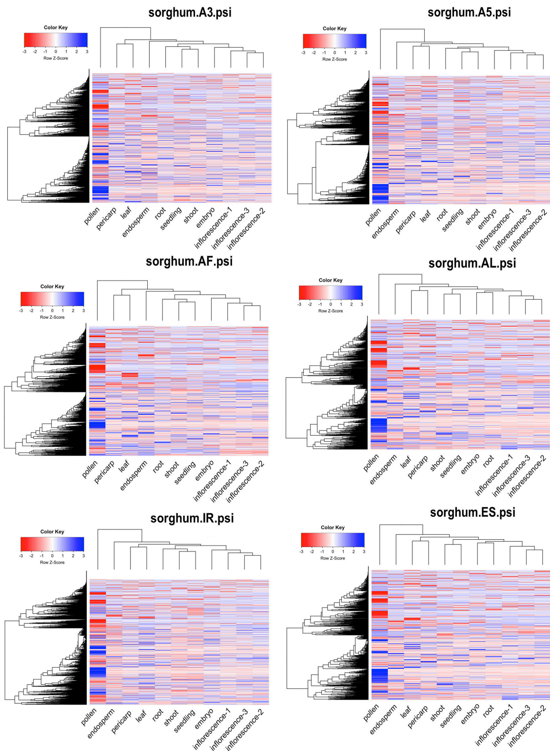
Supplemental Figure S3: Heatmap of PSI distribution of types of splicing events among different tissues in sorghum.
