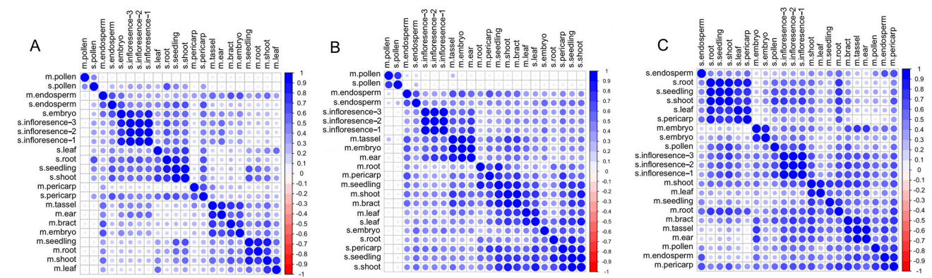
Supplemental Figure S25: Correlation matrix of TFs in maize A genome only, B genome only, and shared by A and B genome.
