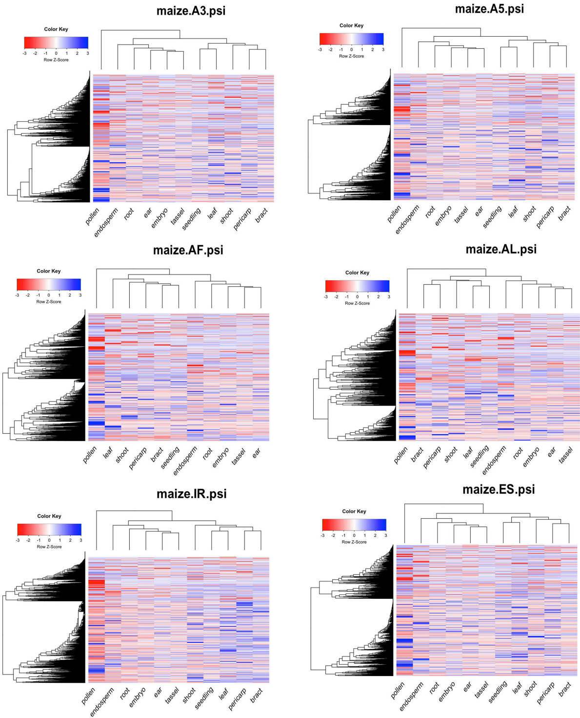
Supplemental Figure S2: Heatmap of PSI distribution of types of splicing events among different tissues in maize.
