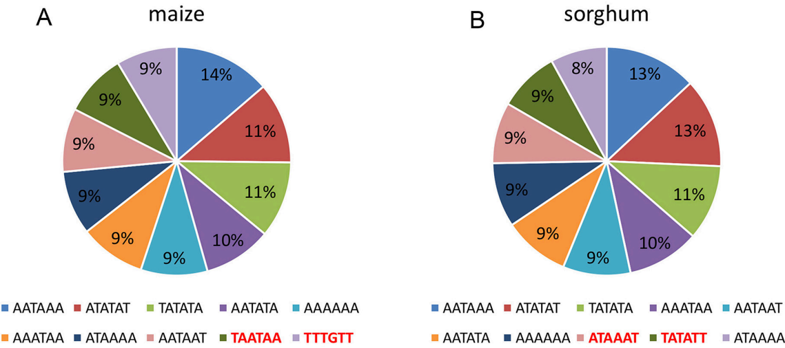
Supplemental Figure S19: APA motifs in maize and sorghum orthologous genes.
