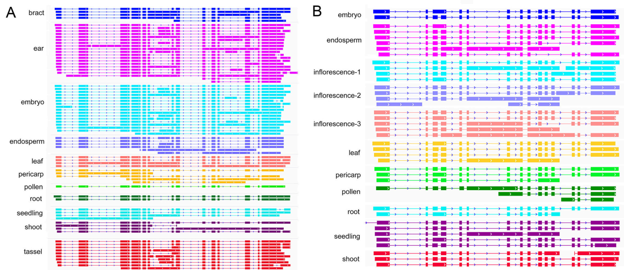
Supplemental Figure S18: Example of different polyA cleavage sites in maize and sorghum isoforms.
