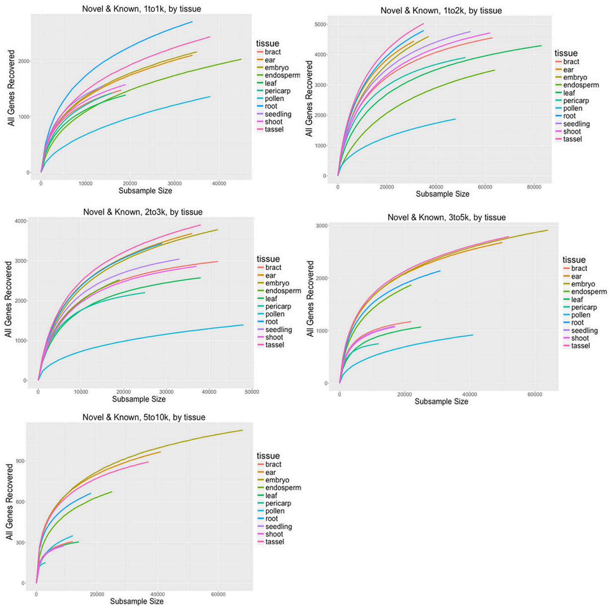
Supplemental Figure S15: Rarefaction analysis of genes in each tissue of maize across size fractions.
