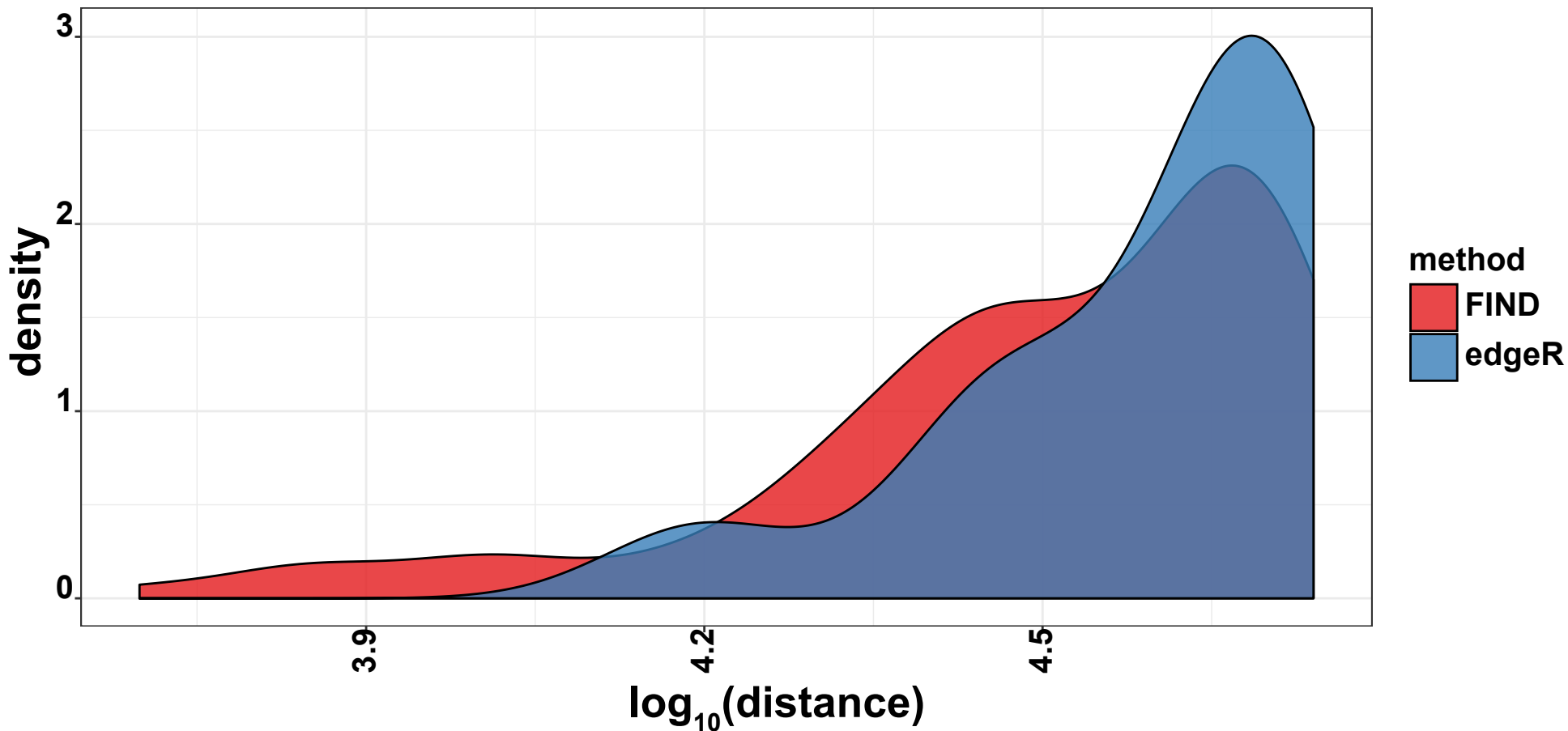
Figure S7. The distribution of the distance between the DCI detected by FIND and edgeR.
