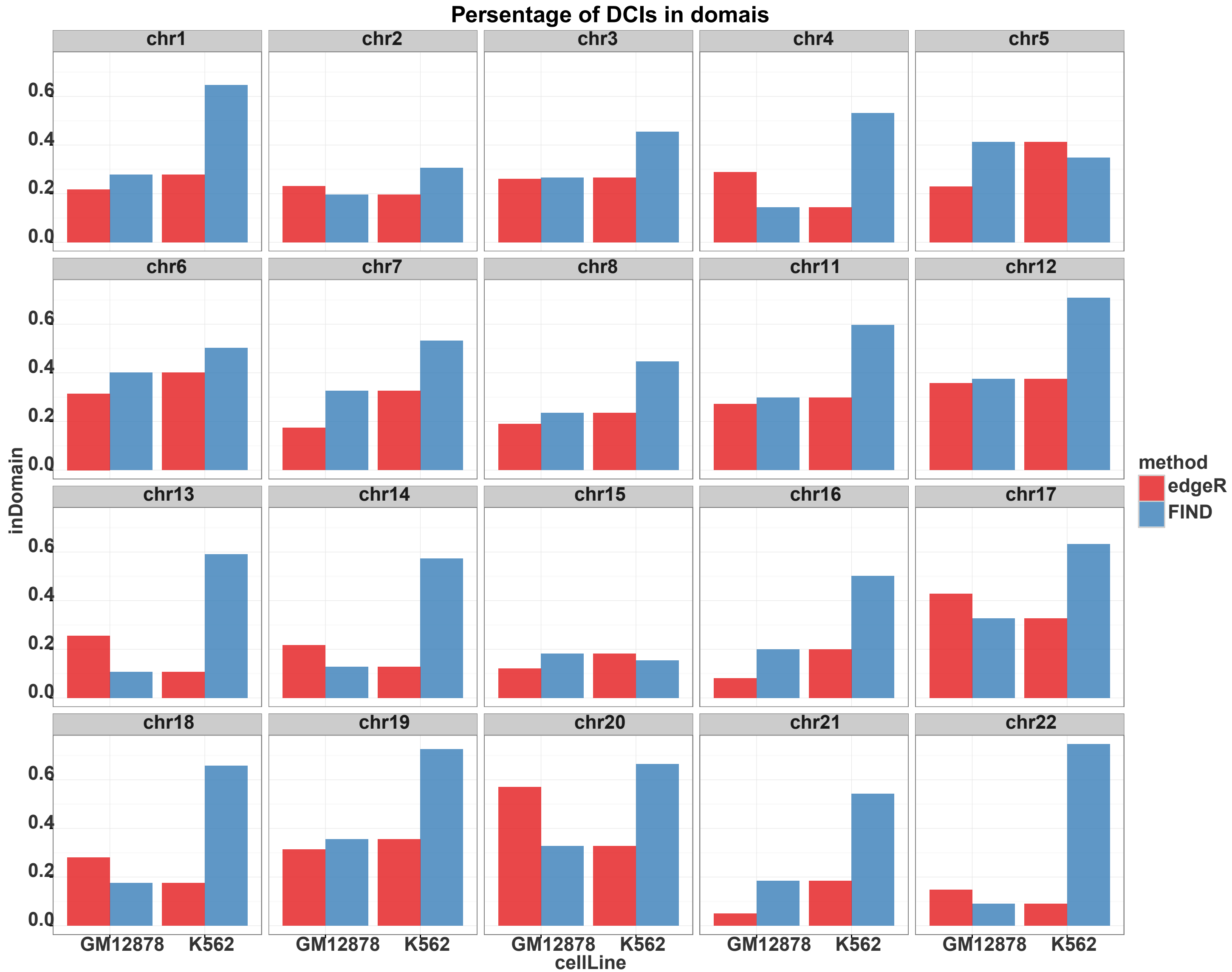
Figure S5. Comparison of the percentage of the DCI located within TADs between FIND and edgeR.
