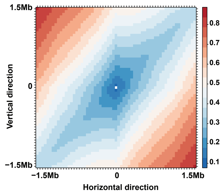
K562 Chr22 variogram (50kb)
