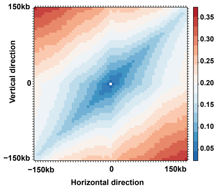
K562 Chr22 variogram (5kb)
