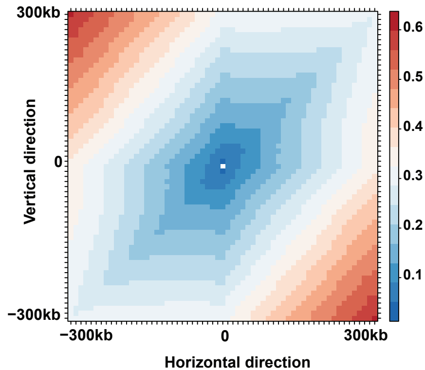
K562 Chr22 variogram (10kb)
