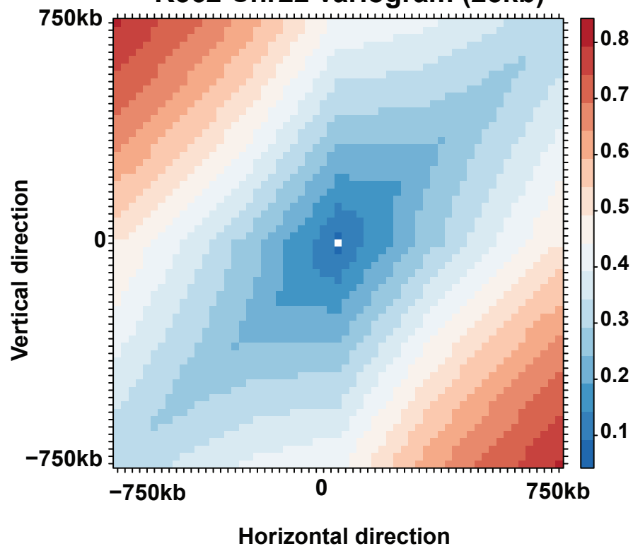
K562 Chr22 variogram (25kb)
