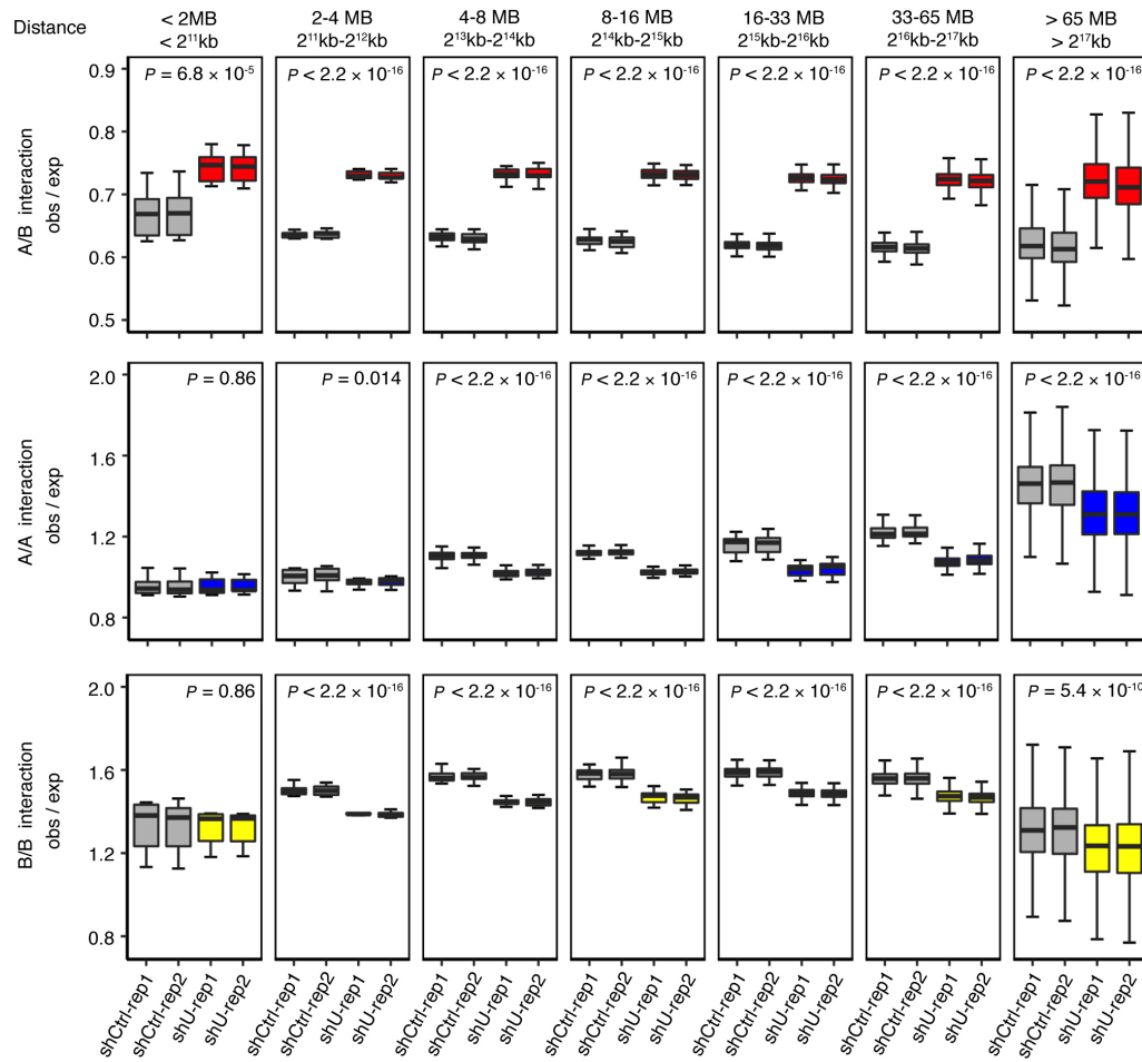
Supplemental Figure S5. Long-range interactions among compartments in different distance ranges. Boxplots show interactions of two replicates in control and knockdown. In all distance ranges, interactions between A and B compartments (upper), among A compartments (middle) and among B compartments (lower) were compared. P values were obtained by ANOVA.
