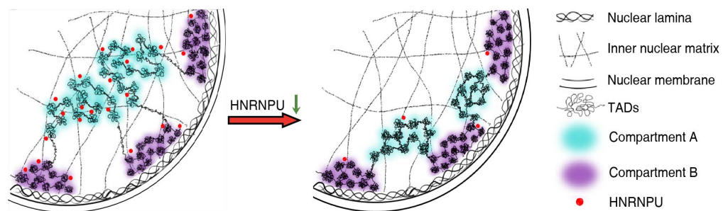
Supplemental Figure S11. A hypothetical model for how HNRNPU can maintain 3D genome architectures including compartments and TADs.
