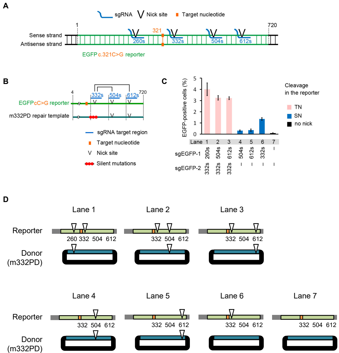
Supplemental Figure S2. Nucleotide substitution by tandem nick (TN) of the reporter gene. (A) Diagram of the EGFPcC>G reporter gene and sgRNAs. (B) Diagram of the repair templates. (C) The nucleotide substitution efficiency as measured by flow cytometry (mean \pm s.d., N=3) is presented. The indicated sgRNAs were expressed with Cas9D10A. m332PD was introduced into the cells as plasmid donors. (D) Schematic of the experiment in C. Nick sites are indicated by inverted triangles. The target nucleotide is indicated by an orange rectangle.
