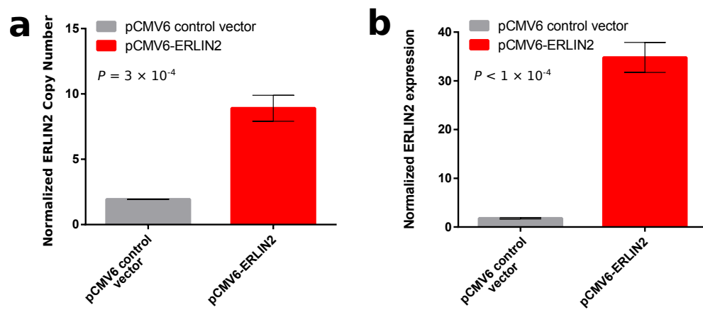
Figure 5: Plots showing the change in ERLIN2 (a) copy number and (b) expression following transfection with ERLIN2 containing and control plasmids.
