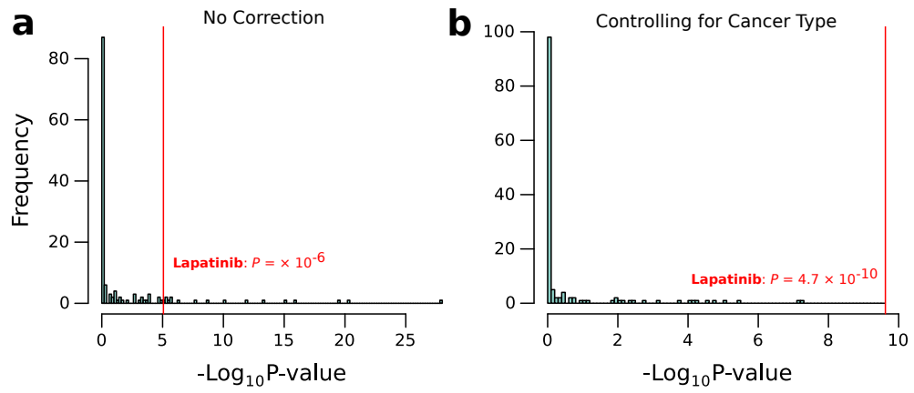
Figure 10: P-value for difference in predicted lapatinib response between ERBB2+ and ERBB2- TCGA samples. These P-values are derived across the entire dataset when (a) calculating the association with no correction or (b) calculating the association when controlling for tissue-of-origin.
