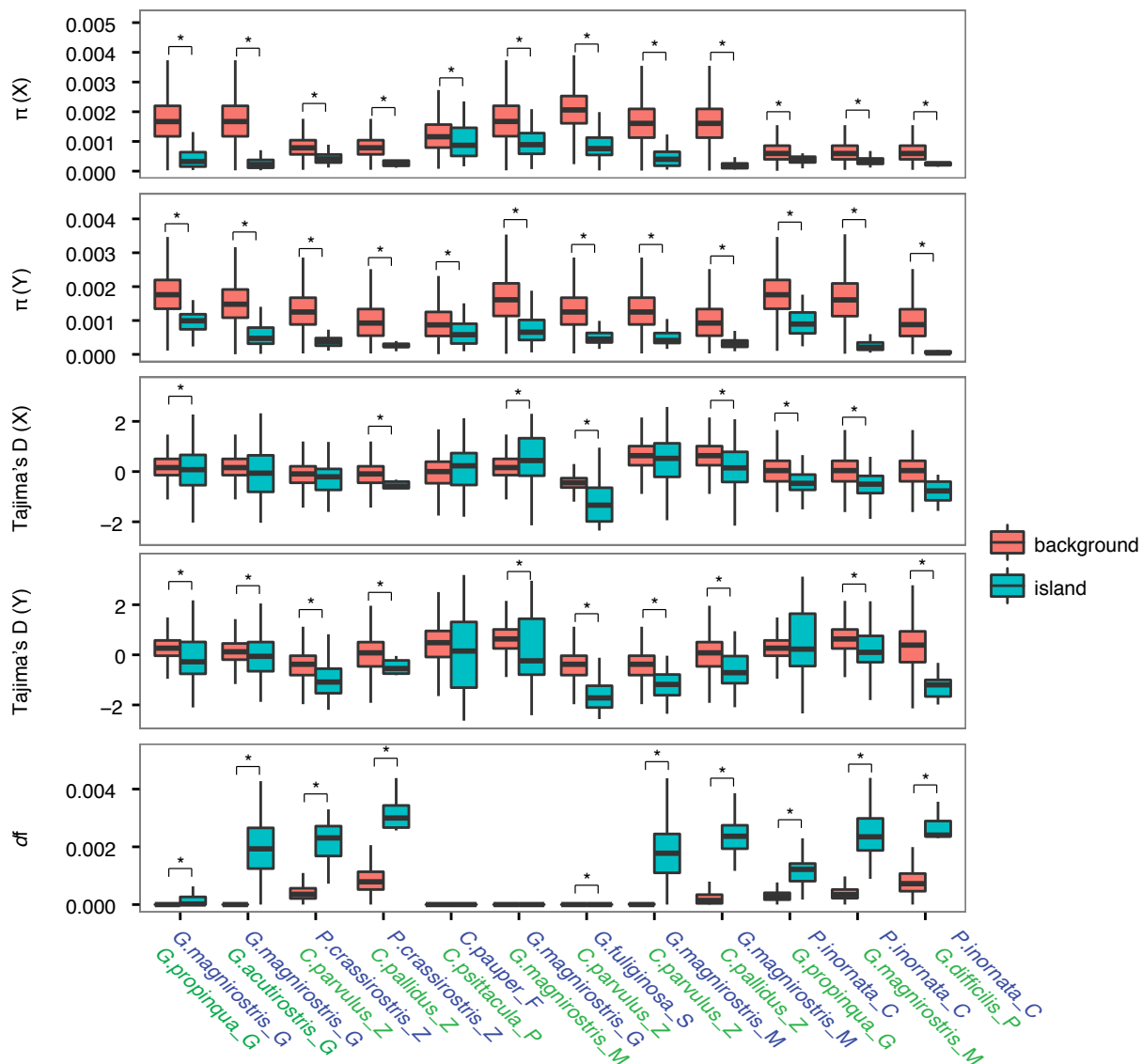
Figure S2. Estimates of genomic parameters among pairs of Darwin's finch species. The two species in each pair are denoted X (species name in blue) and Y (species name in green). Five panels from top to bottom represent nucleotide diversity in species X and Y, Tajima's D in species X and Y, fixed differences between species X and Y. Significance is tested with Wilcoxon rank sum test. *, P < 0.05 .
