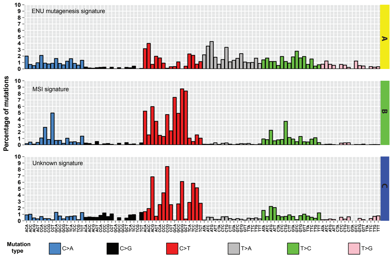
Supp Figure S4. Mutational signatures extracted from ENU-derived CCK-81 and NCI-H508-Cetuximab resistant clones based on the trinucleotide pattern of substitutions and using for each locus the substitution class (C>T, C>A, C>G, A>T, A>C, A>G) and the sequence context immediately 5' and 3' to the mutated base. Signature A is that of the ENU-derived mutations whereas Signature B is that of MSI (microsatellite instability). Signature C is of unknown aetiology.
