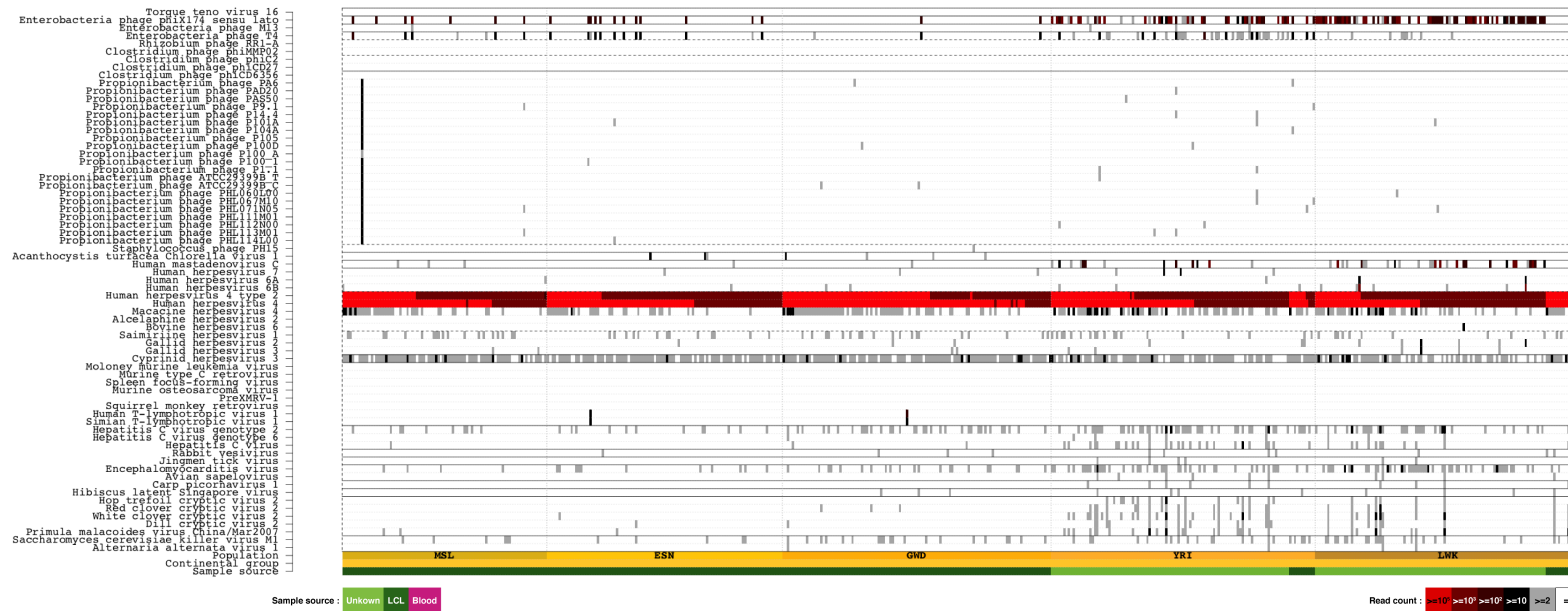
Supplemental Fig 6. Viral sequences found in the 1000GP population BWT (AFR continental group). Individuals are represented on the x-axis. Only virus taxa with greater than 10 reads (black bars) in at least one sample are shown. Samples are ordered by population, source (blood: pink, LCL: dark green, unknown: light green), and total virus load (sum of read counts per virus and sample).
