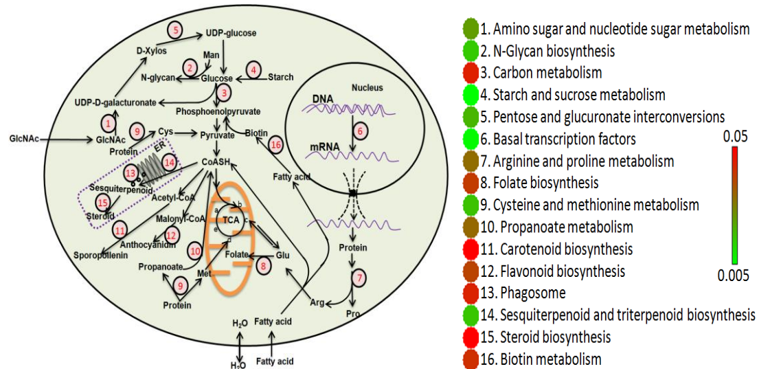
Supplemental figure 4 Analyses of KEGG (Kyoto Encyclopedia of Genes and Genomes) pathways of pollen specific isoforms. Each number represents one pathway of right lists. Color codes indicate p-value. Labels on the TCA cycle: a, oxalocetate. b, citrate. c, \alpha -ketoglutarate. d, succinyl CoA. e, fumaric acid.
