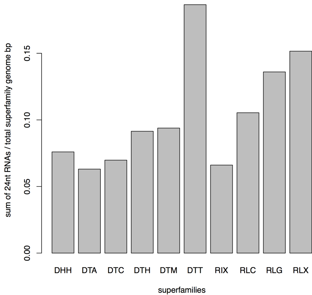
Supplemental Figure 6. Sum of 24nt RNAs from IBI 2010 normalized by total element size sum by transposon superfamily.
