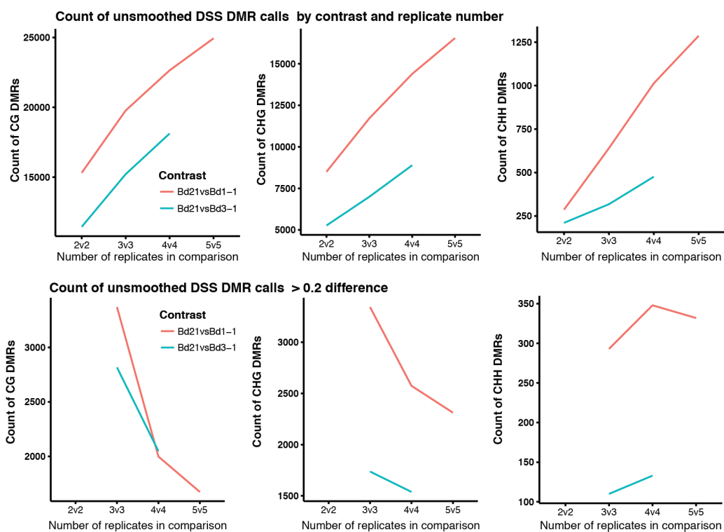
Supplemental Figure 18. Comparisons of unsmoothed DSS results for 2v2, 3v3, 4v4, and 5v5 (Bd1-1 only) replicate comparisons. Plots indicate total number of DMRs called (top panels) and the number of DMRs with differences between accessions > 0.2 (bottom panels).
