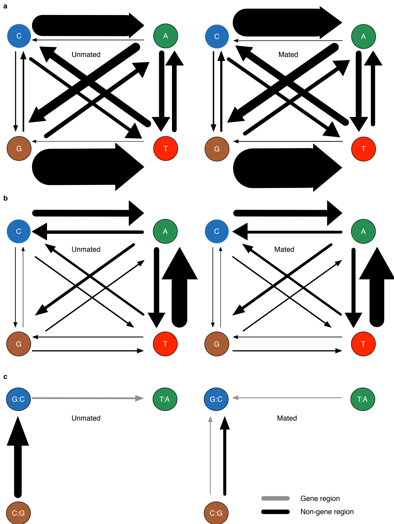
Supplemental Fig S7. Spectra of substitution disagreements and mismatches, and of substitutions. (a-c) Duplex substitution disagreement (a), raw Q2 substitution mismatch (b), or substitution (c) spectra. Arrow thickness is proportional to the rate of corresponding substitution.
