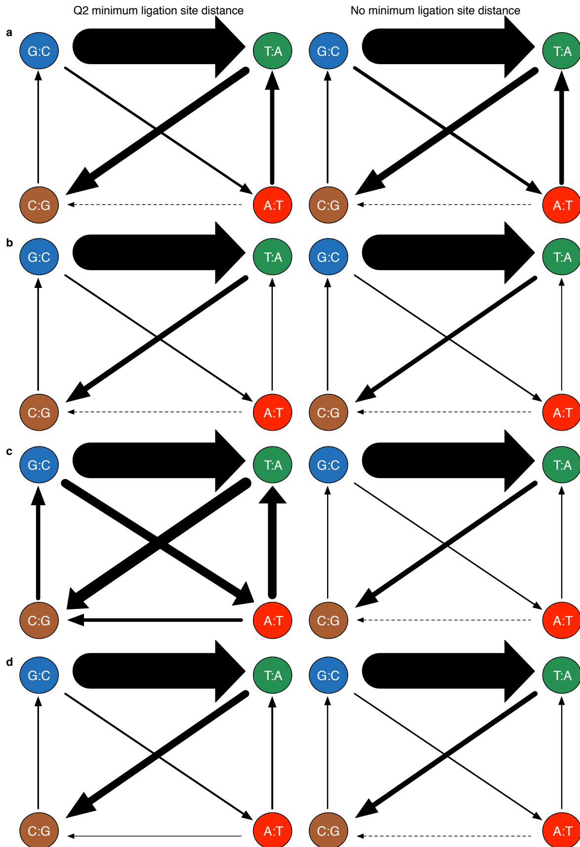
Supplemental Fig S17. Comparison of Mutinack duplex substitution disagreement spectra and VarScan 2, MuTect 1, or MuTect 2 mutation spectra.
