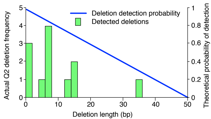
Supplemental Fig S11. Distribution of deletion lengths. Overlay shows detection probability of a deletion as a function of its length, assuming 150 bp reads.
