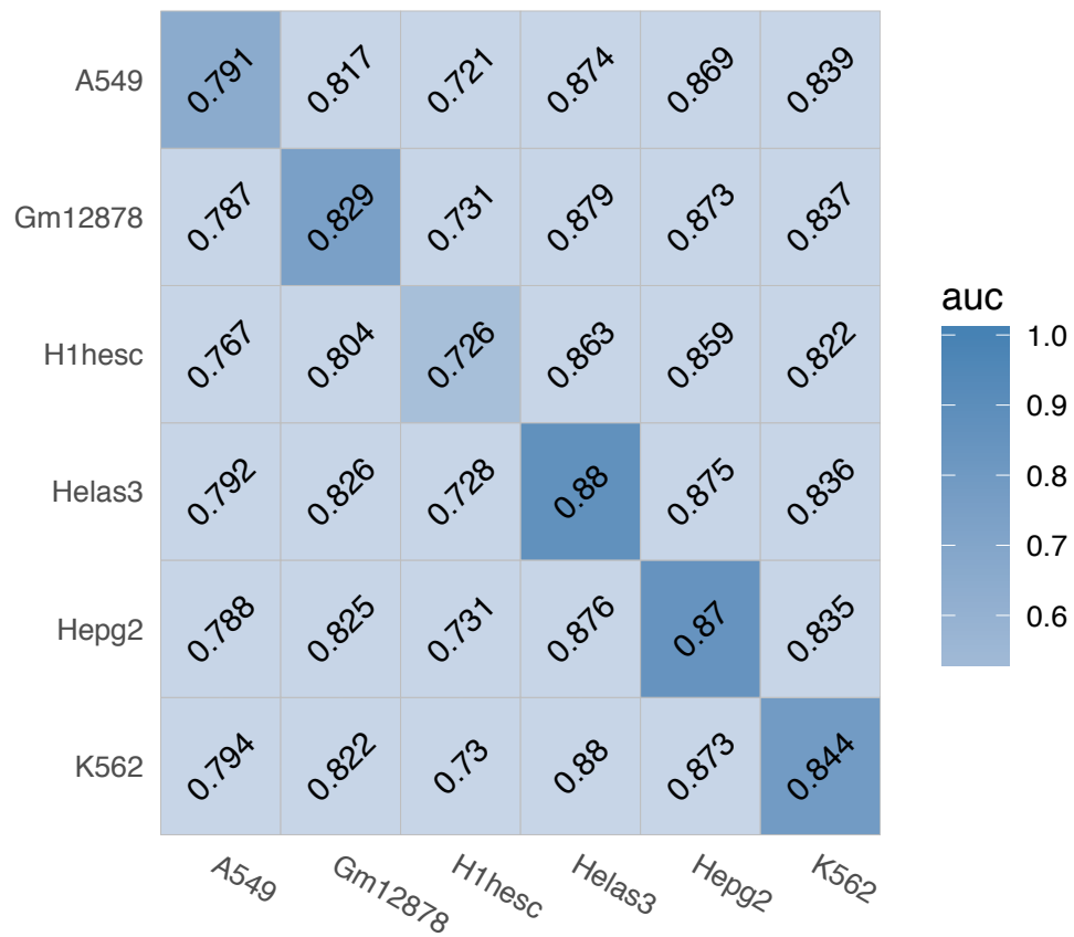
GABPA (Non-interaction)
