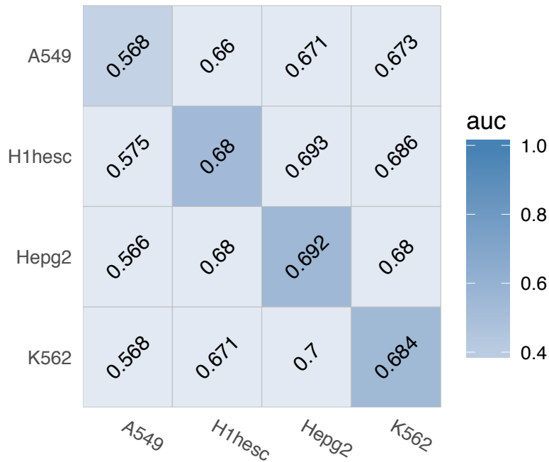
ATF3 (Non-interaction)
