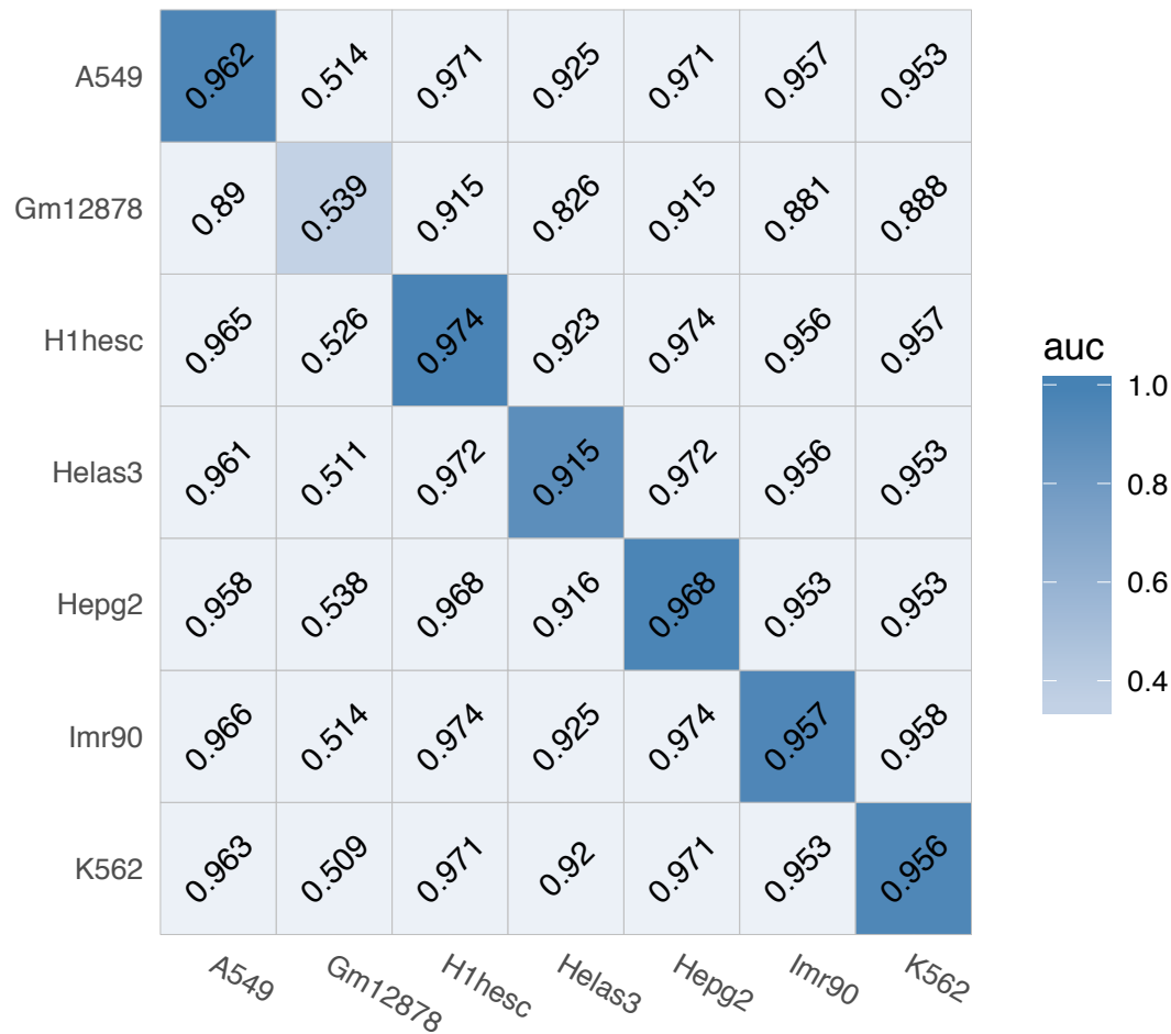
CEBPB (Non-interaction)
