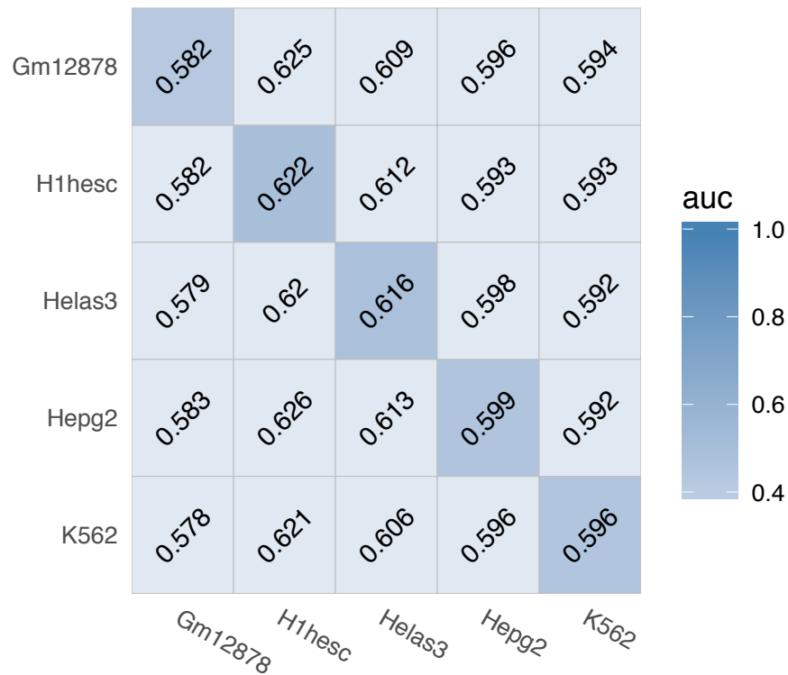
MXI1 (Non-interaction)
