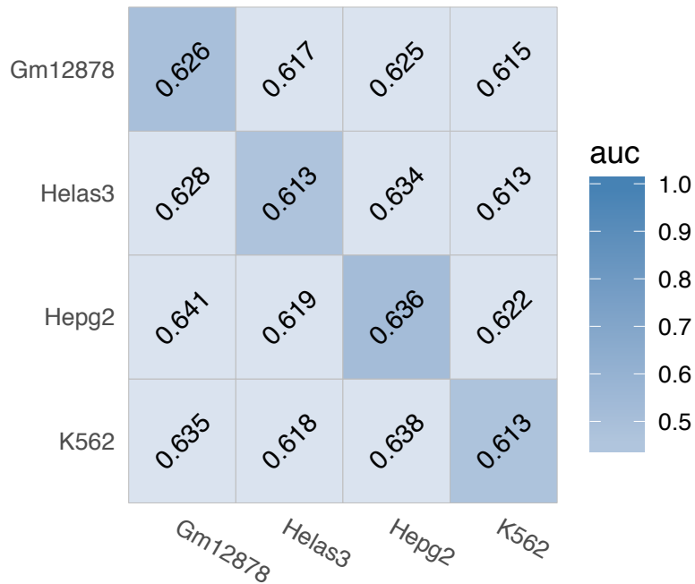
MAZ (Non-interaction)
