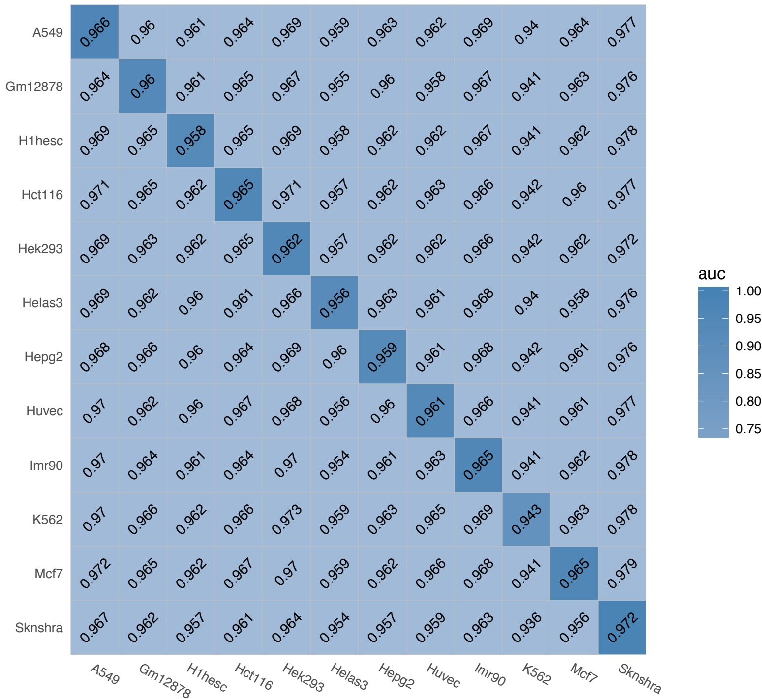
CTCF (Non-interaction)
