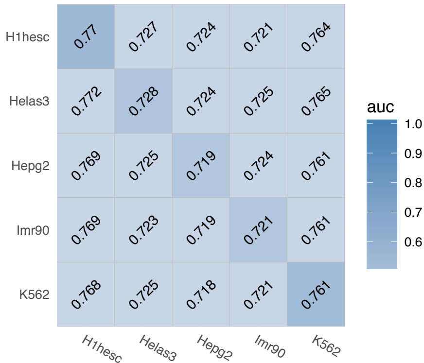
MAFK (Non-interaction)
