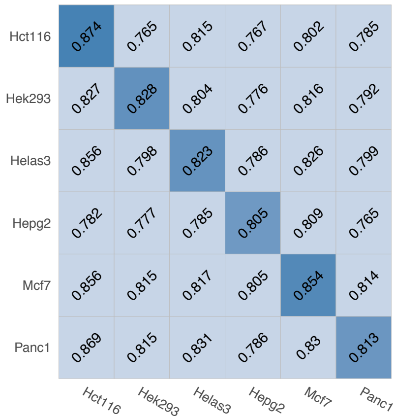
TCF7L2 (Interaction)
