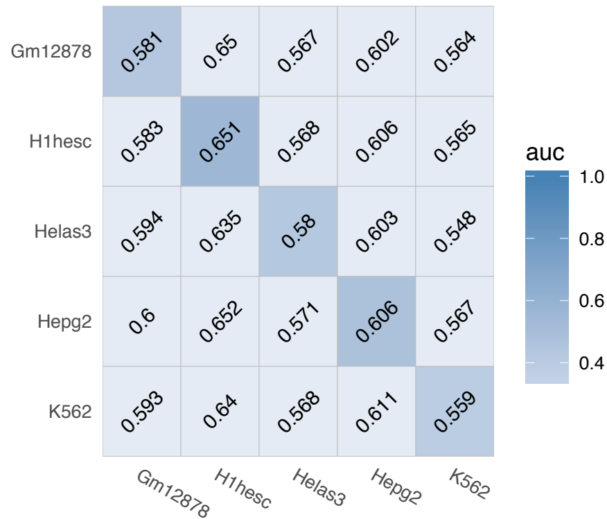
RFX5 (Non-interaction)
