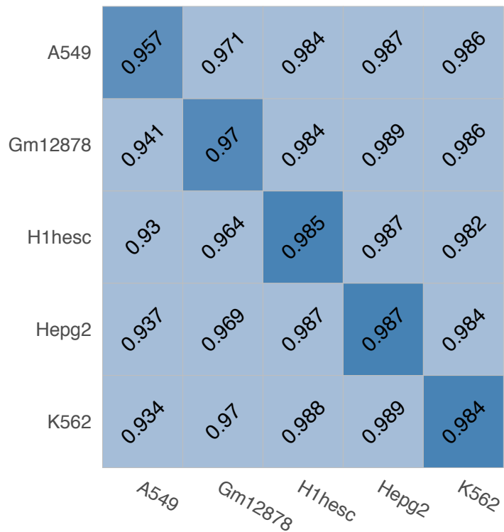
USF1 (Interaction)
