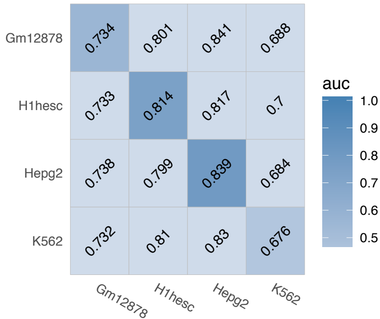
SRF (Non-interaction)
