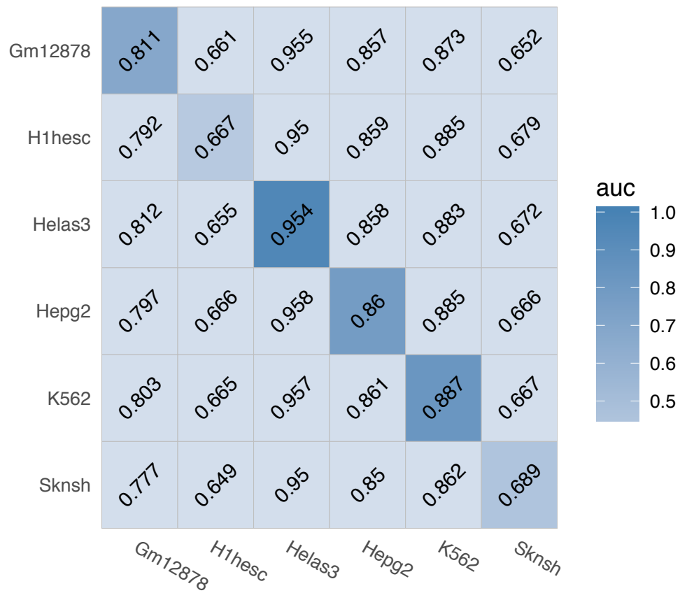
JUND (Non-interaction)
