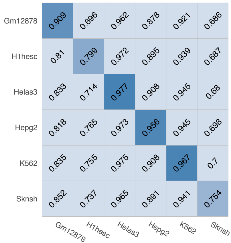
JUND (Interaction)
