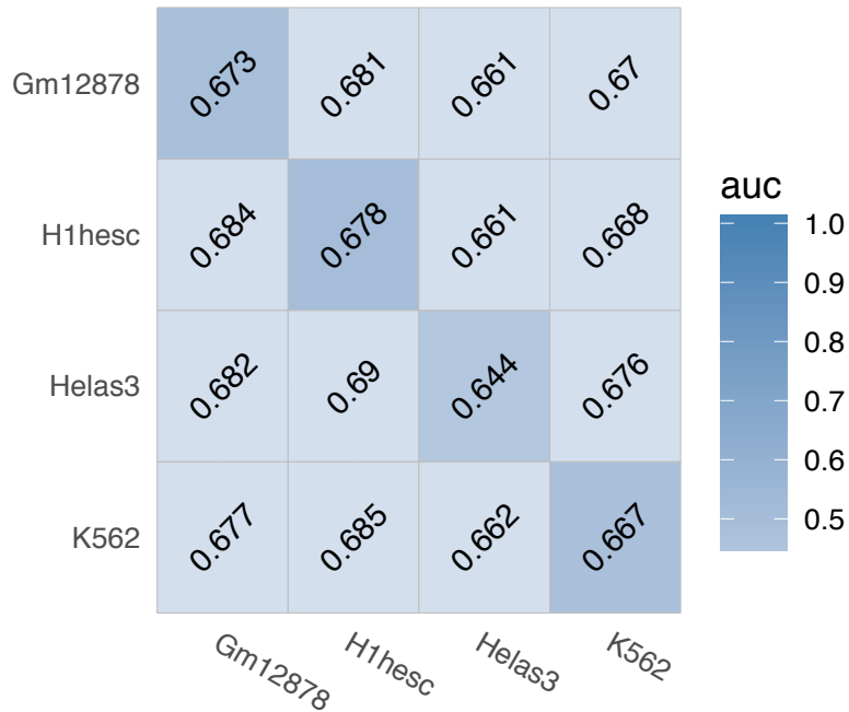
ZNF143 (Non-interaction)
