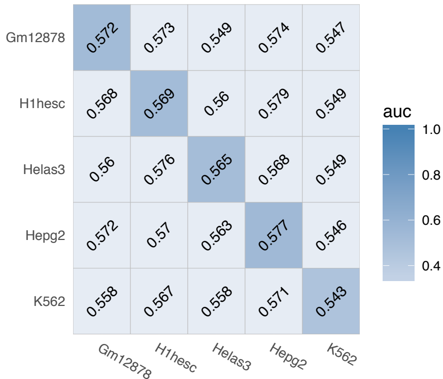
TBP (Non-interaction)
