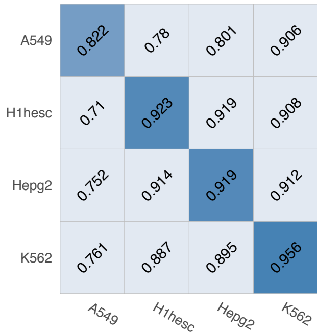
ATF3 (Interaction)
