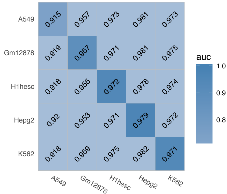
USF1 (Non-interaction)
