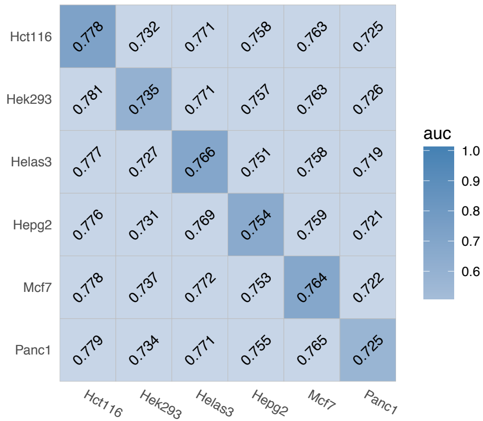
TCF7L2 (Non-interaction)
