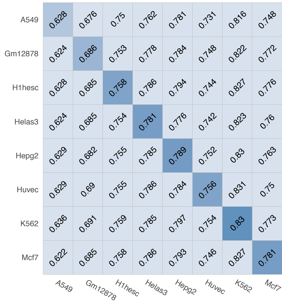
MYC (Non-interaction)
