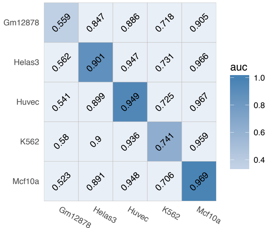
FOS (Non-interaction)
