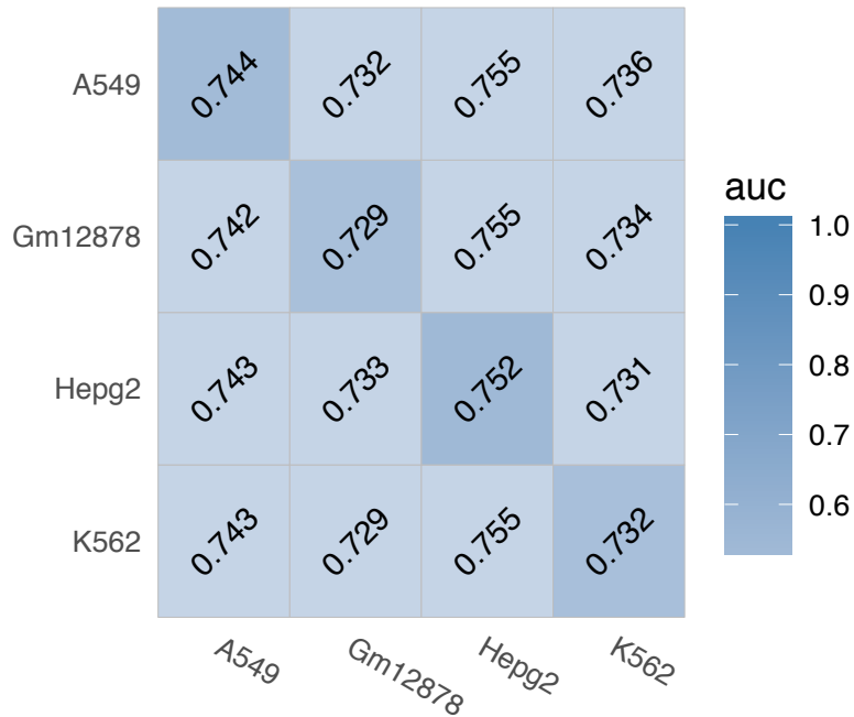
BHLHE40 (Non-interaction)
