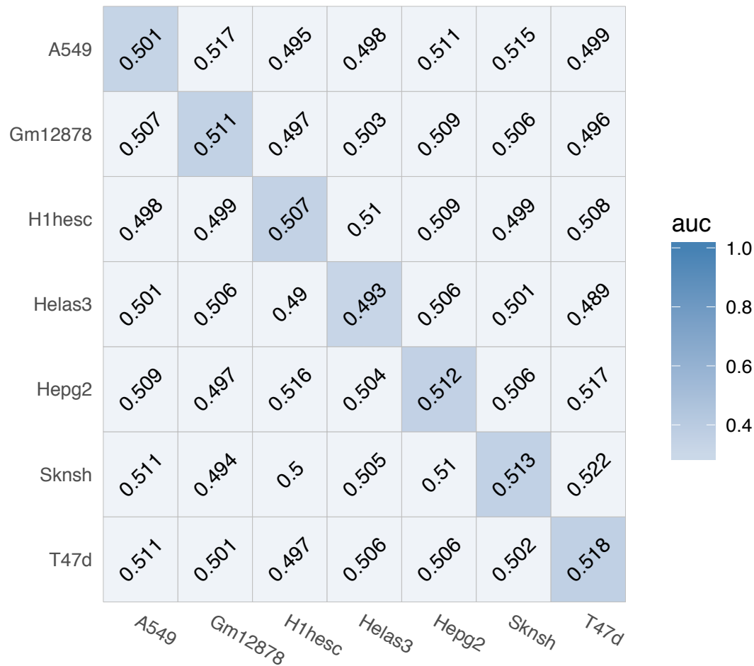
EP300 (Non-interaction)
