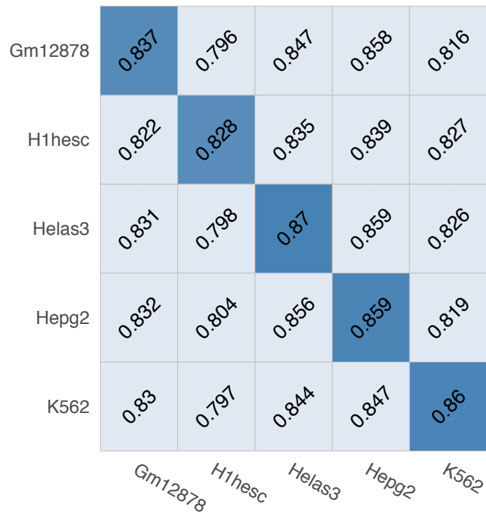
MXI1 (Interaction)
