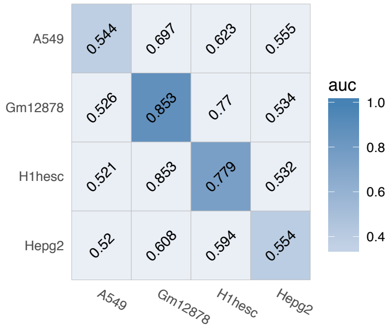
TCF12 (Non-interaction)
