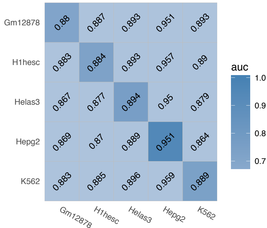
NRF1 (Non-interaction)
