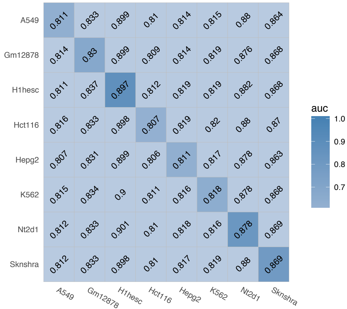
YY1 (Non-interaction)
