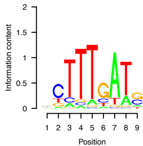
TCF7L2-M01705
