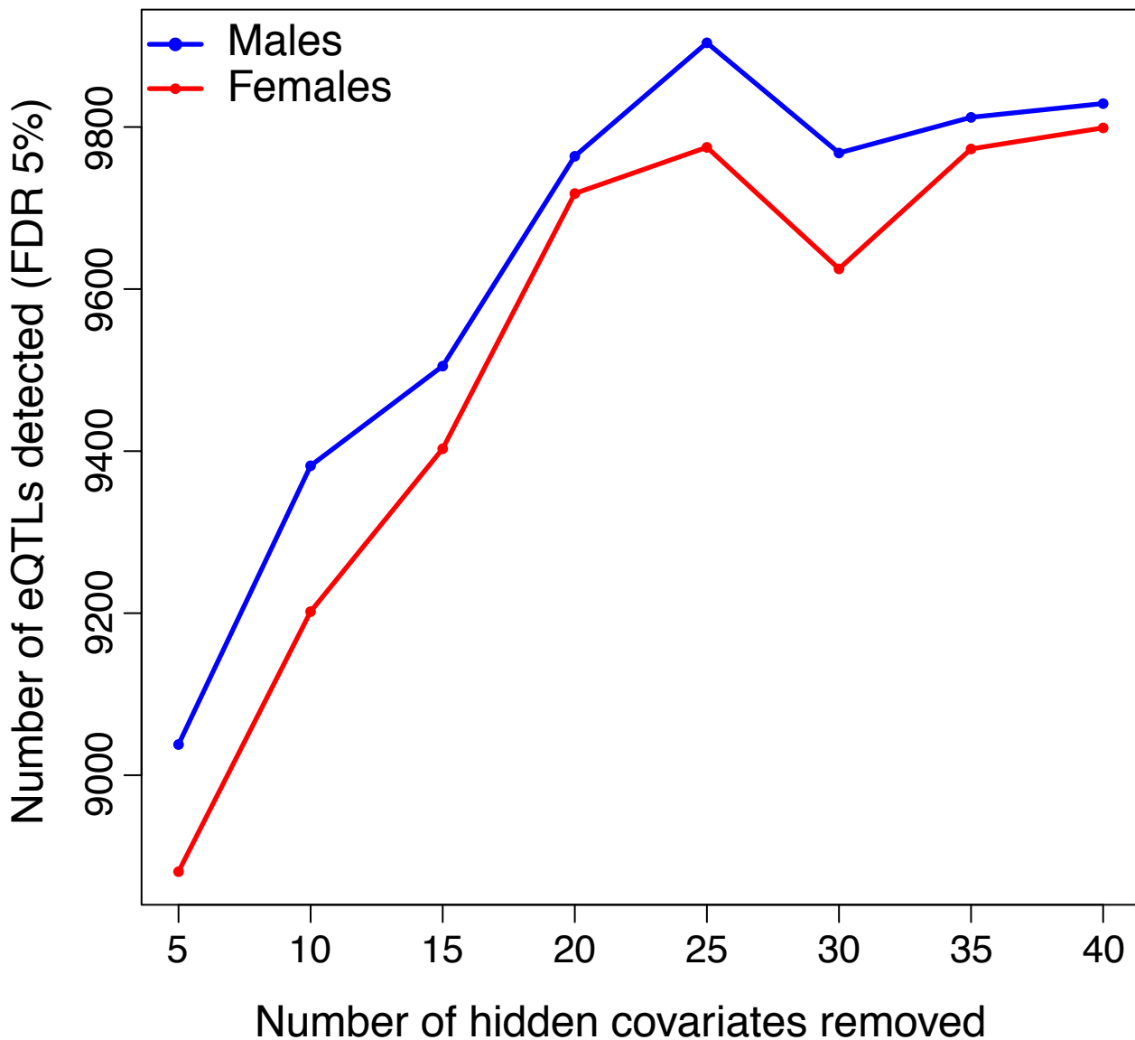
Figure S13. Removal of hidden covariates from expression data.
