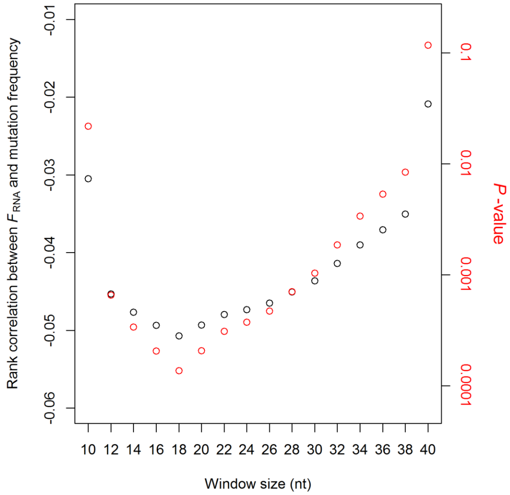
Figure S7. Spearman's rank correlation (black circles) and associated P -value (red circles) between the nascent RNA folding strength ( F_{\text{RNA}} ) of a gene and the mutation rate of the gene in yeast genomic analysis is robust to the window size (between 10 and 40 nucleotides) in F_{\text{RNA}} prediction.
