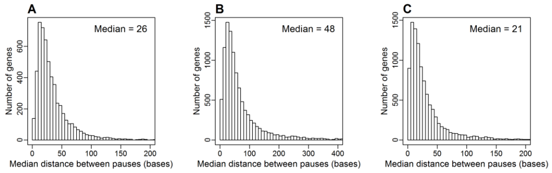
Figure S6. Frequency distribution of the median distance between RNA polymerase II pauses in a gene in (A) yeast ( n = 5,483 genes), (B) human introns ( n = 10,635 genes), and (C) human exons ( n = 10,234 genes).
