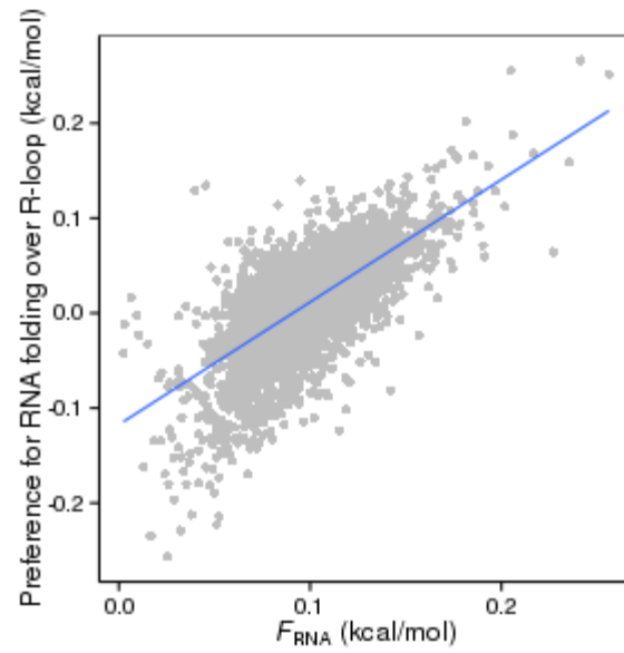
Figure S1. Preference of nascent RNA folding over R-loop formation increases as the nascent RNA folding ( F_{\text{RNA}} ) becomes stronger (Spearman's rank correlation = 0.647, P < 10^{-99} ). Each gray dot represents one of the 6433 intronless yeast genes examined. Blue line shows the fitted line.
