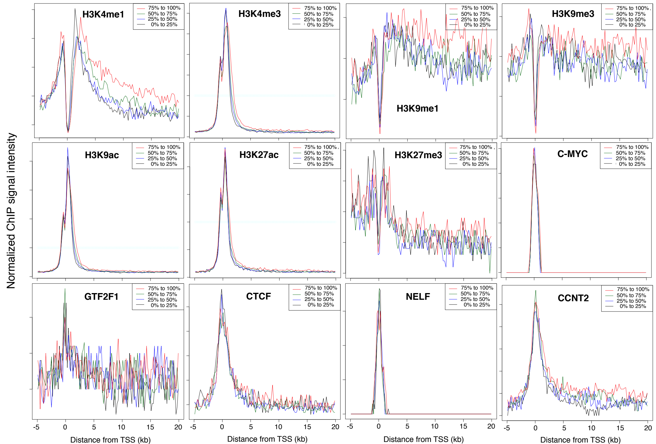
Supplemental Figure 2. Comparisons between elongation rate and histone modification or transcription factor binding. Genes expressed in K562 cells were ranked according to elongation rate and placed into four equal-sized groups (from fastest to slowest: red, green, blue, black). ChIP-Seq signal was obtained from ENCODE and median binned values for each group were plotted as indicated.
