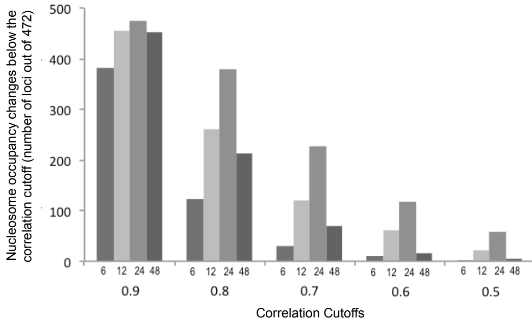
Supp. Fig. 4. Nucleosome distribution changes in loci 6, 12, 24, and 48 hours post reactivation of Kaposi's sarcoma-associated herpesvirus (KSHV) at multiple cutoffs including 0.5, 0.6, 0.7, 0.8, and 0.9. The most discriminative correlation cutoff amongst the timepoints was r=0.7 .
