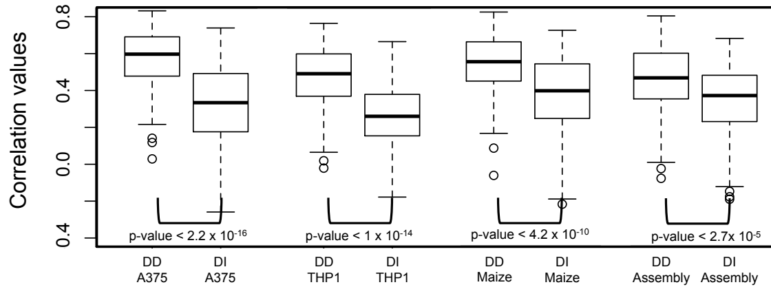
Supp. Fig. 14. Boxplot of correlations between the genes classified as DNA-directed and DNA-independent at 24 hours post KSHV reactivation with the four models: SVM trained model on nucleosome distribution from A375 cells, SVM trained model on nucleosome distribution from THP1 cells, SVM trained model on nucleosome distribution from Maize primary tissue and SVM trained model on salt dialysis assemblies. The genes classified as DNA-directed show statistically significant increase in correlation between the 24 hours and every model tested.
