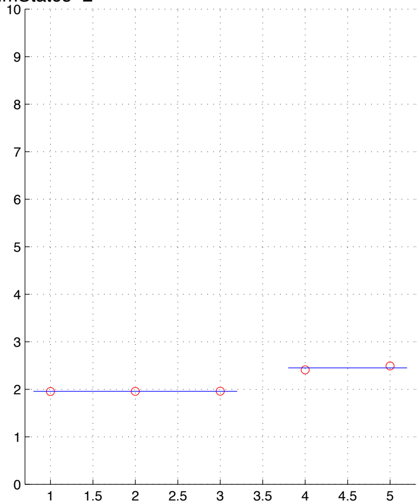
LUSC-8-T.chainID.1 numStates=2
