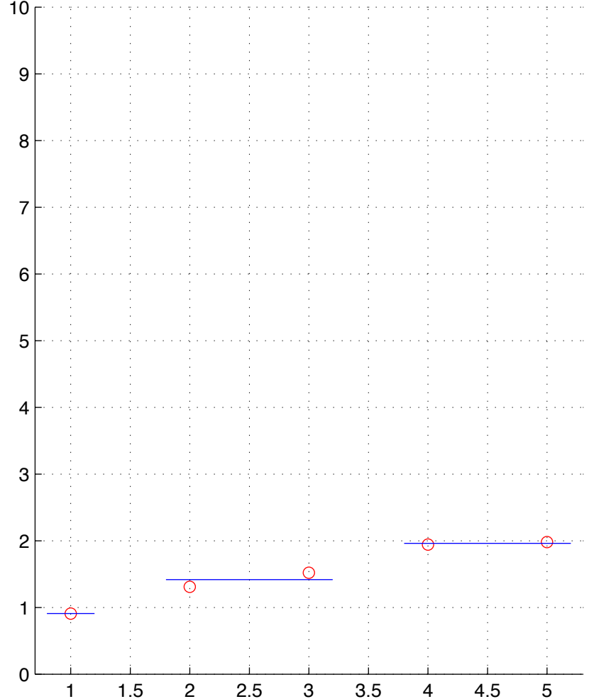
READ-1-T.chainID.2 numStates=3
