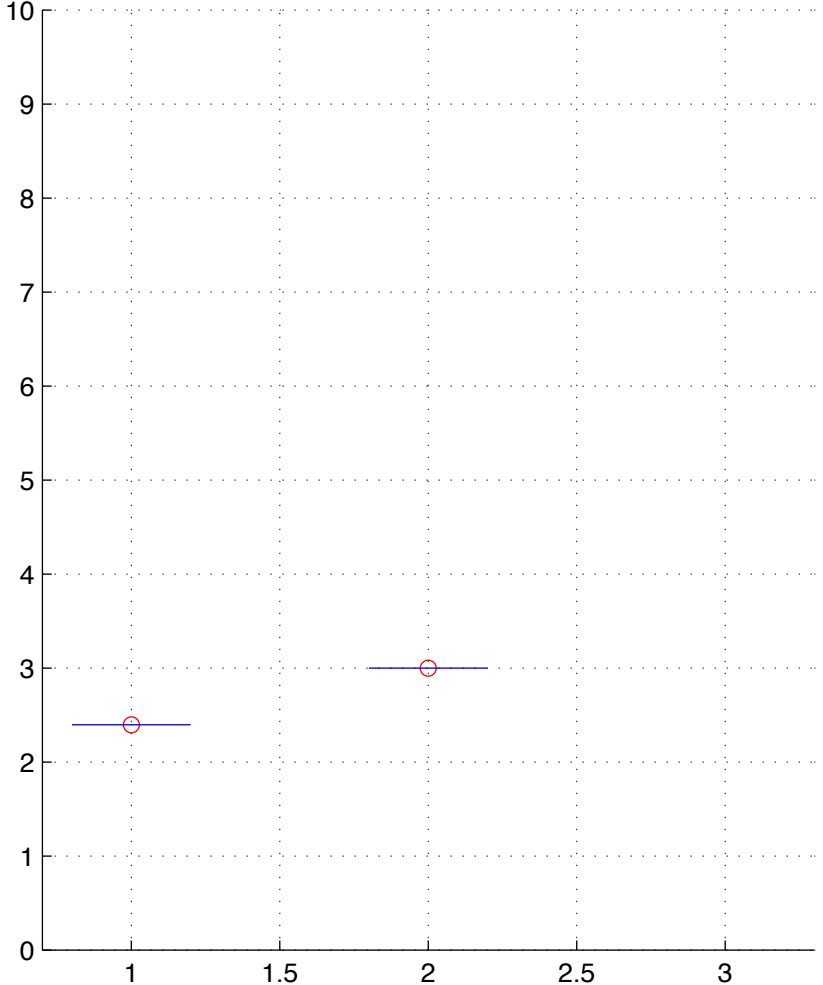
BRCA-4-T.chainID.5 numStates=2
