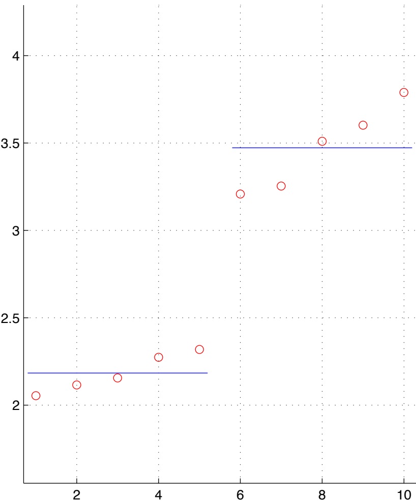
LUSC-6-T.chainID.2 numStates=2
