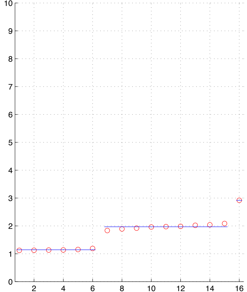
GBM-17-T.chainID.1 numStates=3
