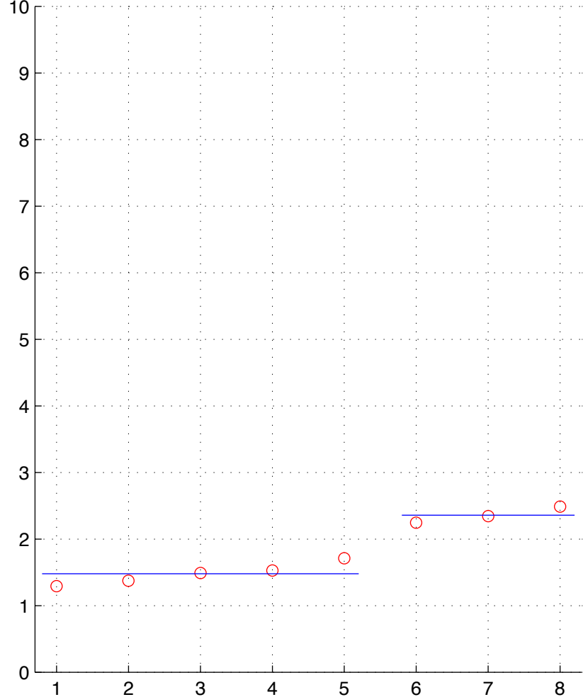
LUSC-5-T.chainID.4 numStates=2
