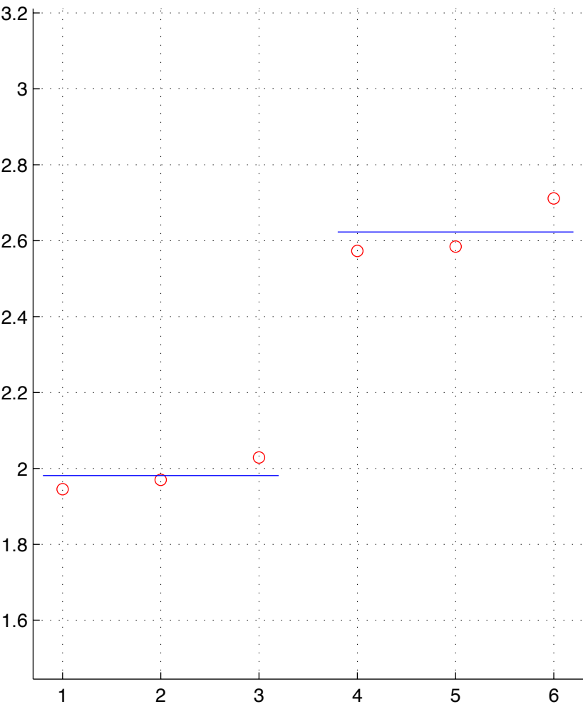
GBM-10-T.chainID.4 numStates=2
