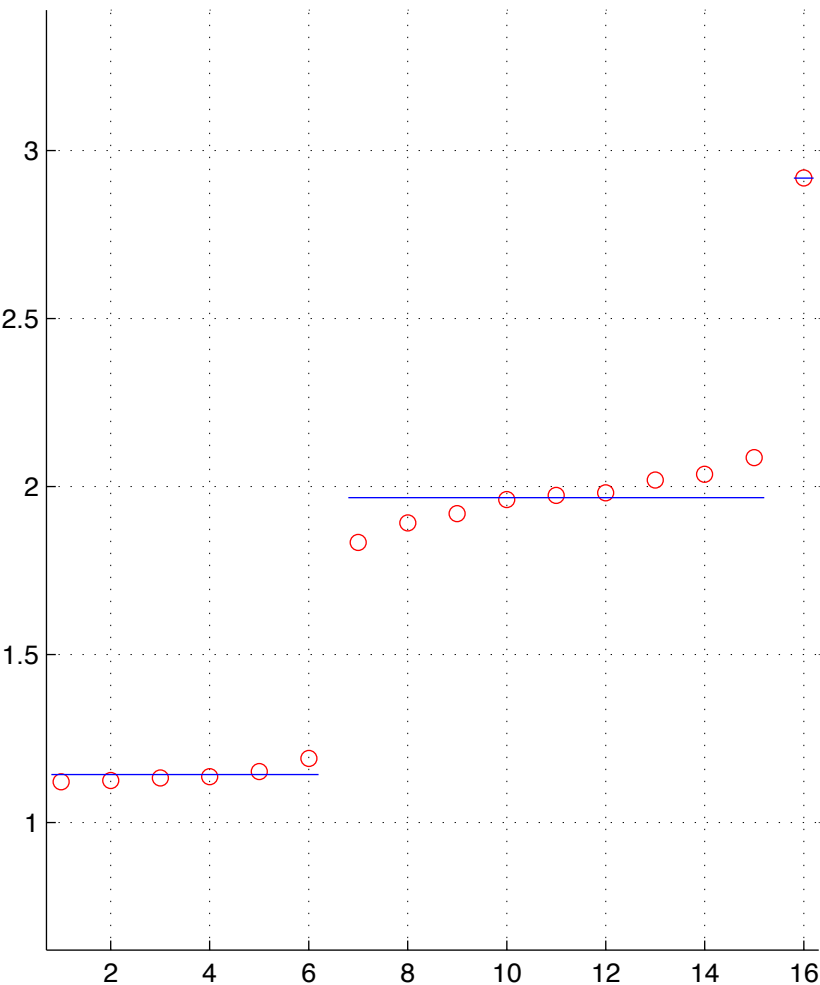
GBM-17-T.chainID.1 numStates=3
