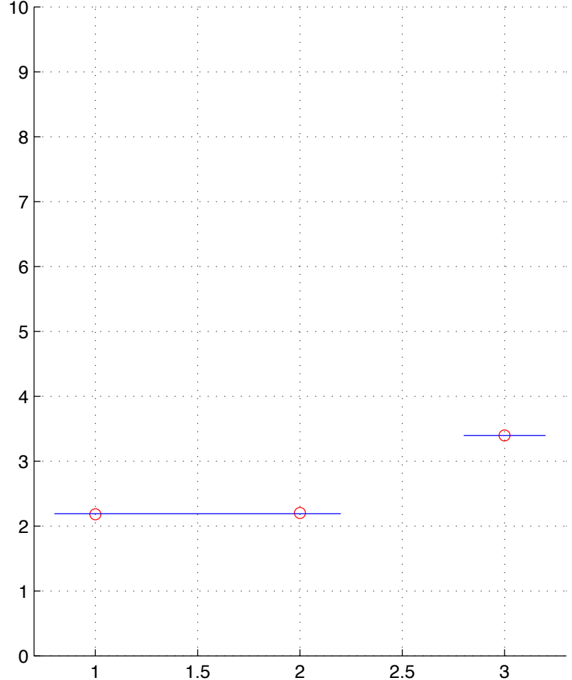
LUSC-13-T.chainID.11 numStates=2
