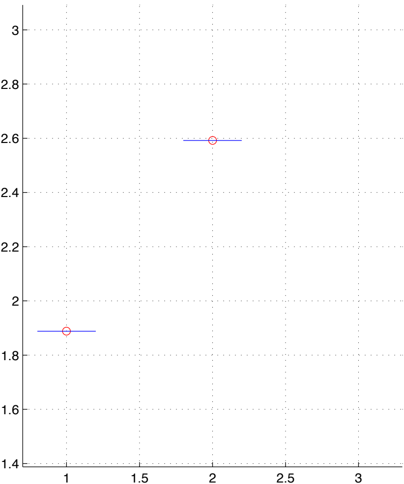
BRCA-5-T.chainID.1 numStates=2
