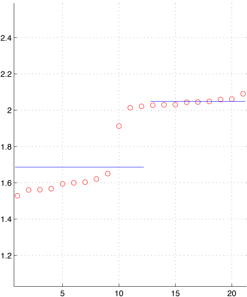
GBM-19-T.chainID.2 numStates=2
