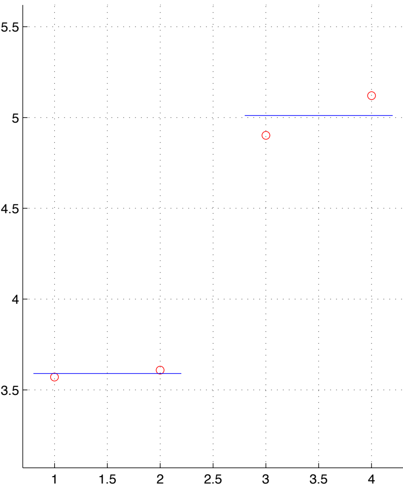
BRCA-12-T.chainID.2 numStates=2
