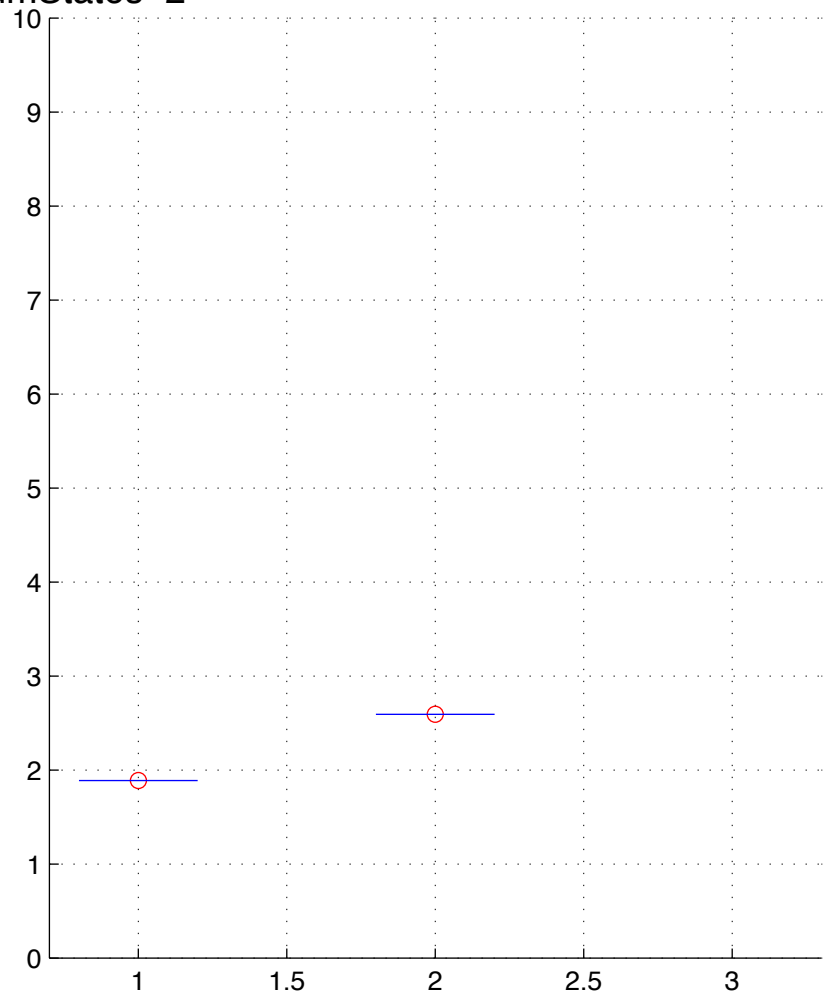
BRCA-5-T.chainID.1 numStates=2
