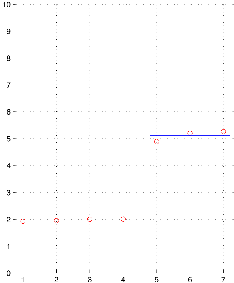
BRCA-12-T.chainID.1 numStates=2
