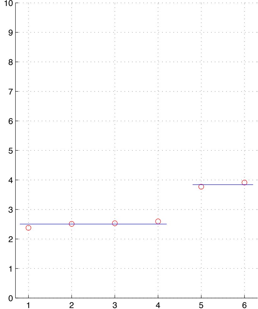
BRCA-1-T.chainID.2 numStates=2
