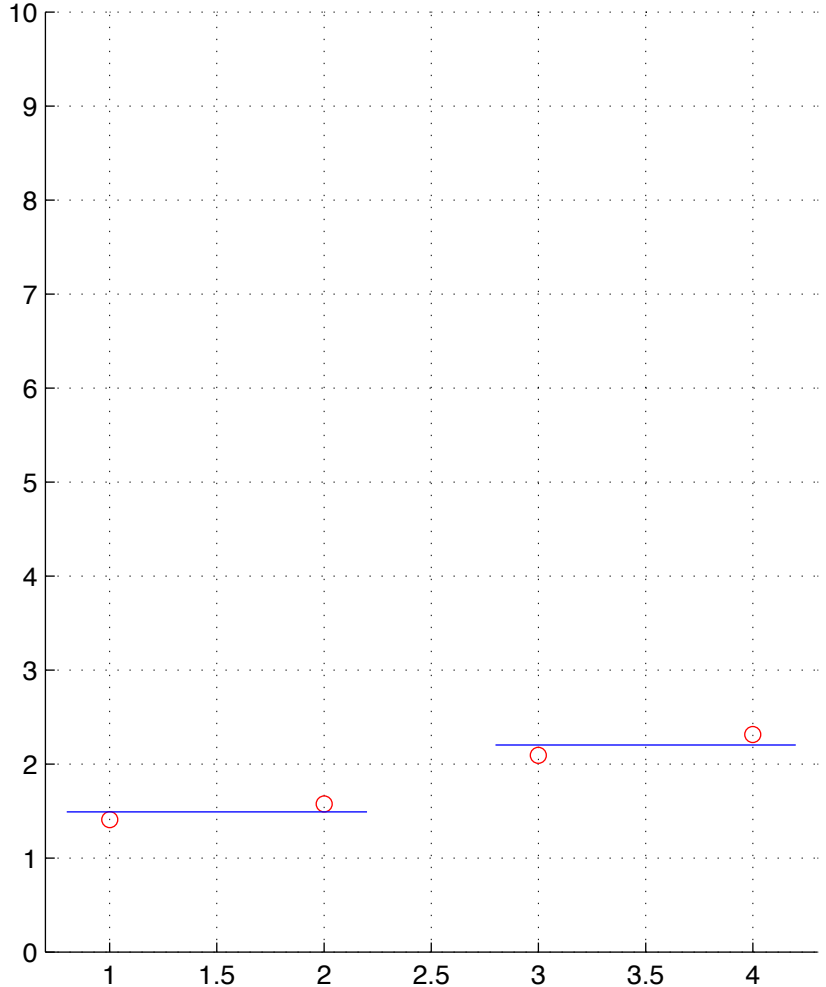
GBM-8-T.chainID.1 numStates=2
