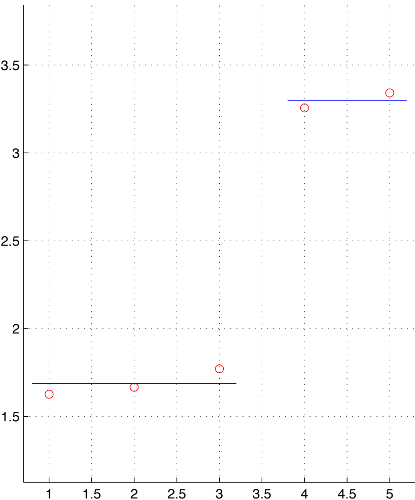
OV-5-T.chainID.5 numStates=2
