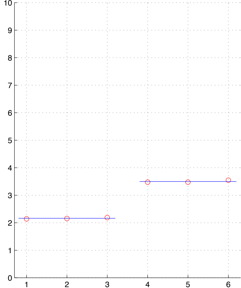
LUSC-11-T.chainID.3 numStates=2
