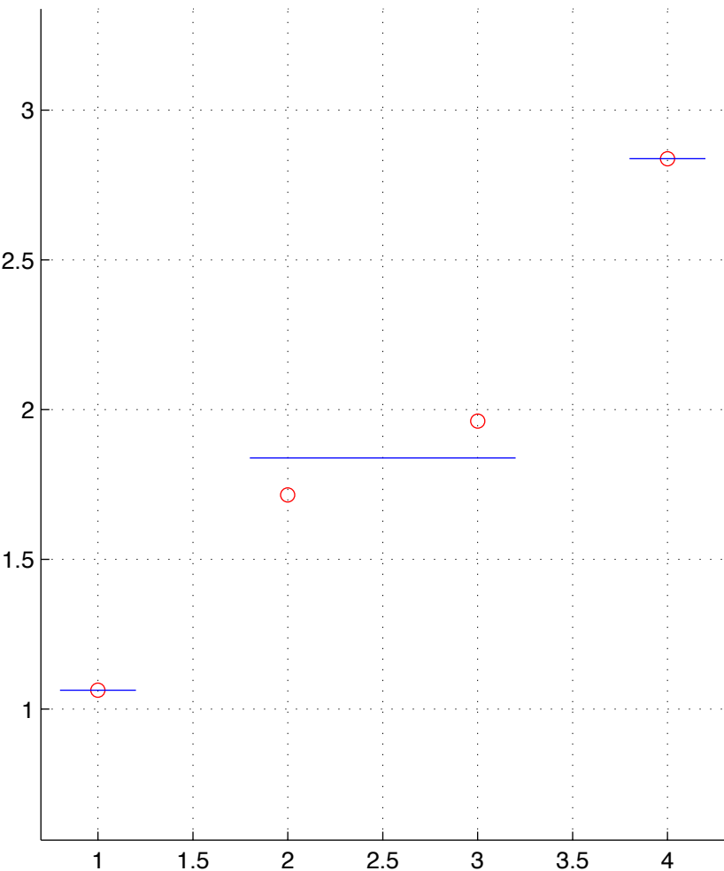
LUSC-13-T.chainID.5 numStates=3
