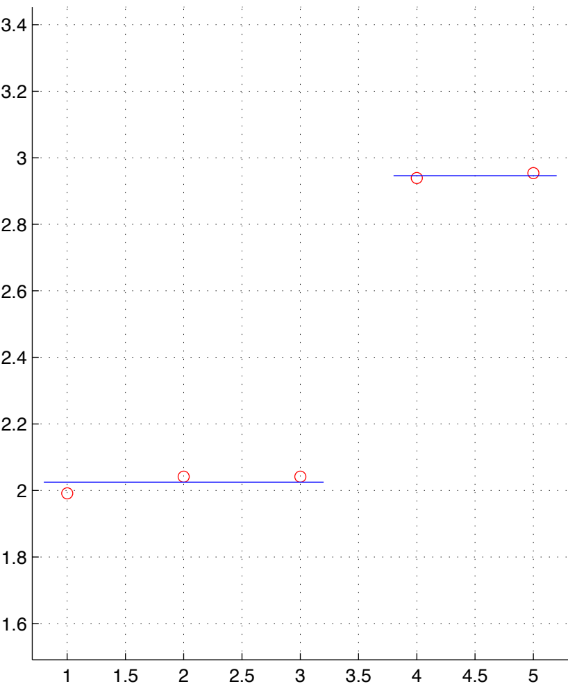
GBM-17-T.chainID.2 numStates=2
