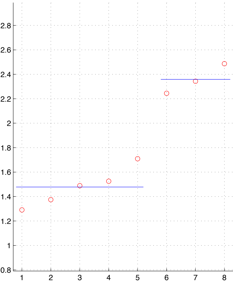
LUSC-5-T.chainID.4 numStates=2
