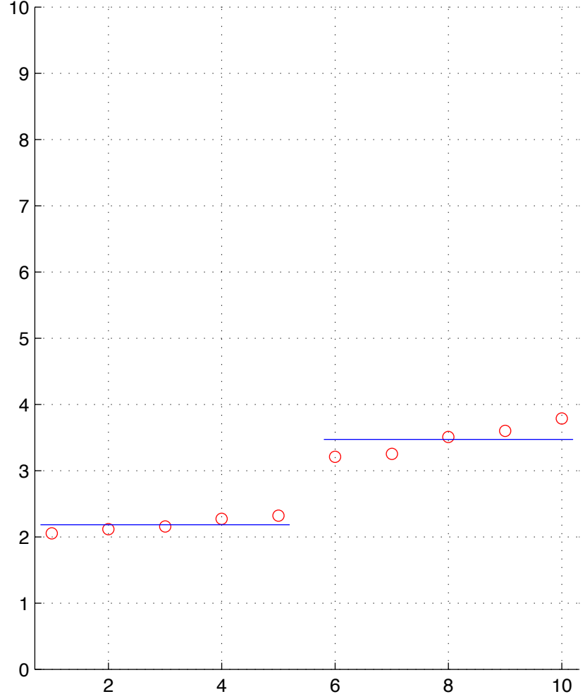
LUSC-6-T.chainID.2 numStates=2
