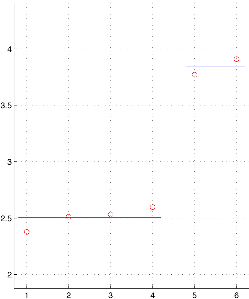
BRCA-1-T.chainID.2 numStates=2
