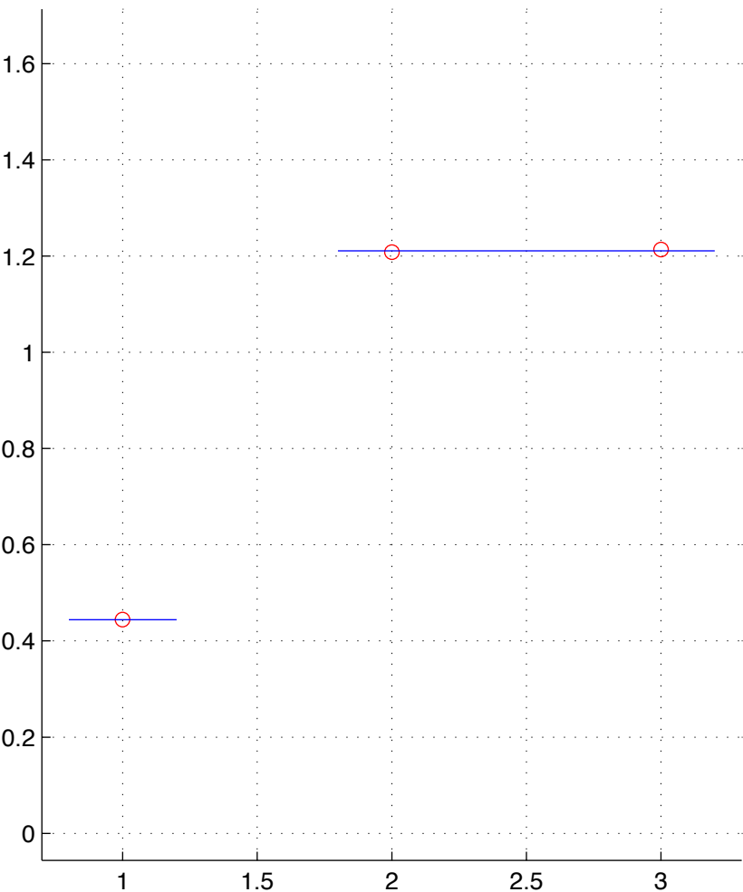
GBM-16-T.chainID.4 numStates=2
