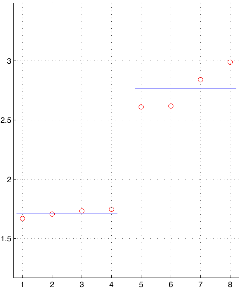
LUAD-6-T.chainID.1 numStates=2
