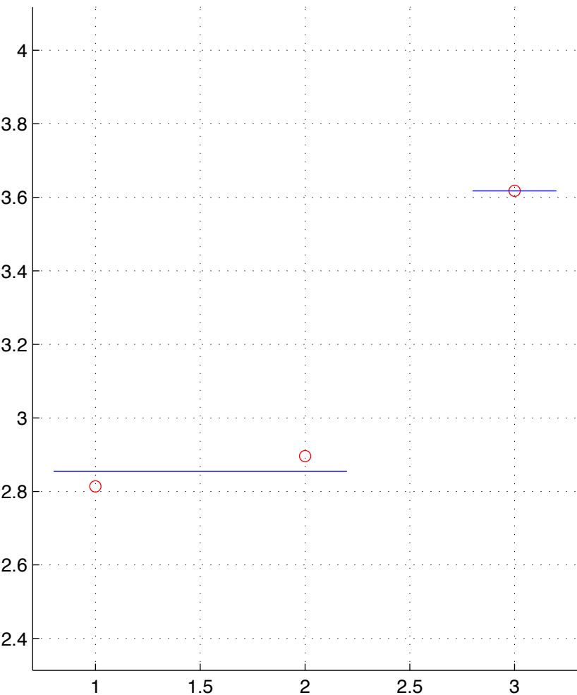
READ-2-T.chainID.1 numStates=2
