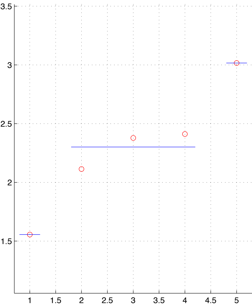
OV-6-T.chainID.1 numStates=3
