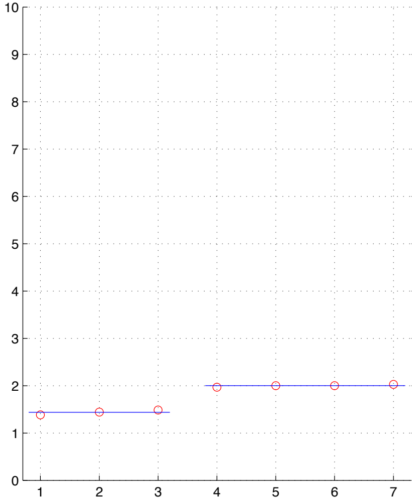
GBM-18-T.chainID.1 numStates=2
