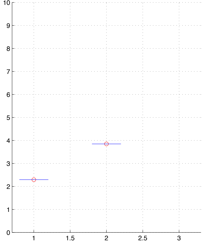
BRCA-3-T.chainID.1 numStates=2
