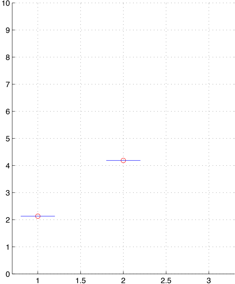
LUSC-5-T.chainID.2 numStates=2
