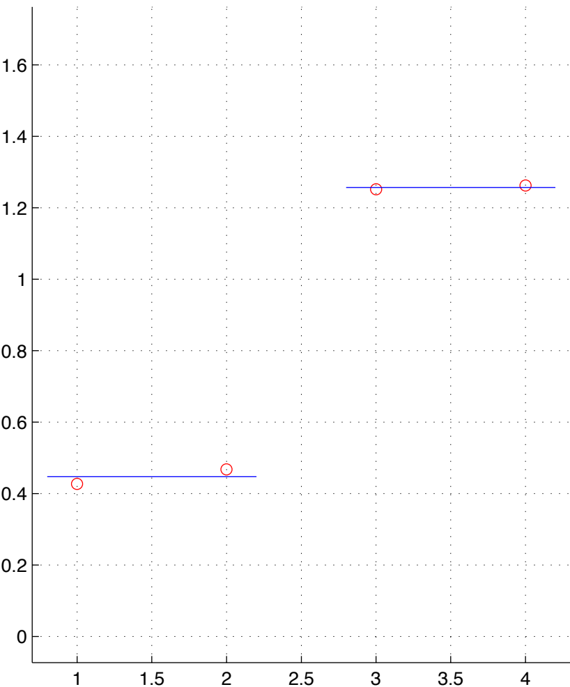
GBM-4-T.chainID.1 numStates=2
