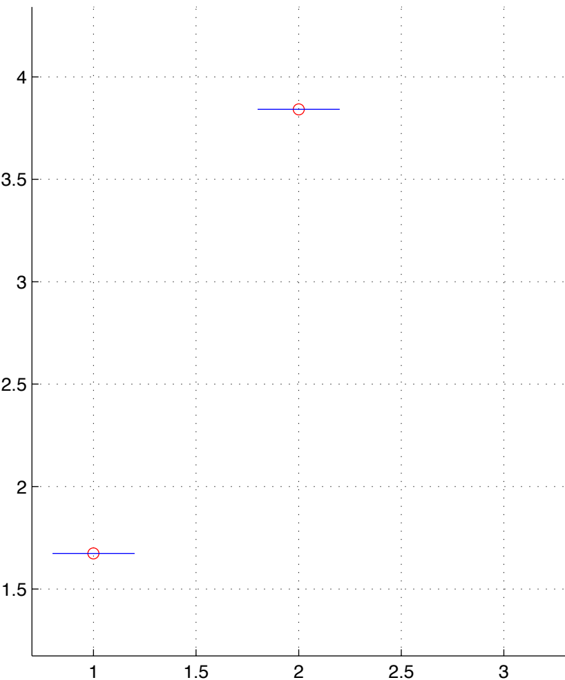
LUSC-11-T.chainID.2 numStates=2
