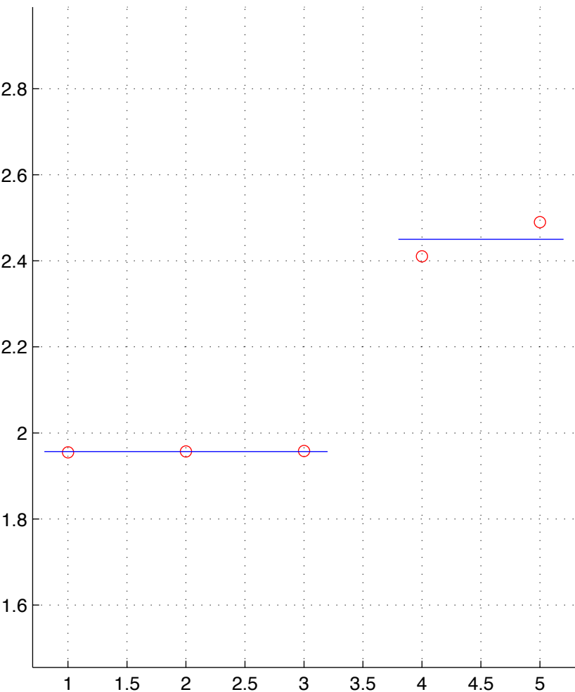
LUSC-8-T.chainID.1 numStates=2
