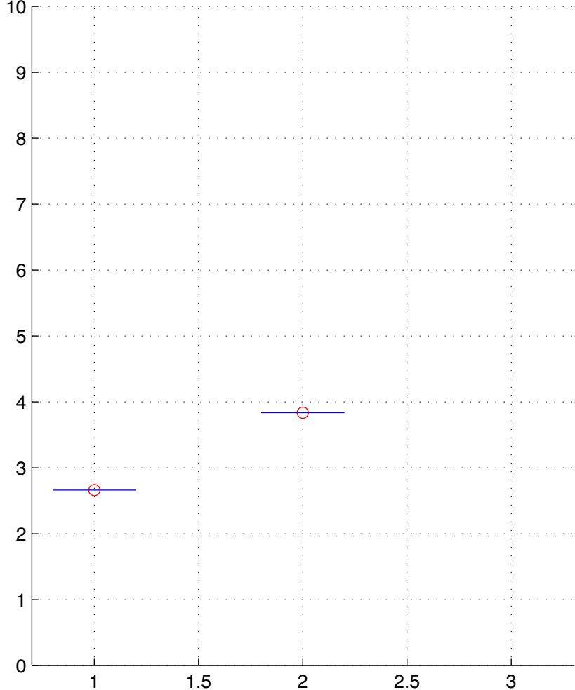
LUSC-13-T.chainID.8 numStates=2
