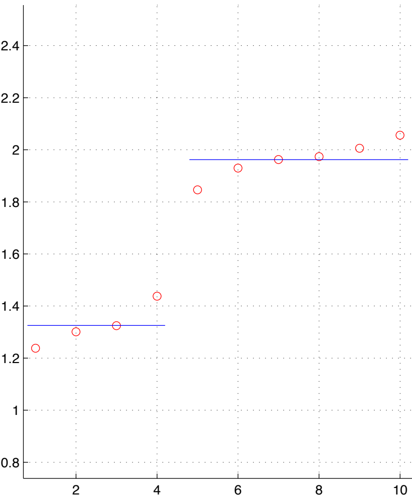
GBM-7-T.chainID.3 numStates=2
