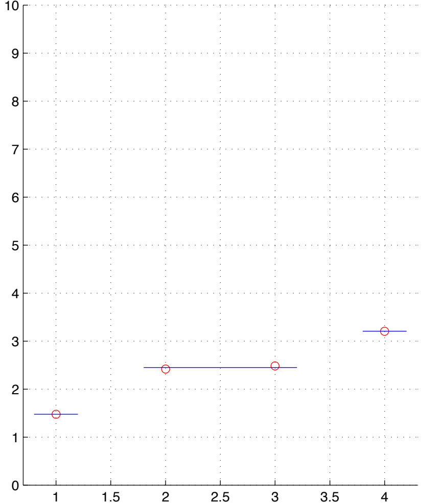
LUSC-11-T.chainID.4 numStates=3
