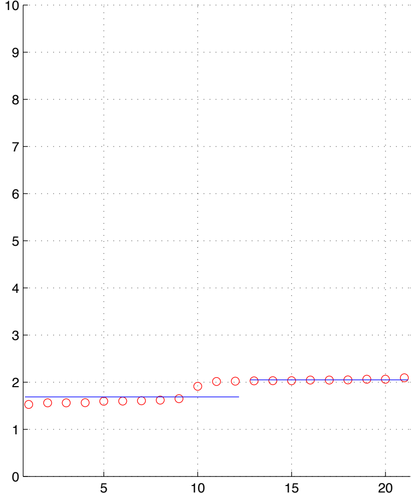
GBM-19-T.chainID.2 numStates=2
