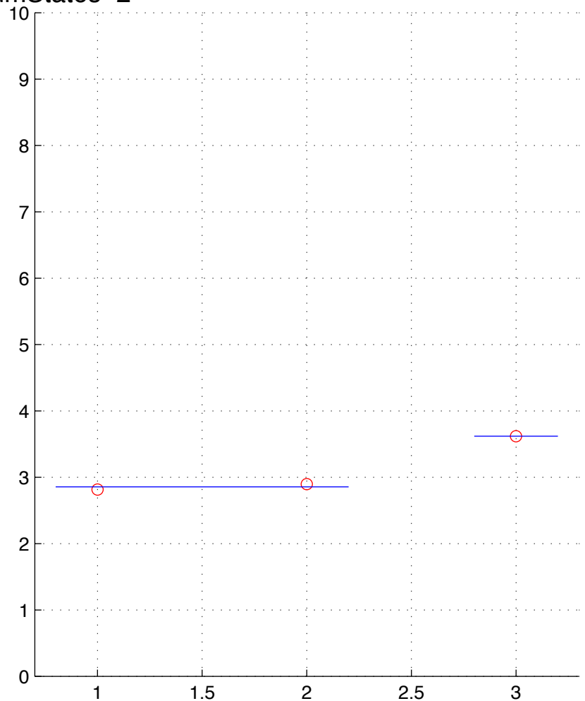
READ-2-T.chainID.1 numStates=2
