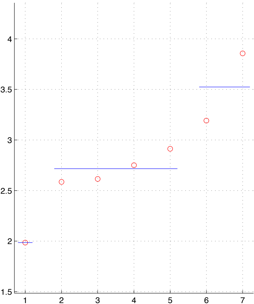
READ-1-T.chainID.1 numStates=3
