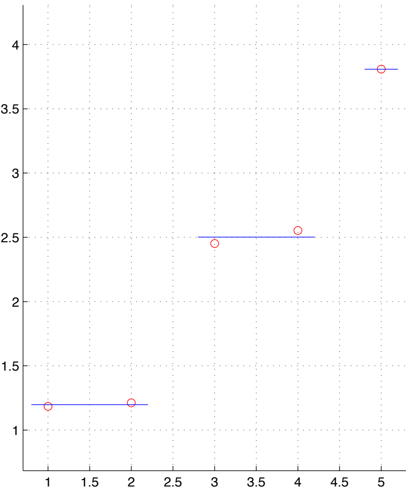
BRCA-4-T.chainID.8 numStates=3
