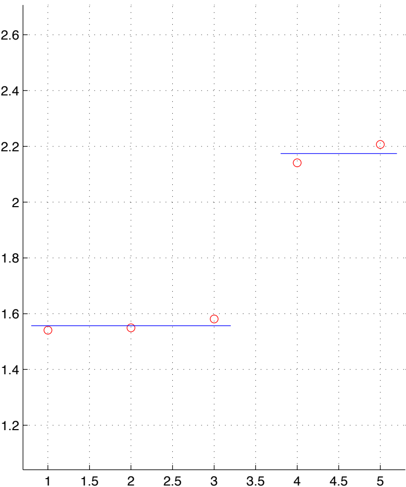
BRCA-6-T.chainID.1 numStates=2
