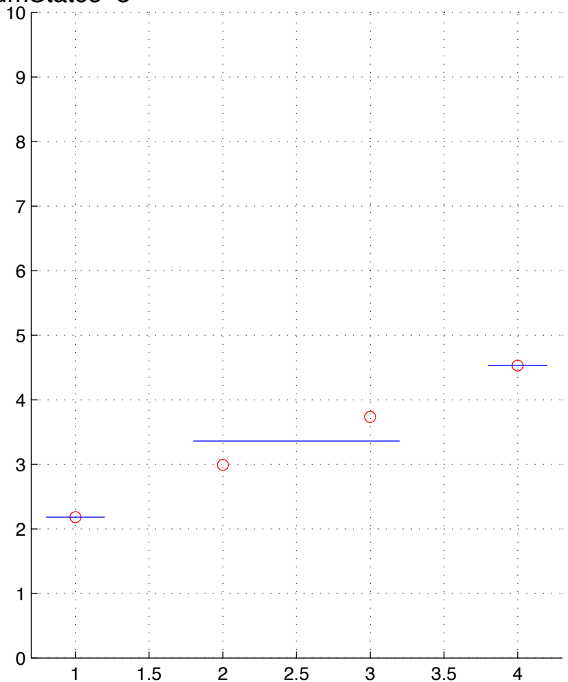
LUSC-13-T.chainID.6 numStates=3
