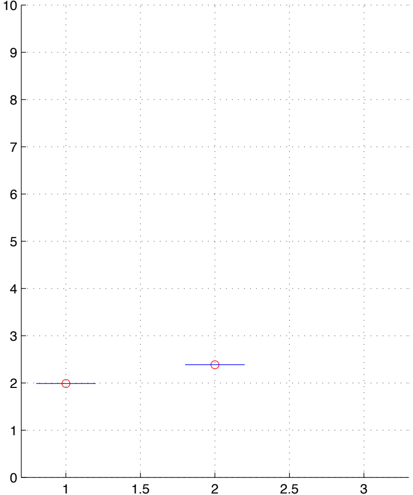
LUAD-6-T.chainID.2 numStates=2
