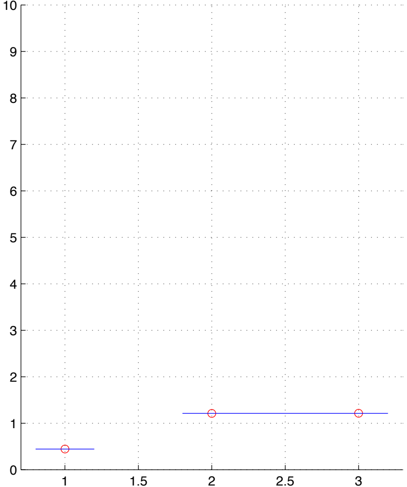
GBM-16-T.chainID.4 numStates=2
