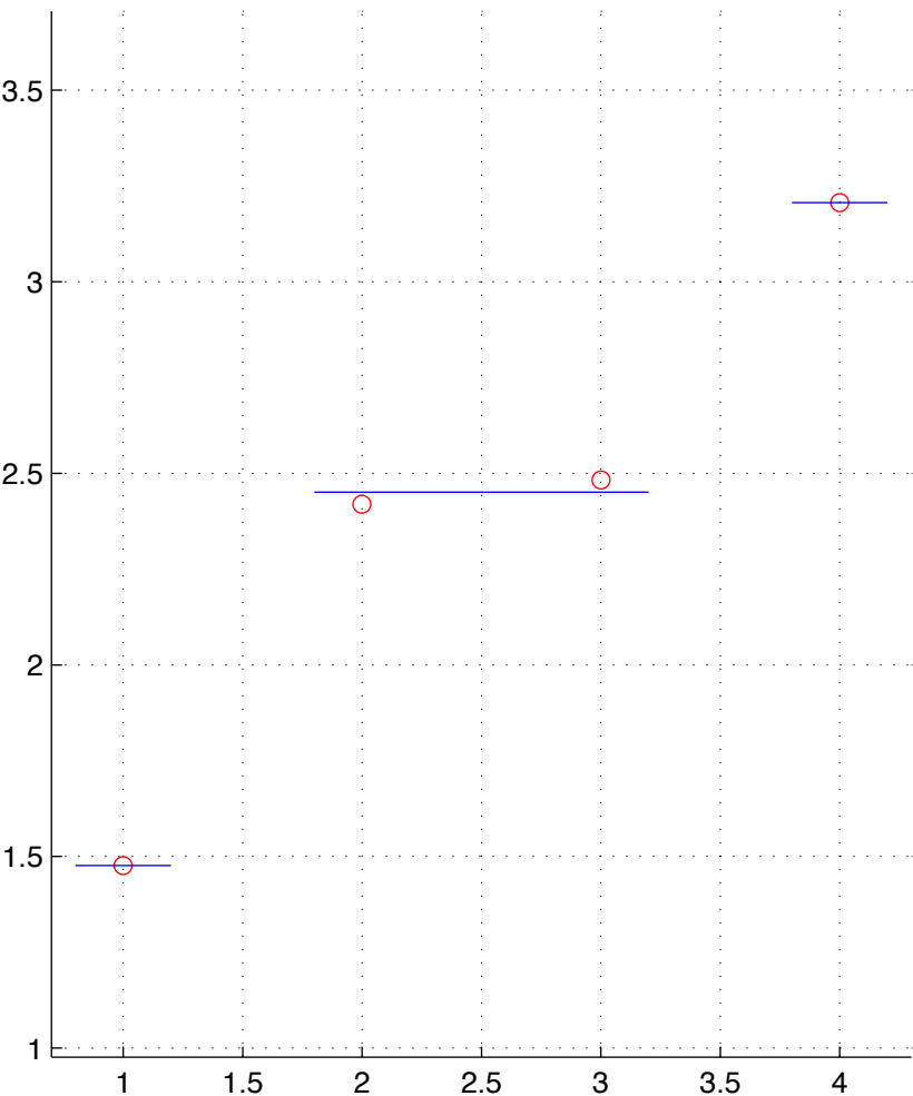
LUSC-11-T.chainID.4 numStates=3
