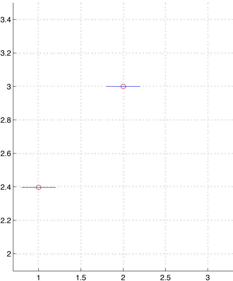
BRCA-4-T.chainID.5 numStates=2
