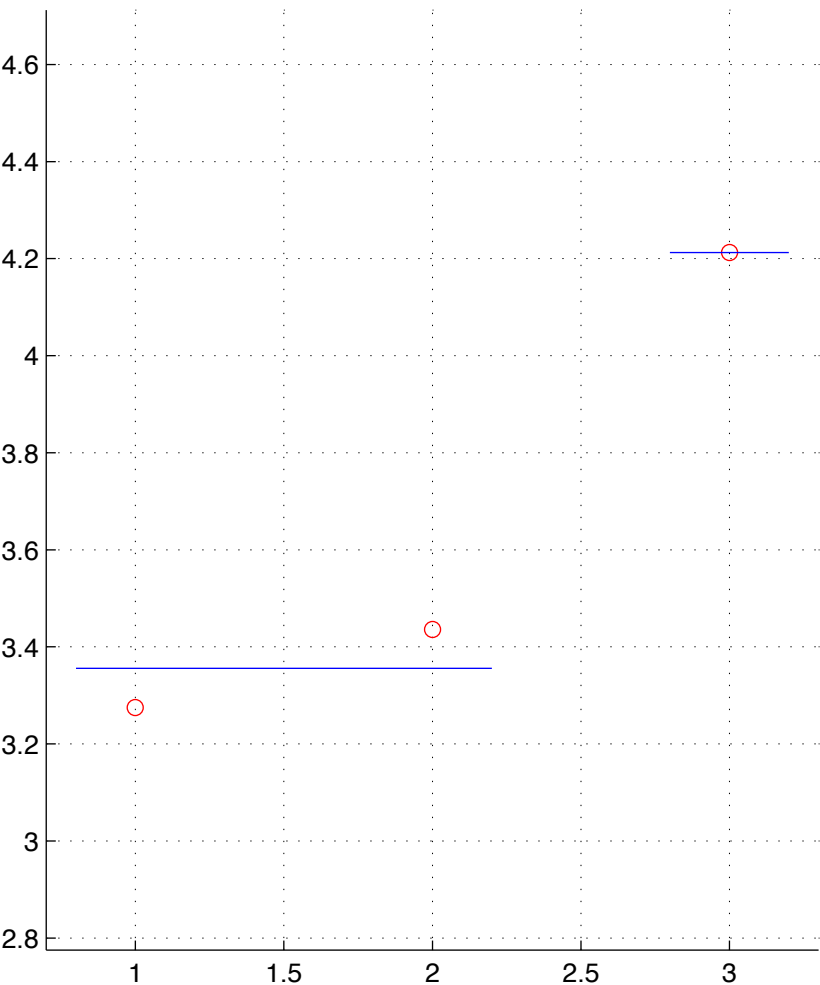
OV-5-T.chainID.6 numStates=2
