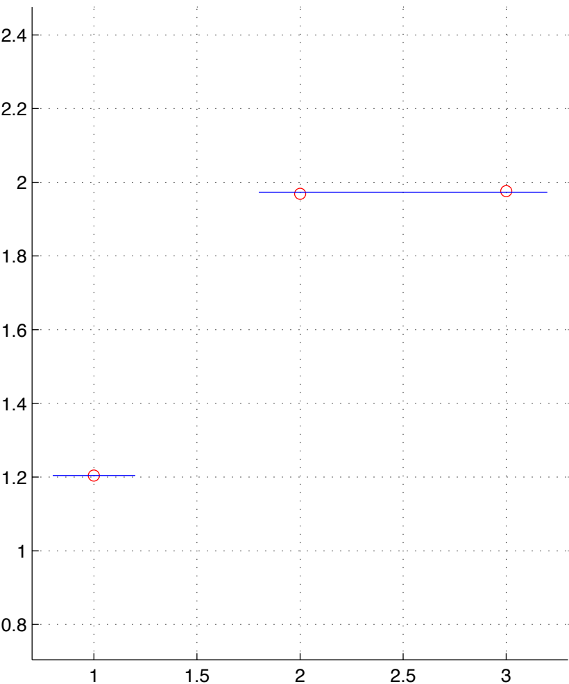
GBM-2-T.chainID.1 numStates=2
