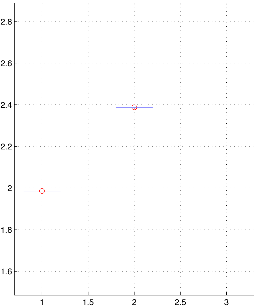
LUAD-6-T.chainID.2 numStates=2
