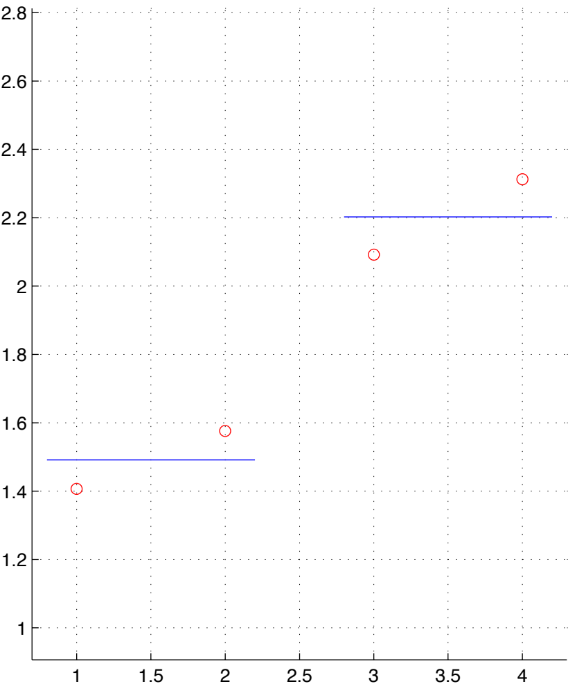
GBM-8-T.chainID.1 numStates=2
