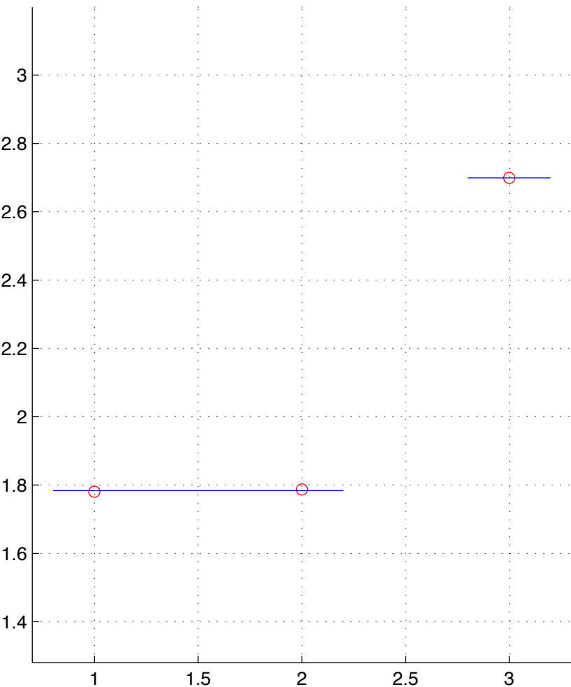
OV-5-T.chainID.3 numStates=2
