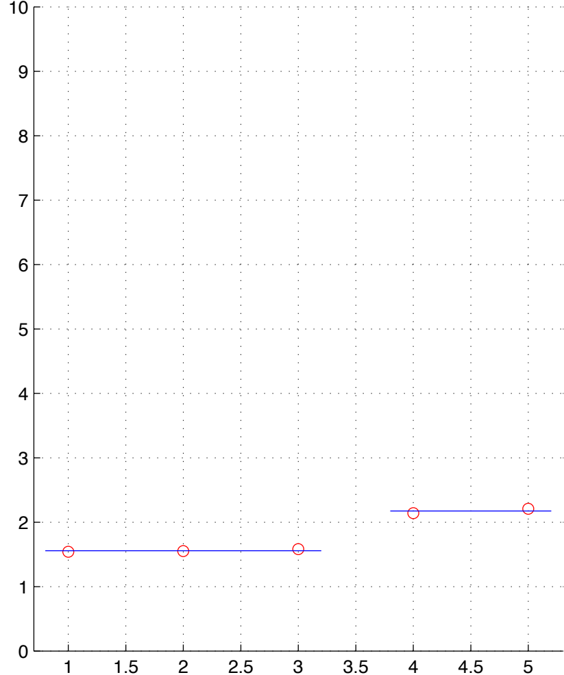
BRCA-6-T.chainID.1 numStates=2
