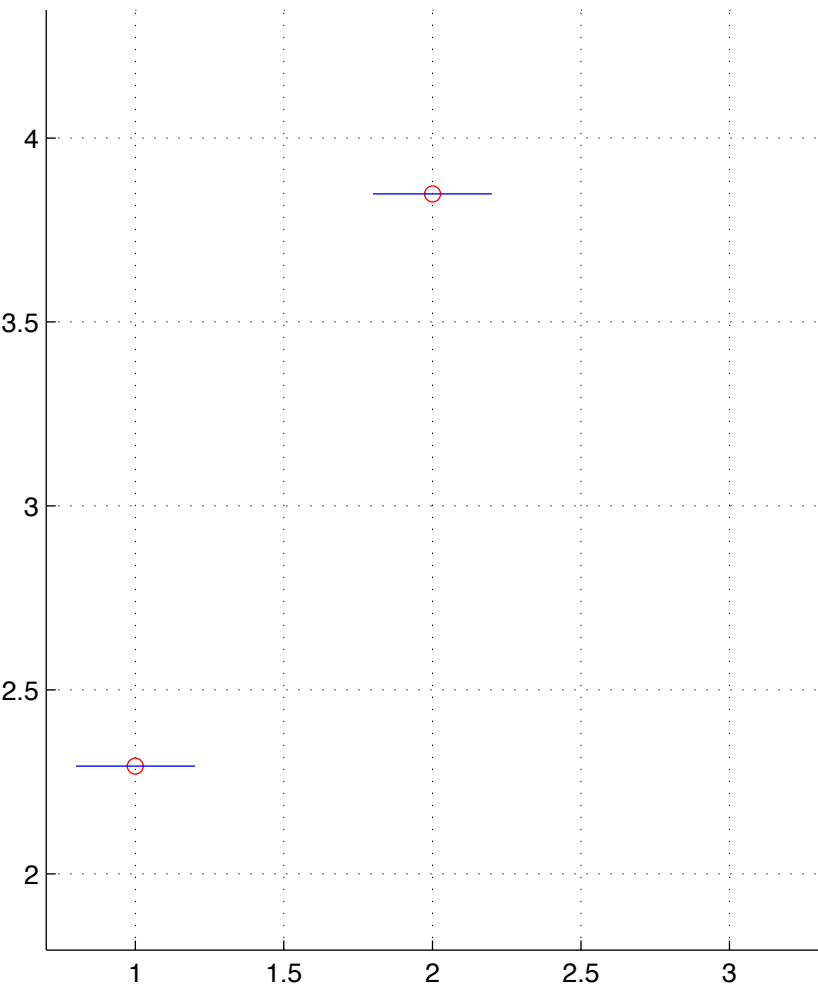
BRCA-3-T.chainID.1 numStates=2
