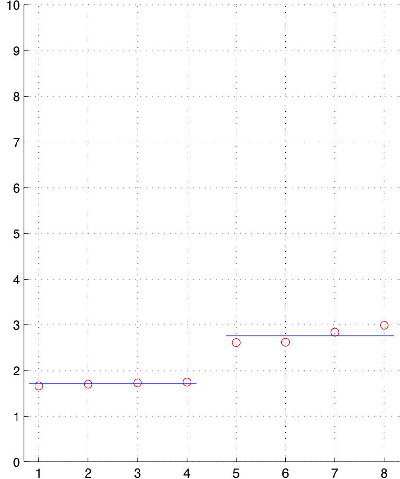
LUAD-6-T.chainID.1 numStates=2
