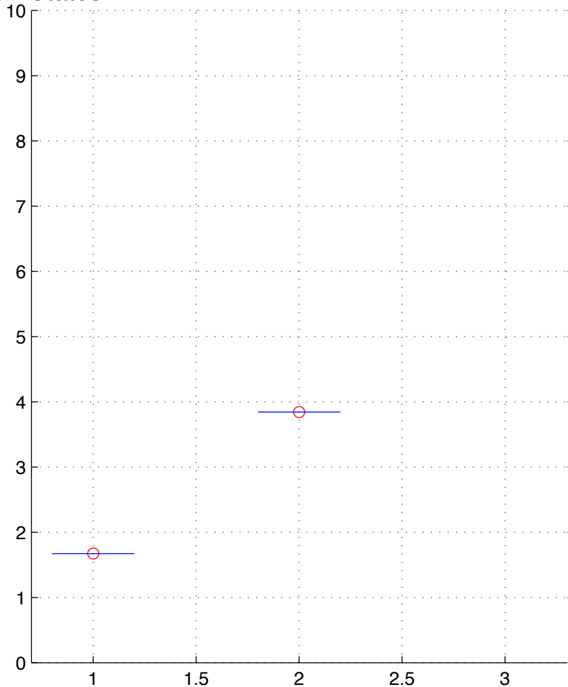
LUSC-11-T.chainID.2 numStates=2
