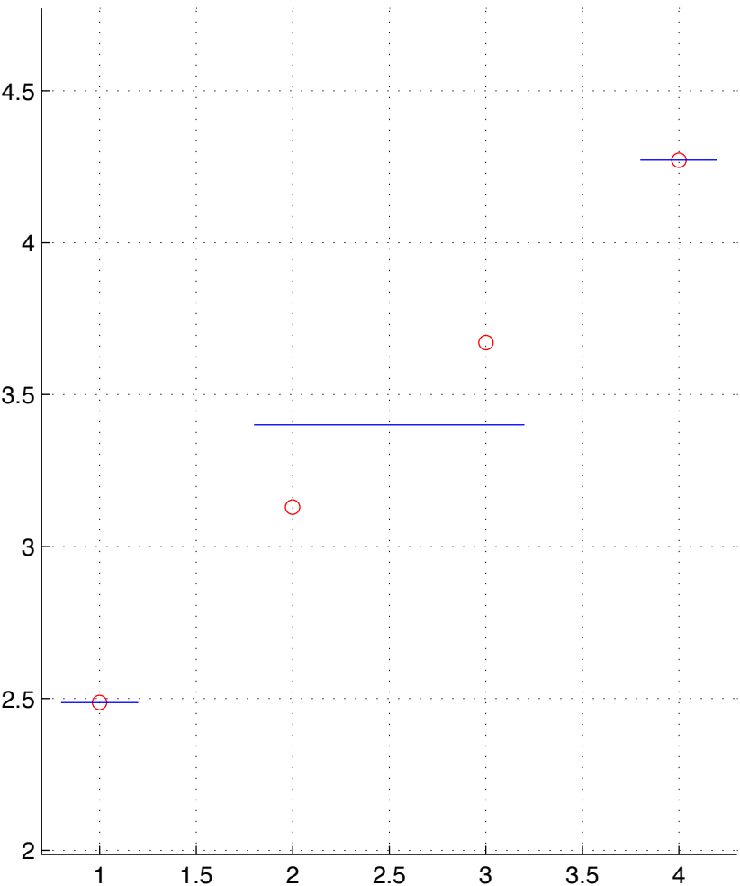
BRCA-4-T.chainID.1 numStates=3
