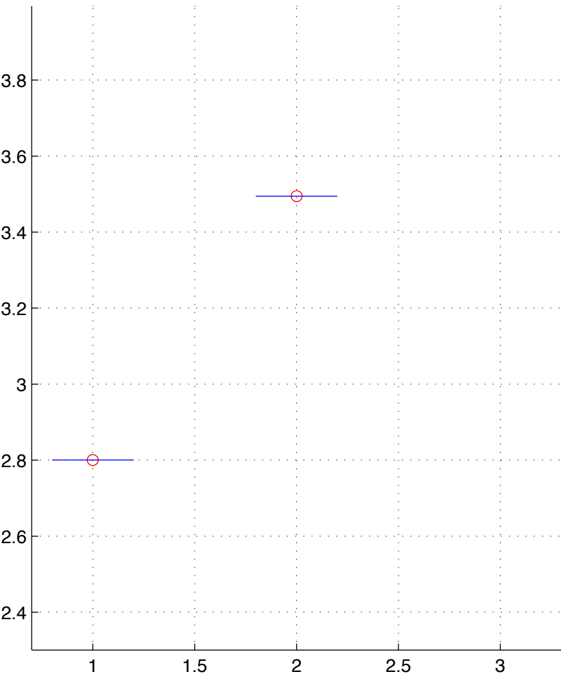
LUSC-13-T.chainID.1 numStates=2
