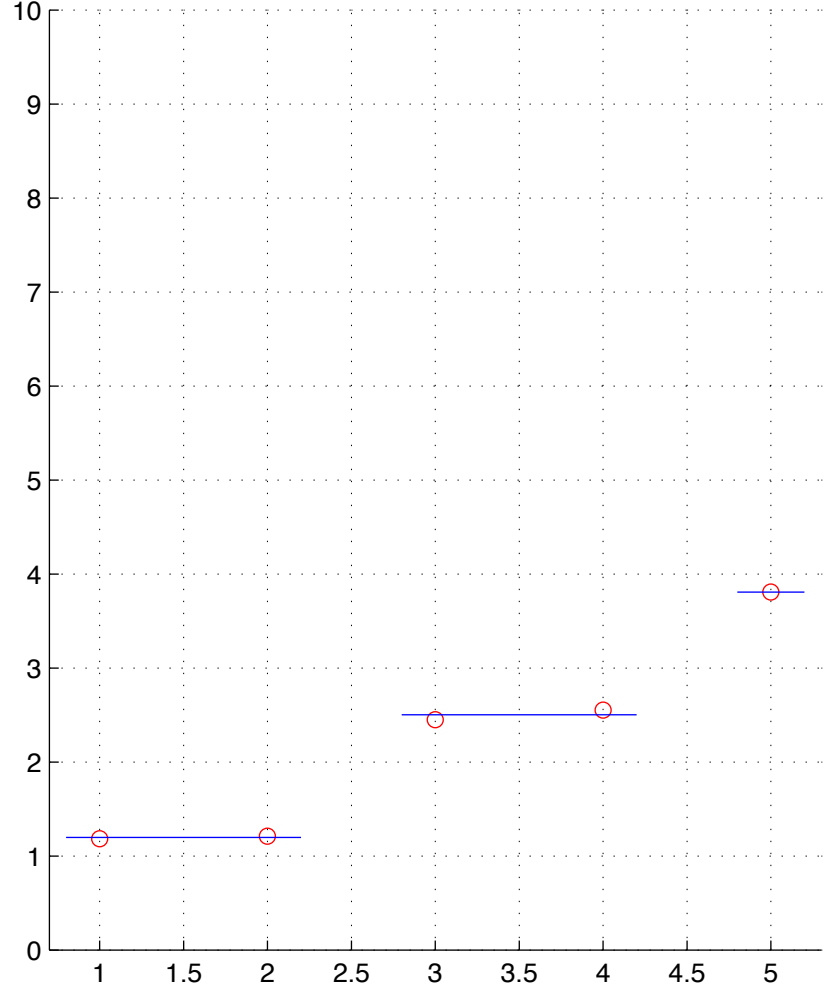
BRCA-4-T.chainID.8 numStates=3
