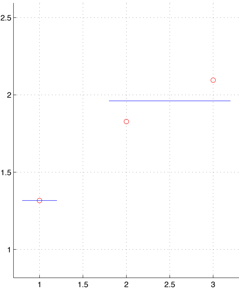
GBM-6-T.chainID.3 numStates=2
