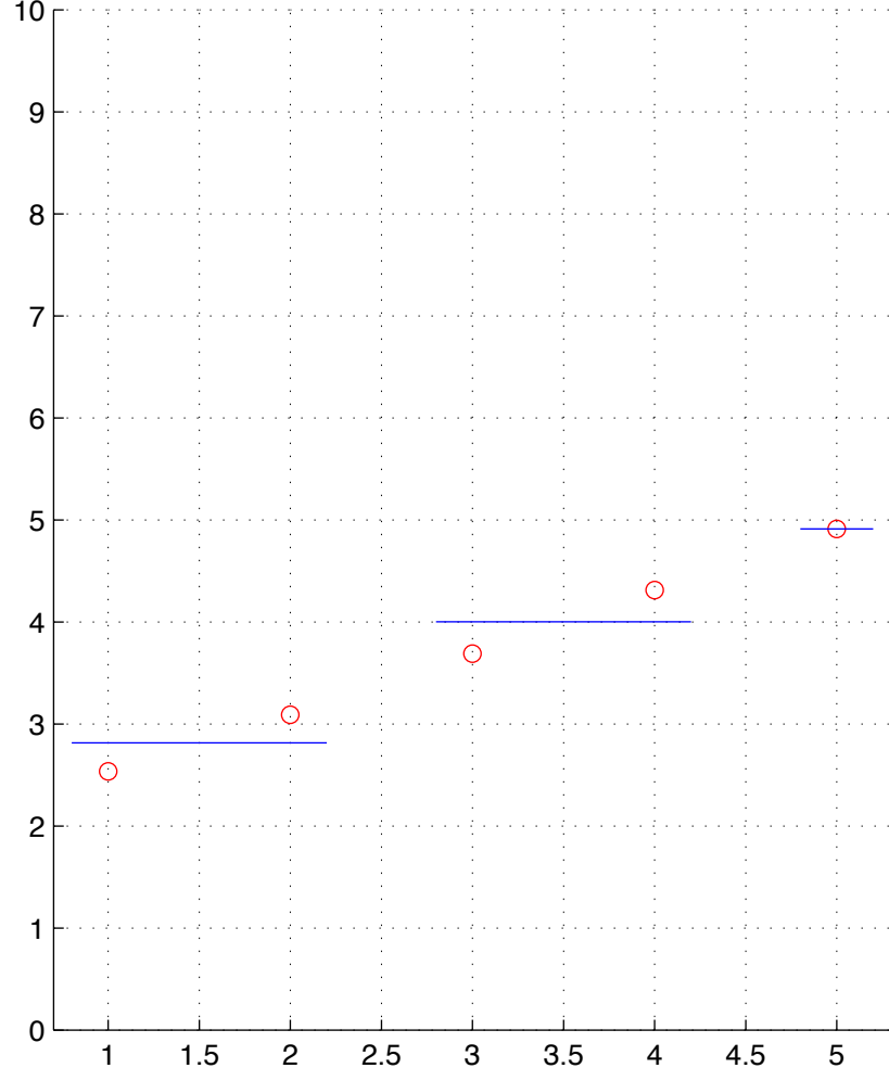
LUSC-9-T.chainID.1 numStates=3
