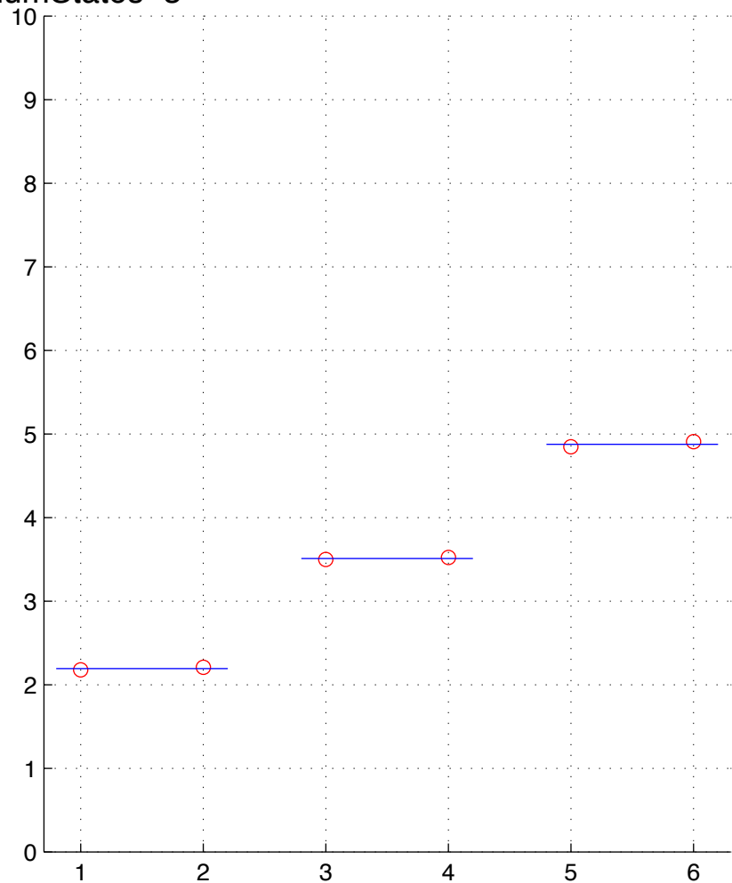
LUSC-13-T.chainID.10 numStates=3
