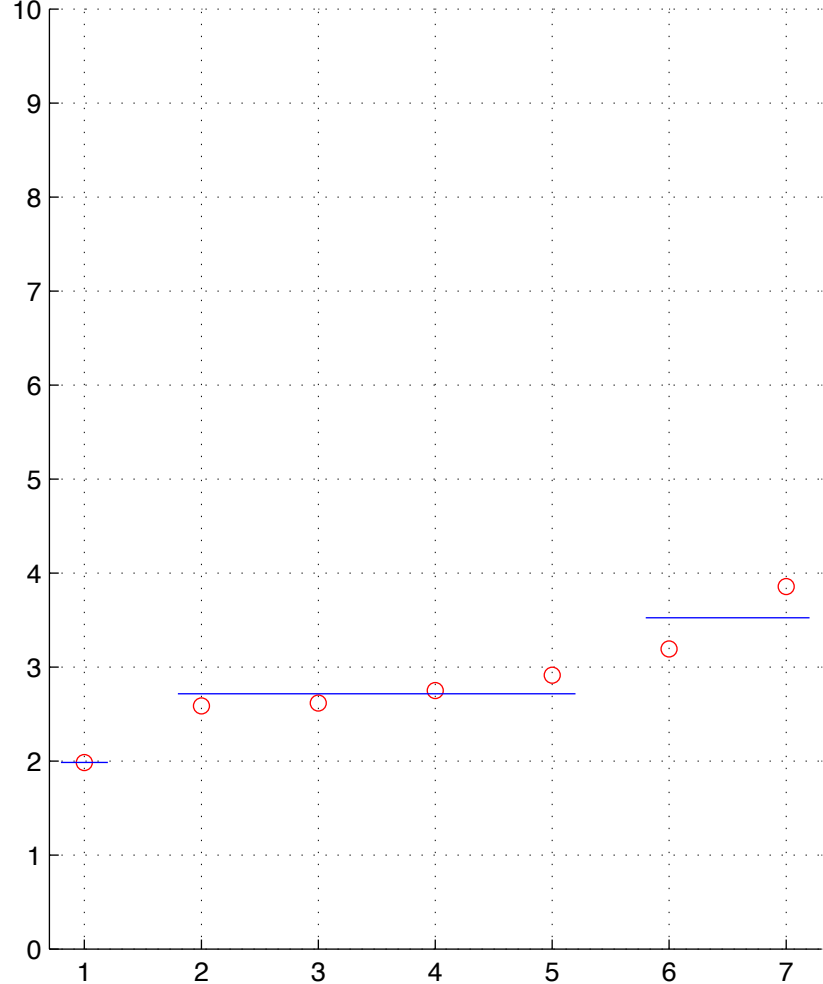
READ-1-T.chainID.1 numStates=3
