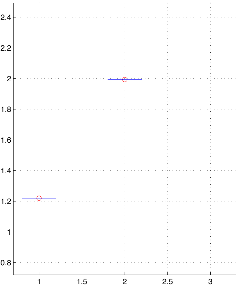
GBM-16-T.chainID.2 numStates=2
