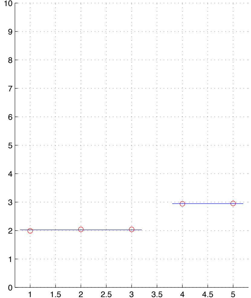
GBM-17-T.chainID.2 numStates=2
