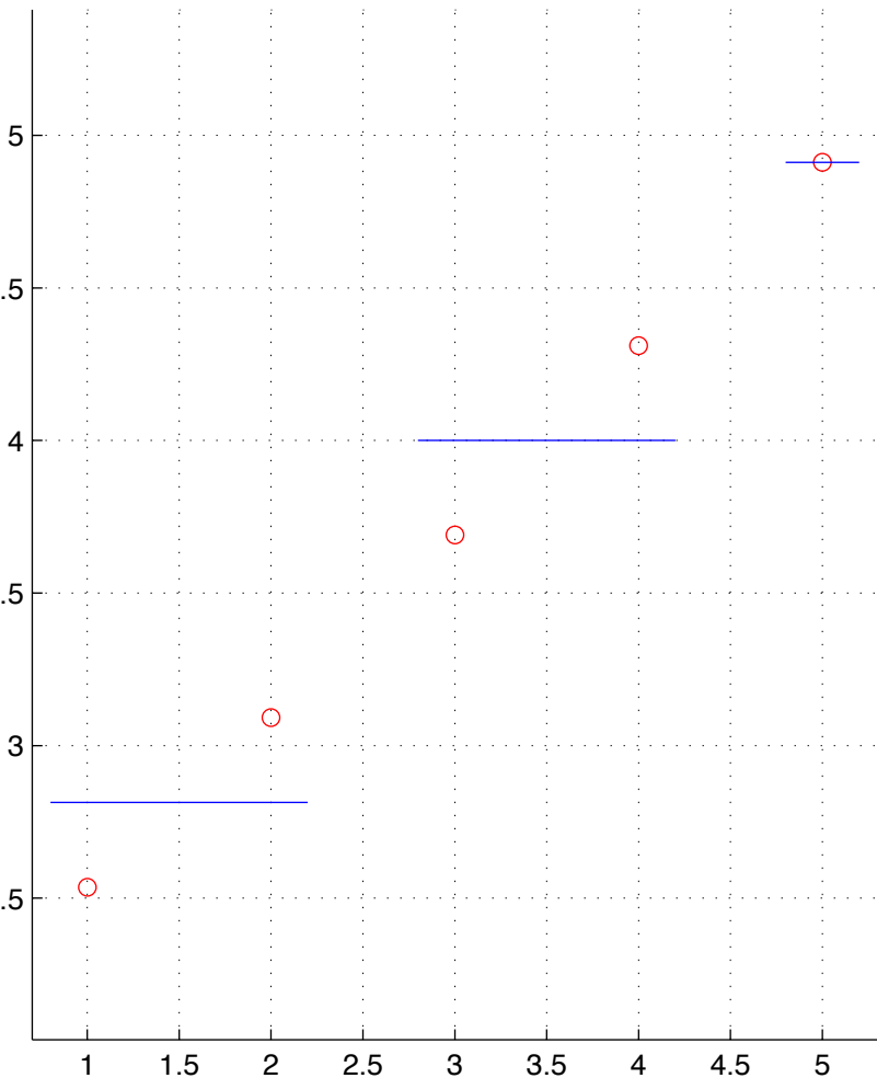
LUSC-9-T.chainID.1 numStates=3
