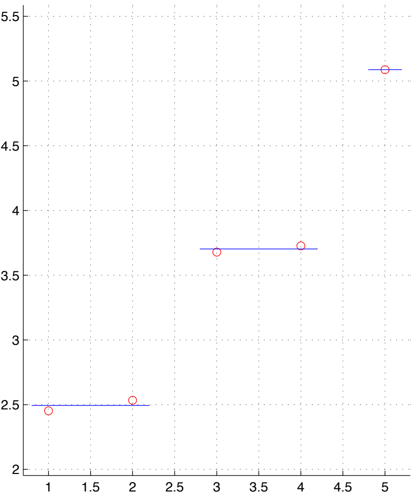
BRCA-4-T.chainID.2 numStates=3
