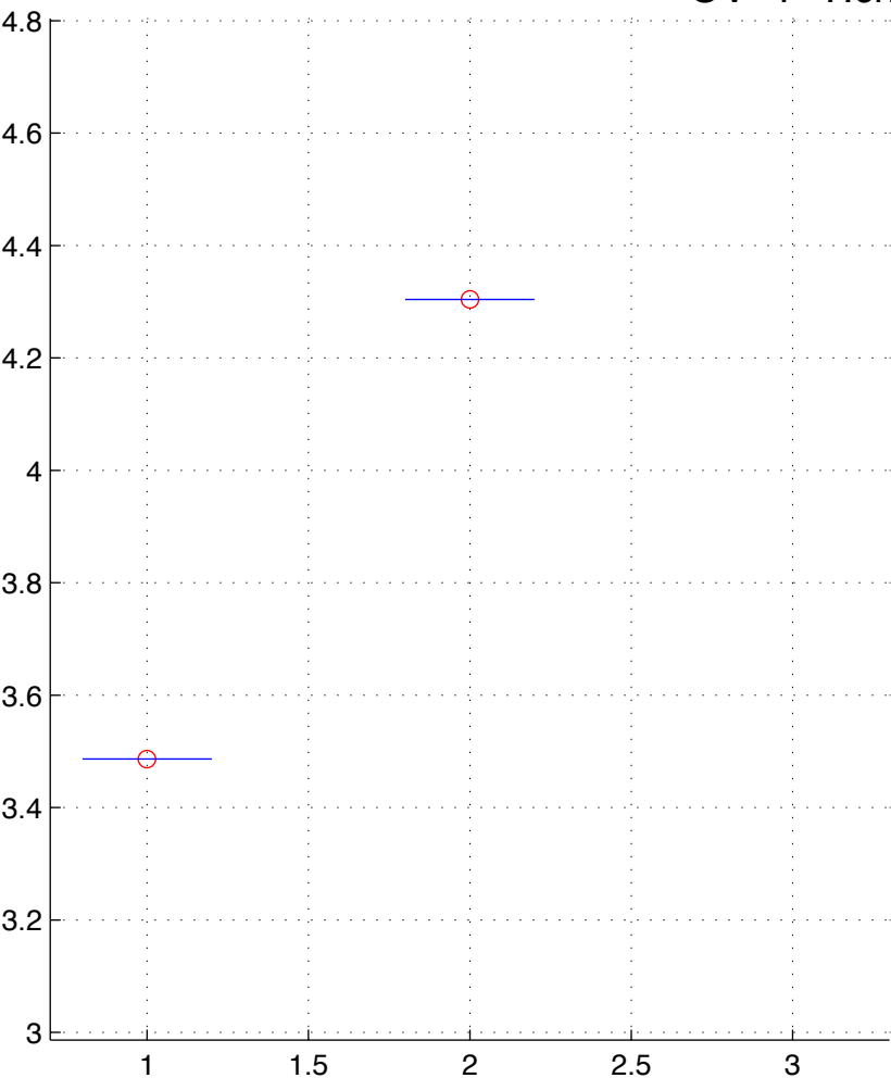
OV-1-T.chainID.1 numStates=2
