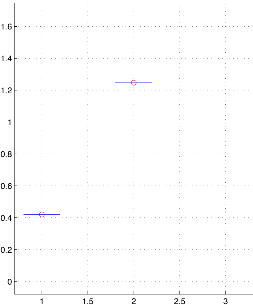
GBM-6-T.chainID.2 numStates=2
