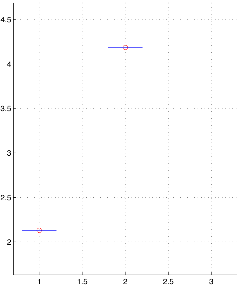
LUSC-5-T.chainID.2 numStates=2
