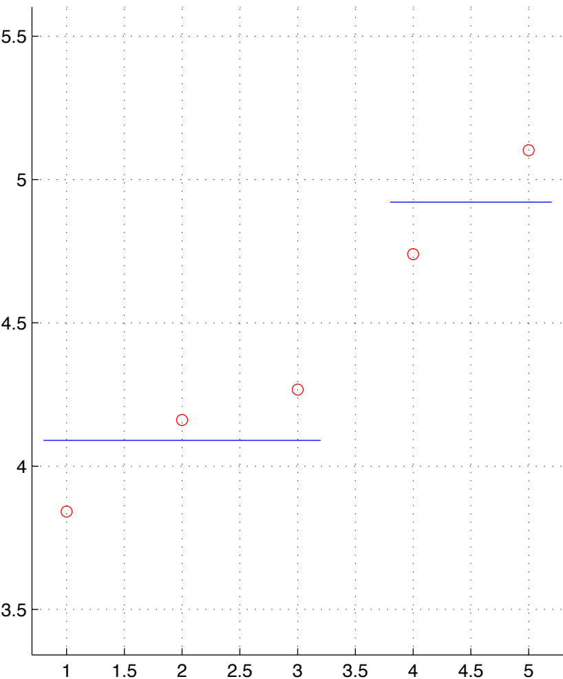
OV-5-T.chainID.1 numStates=2
