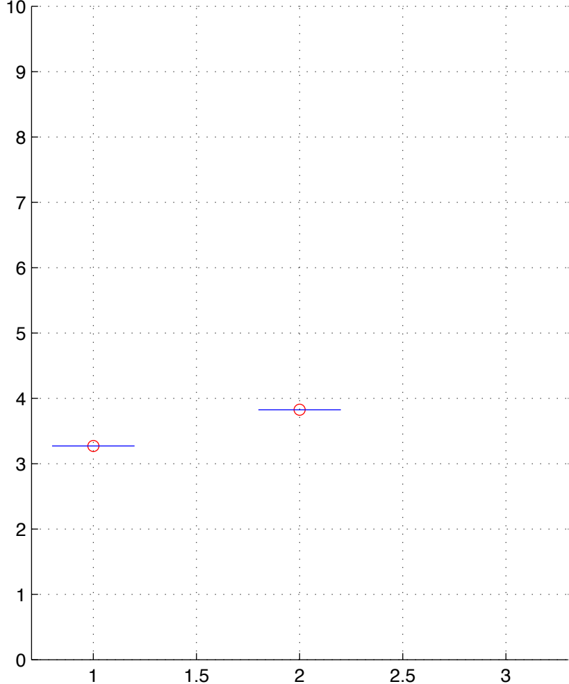
LUSC-13-T.chainID.3 numStates=2
