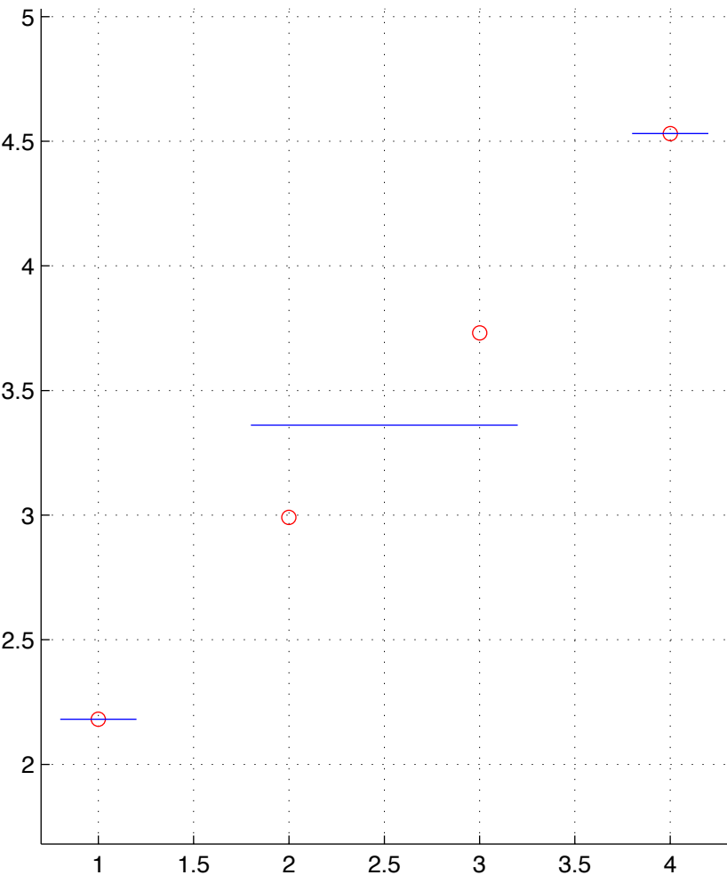
LUSC-13-T.chainID.6 numStates=3
