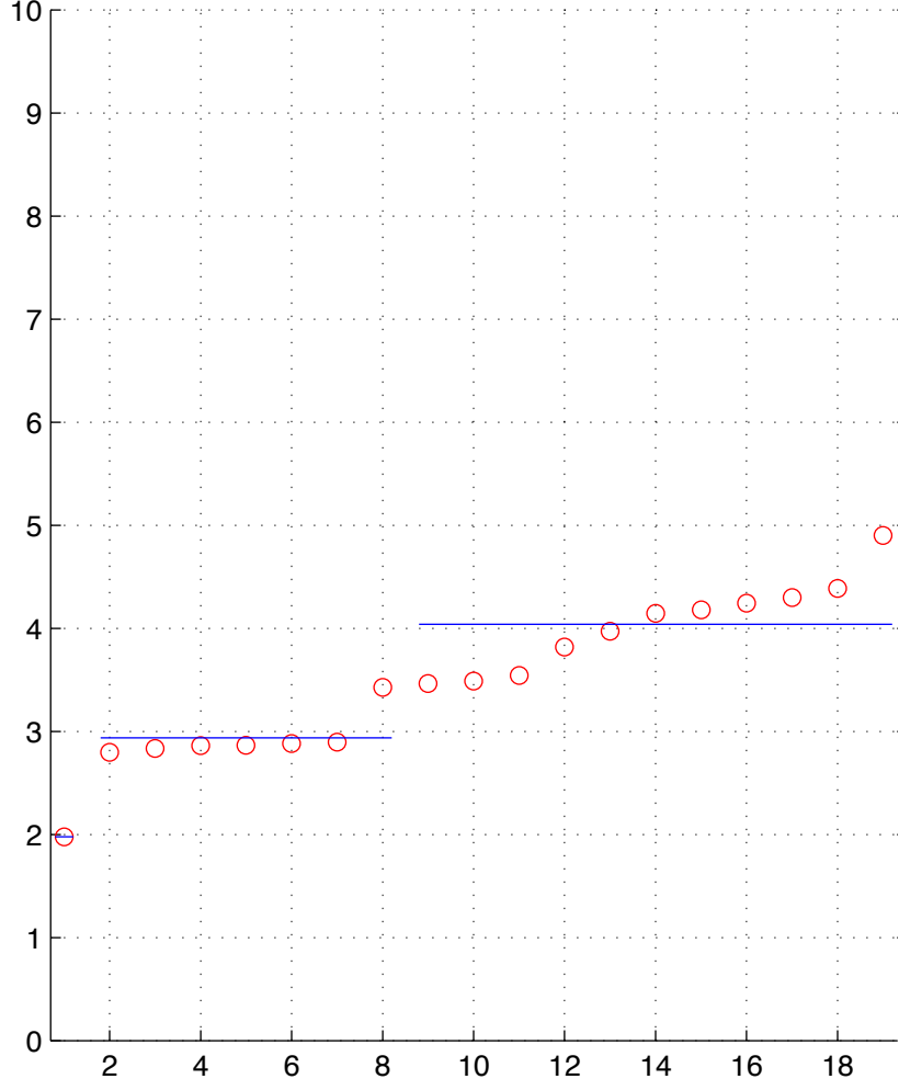
LUSC-12-T.chainID.2 numStates=3
