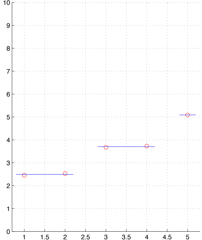
BRCA-4-T.chainID.2 numStates=3
