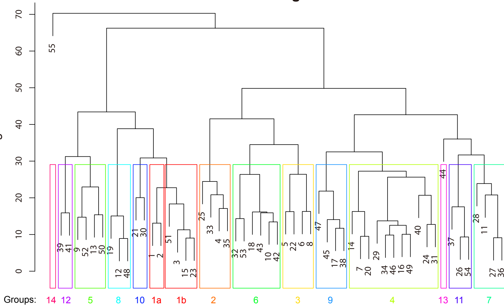
Cluster dendrogram
