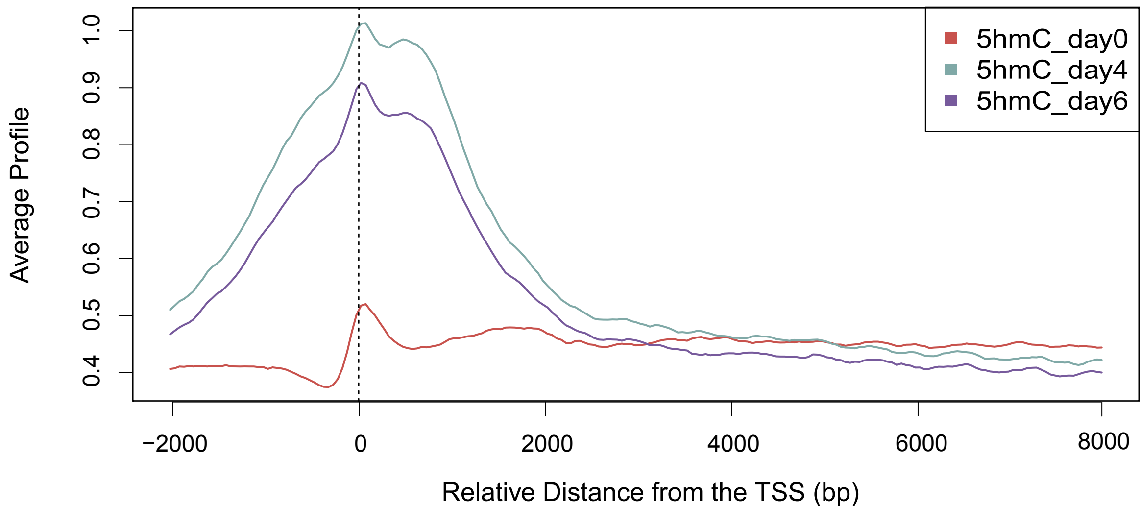
Average profiles of 5-hmC around TSS
