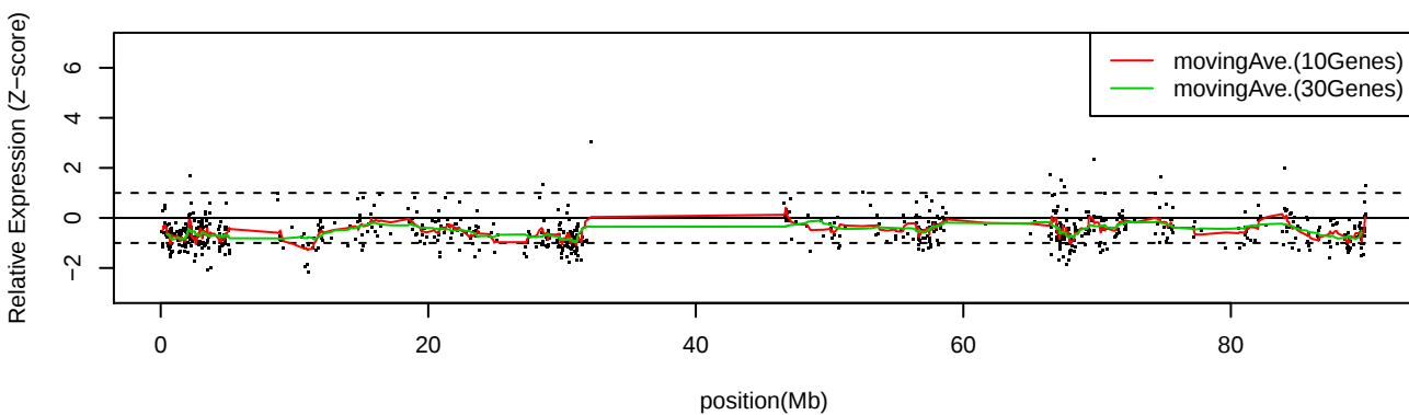
LC_S3 Chr16
