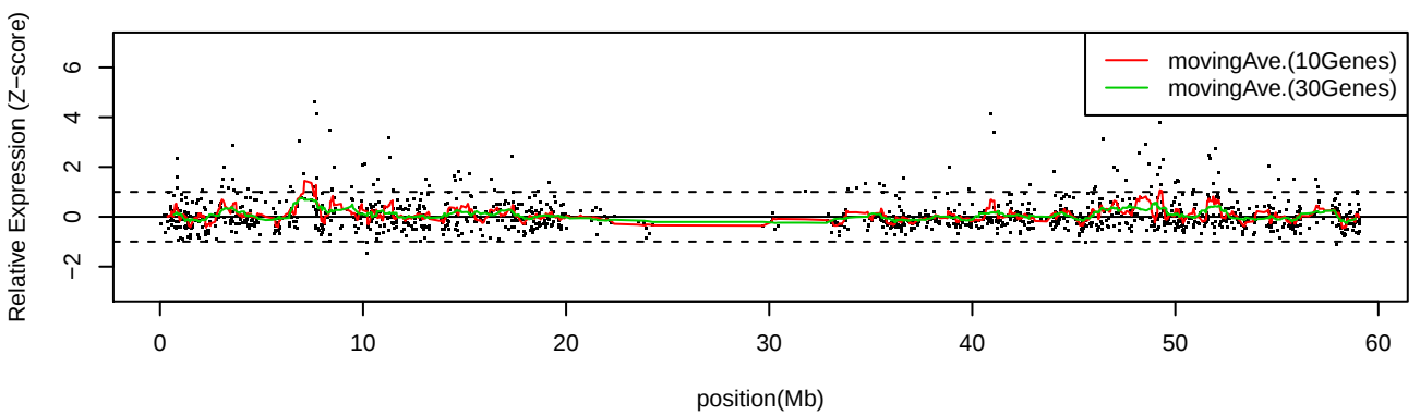
LC_S52 Chr19
