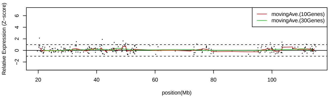
LC_S2 Chr13
