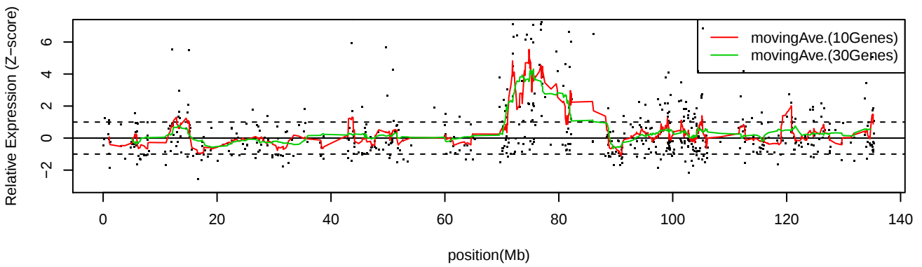
LC_S51 Chr10
