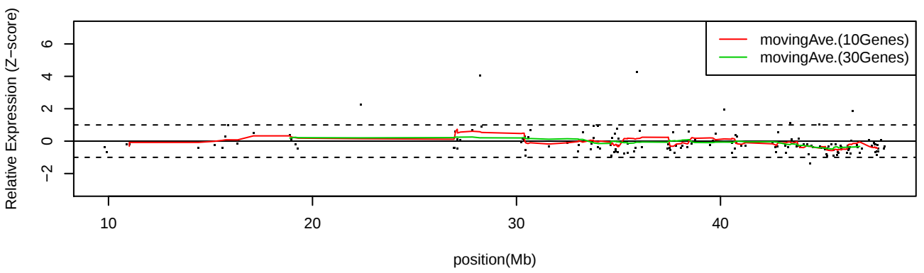
LC_S50 Chr21
