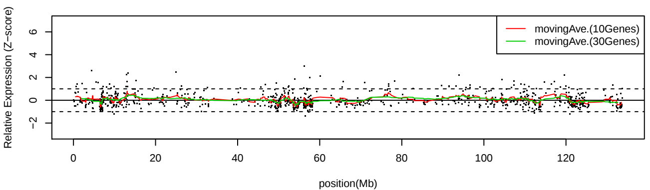
LC_S50 Chr12
