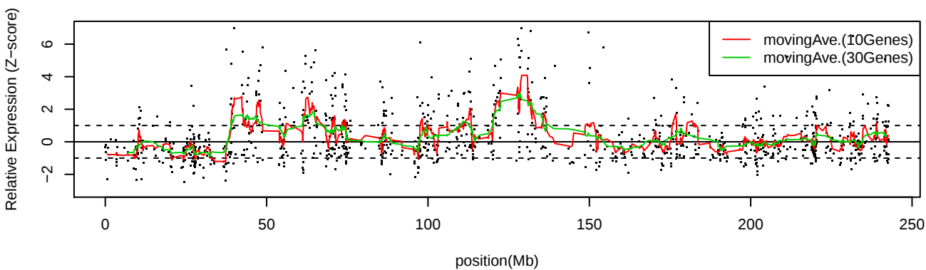
LC_S51 Chr2
