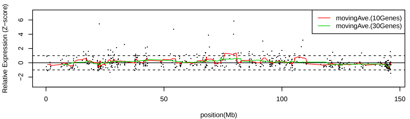
LC_S5 Chr8
