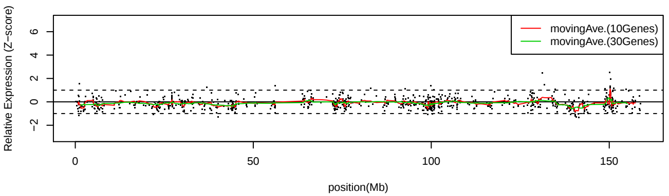
LC_S2 Chr7
