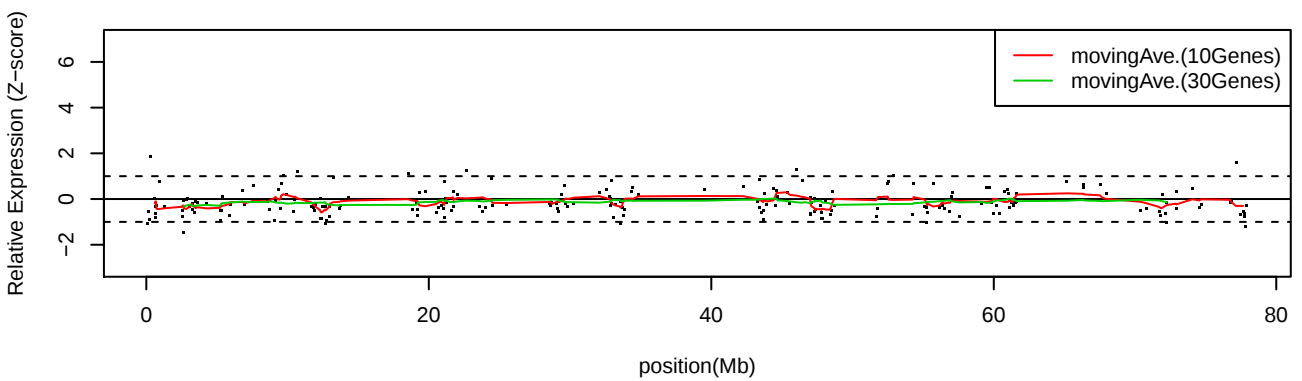
LC_S50 Chr18
