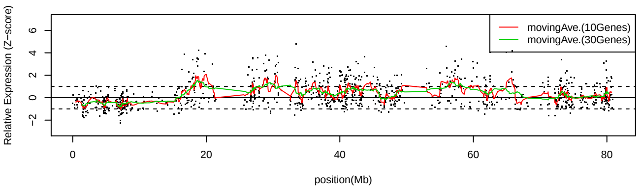
LC_S3 Chr17
