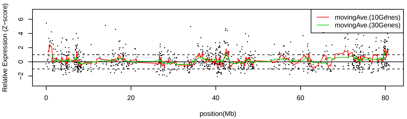
LC_S51 Chr17
