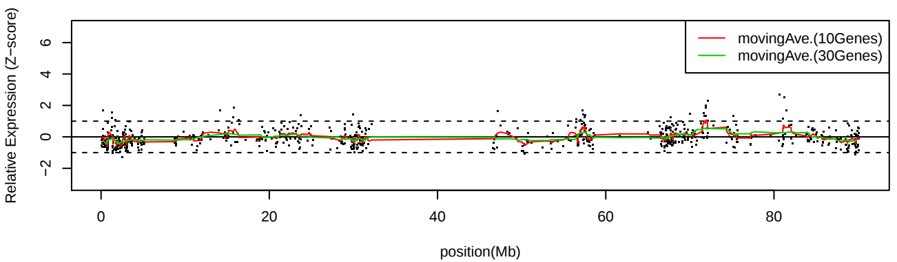
LC_S2 Chr16
