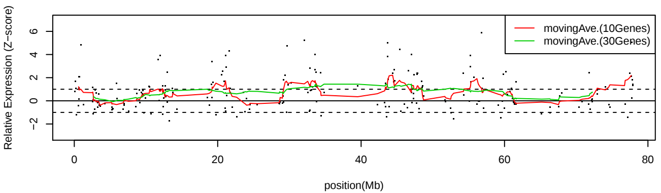
LC_S51 Chr18
