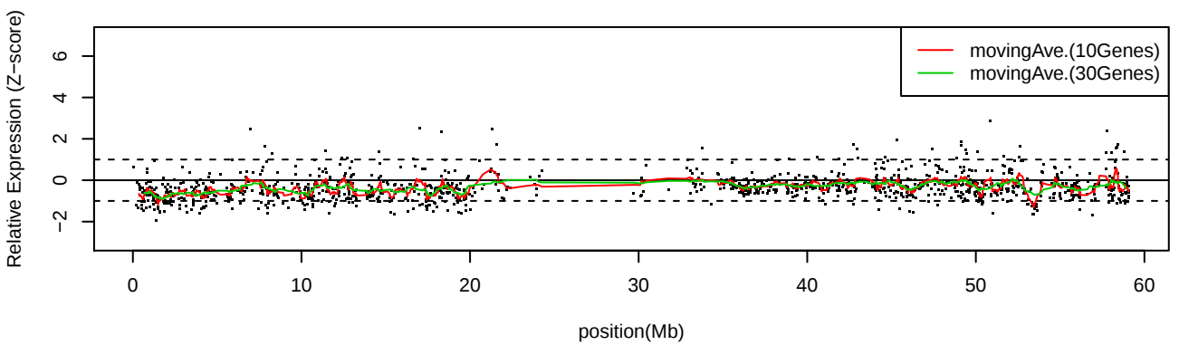
LC_S5 Chr19
