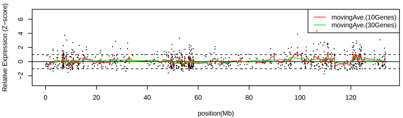
LC_S4 Chr12
