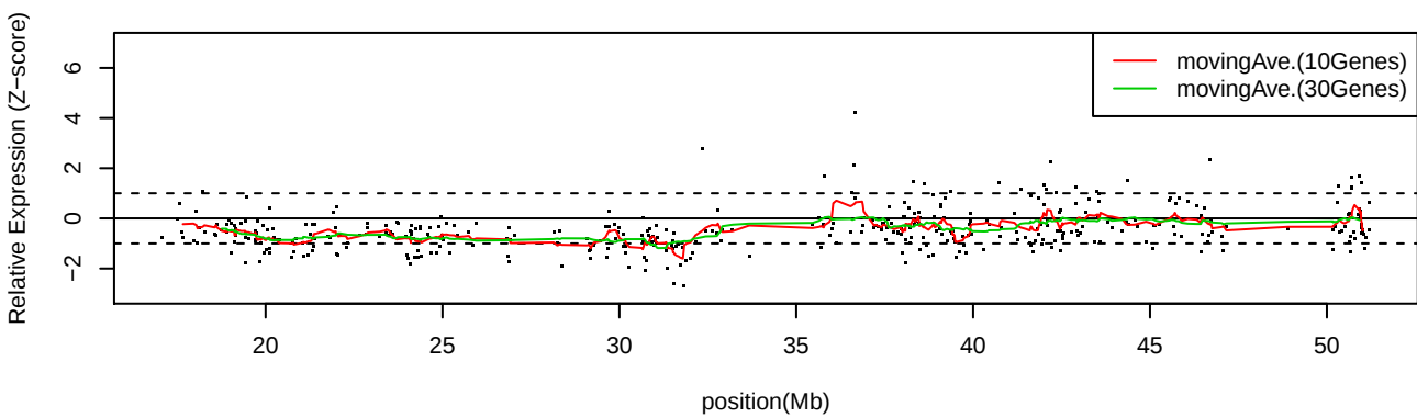
LC_S4 Chr22
