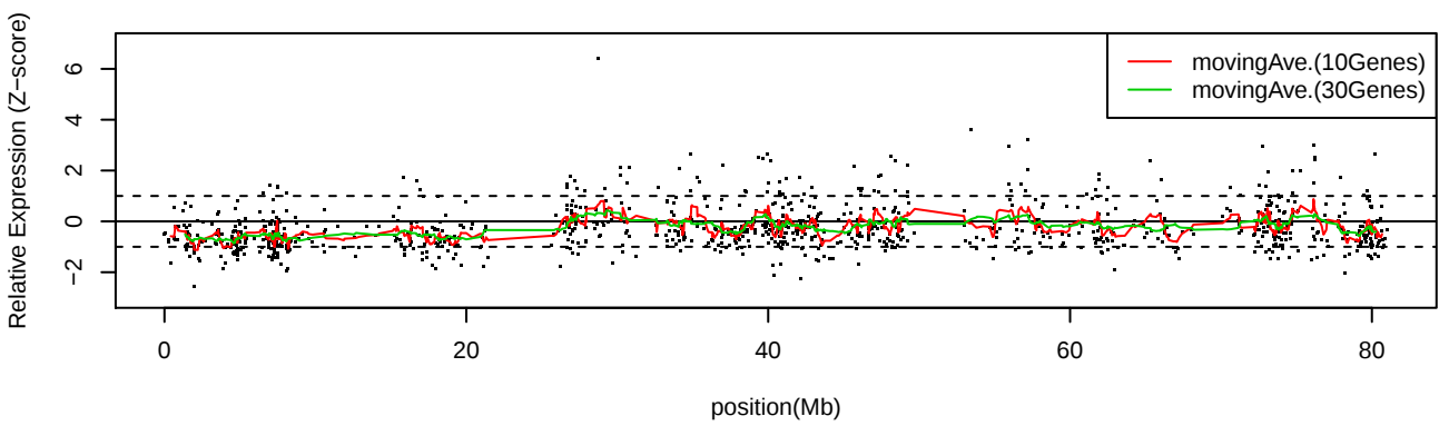
LC_S4 Chr17
