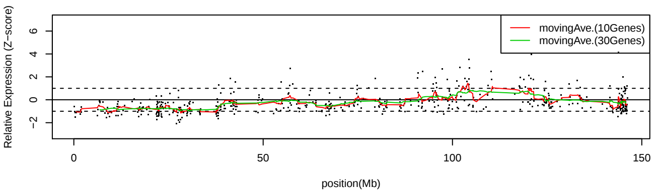
LC_S4 Chr8
