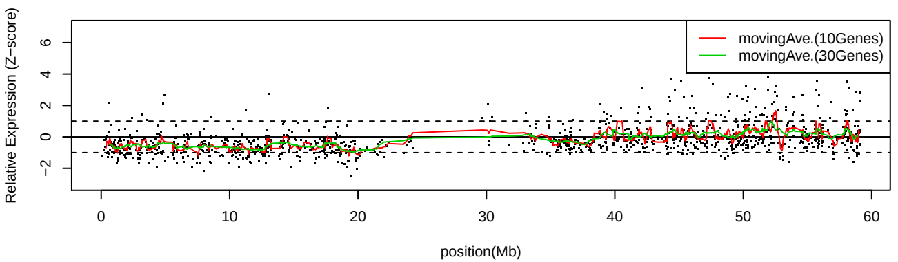
LC_S4 Chr19
