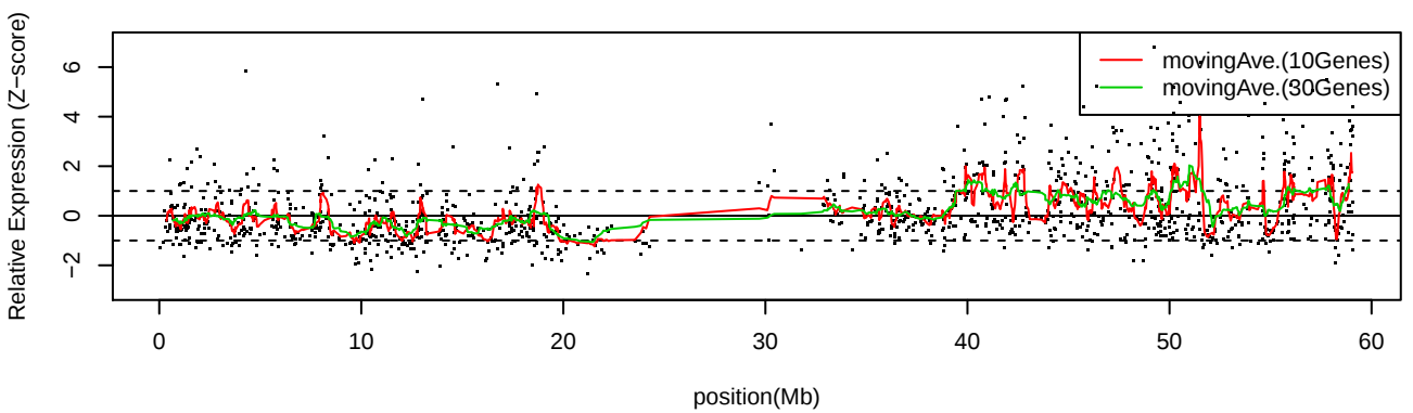
LC_S51 Chr19
