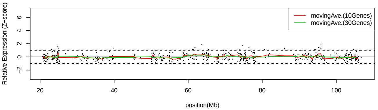
LC_S2 Chr14
