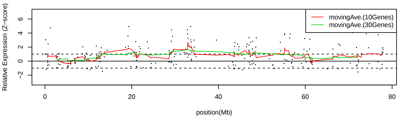
LC_S3 Chr18
