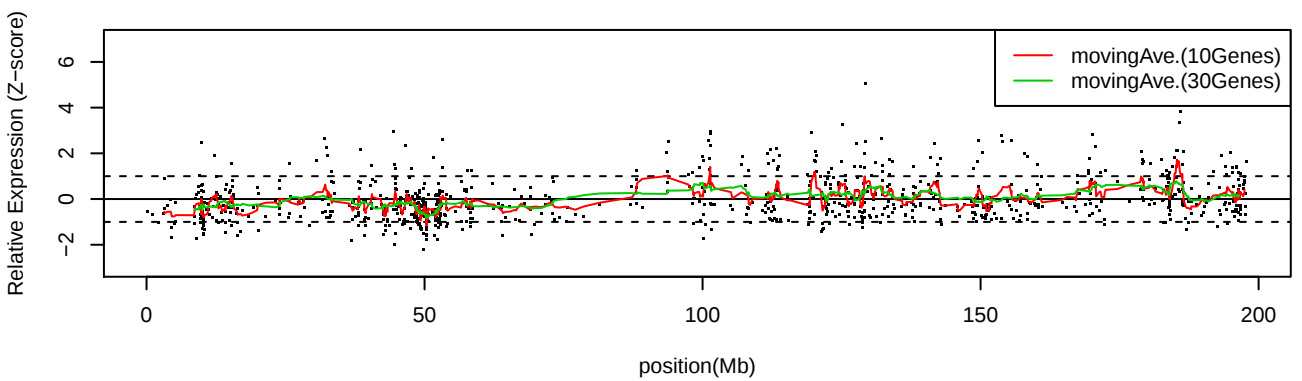
LC_S3 Chr3
