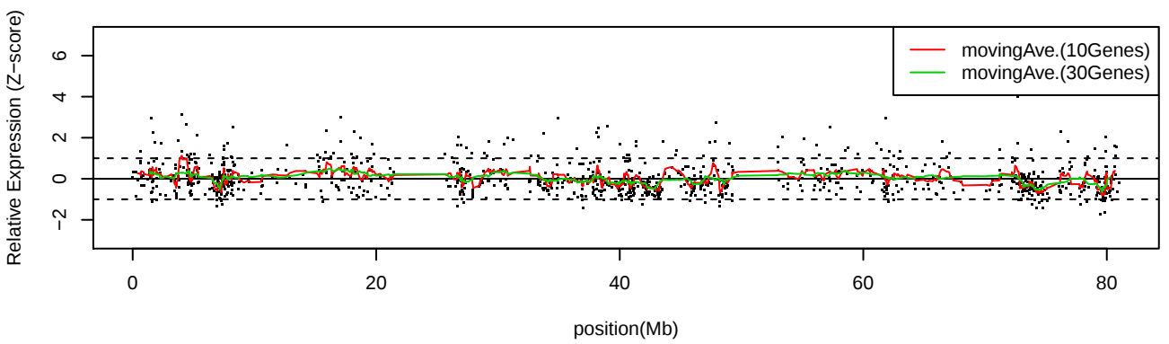
LC_S5 Chr17
