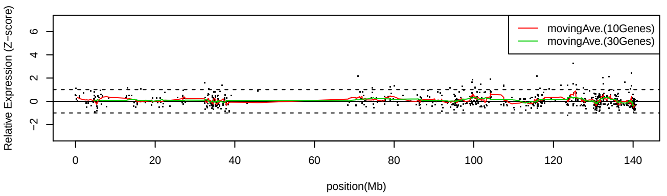
LC_S2 Chr9
