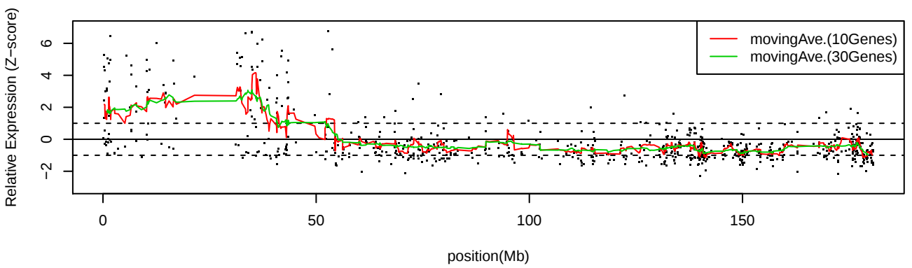
LC_S51 Chr5
