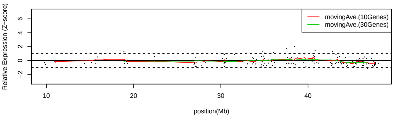
LC_S5 Chr21
