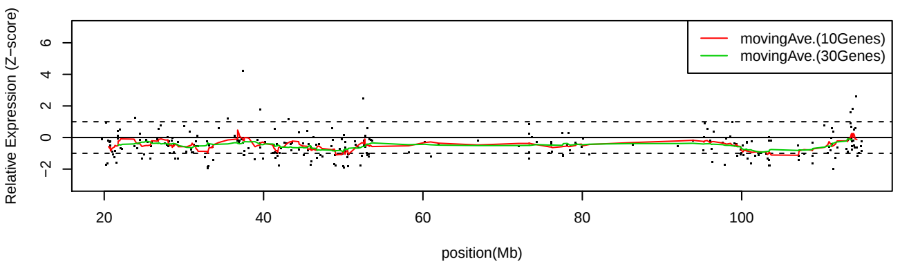
LC_S51 Chr13
