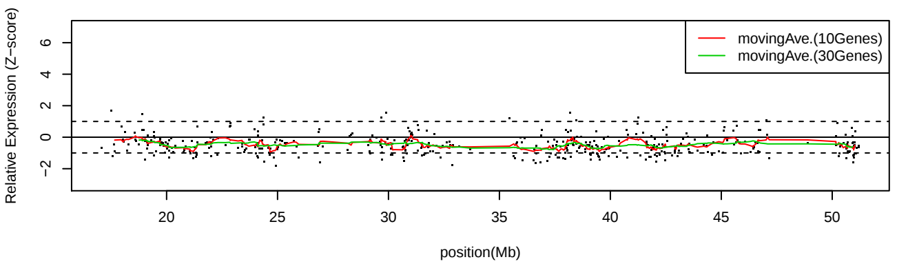
LC_S3 Chr22
