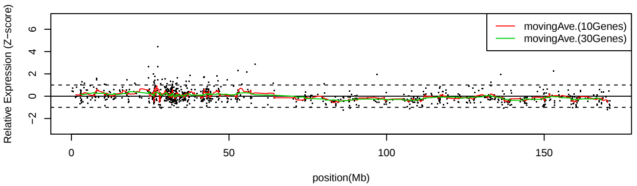
LC_S2 Chr6
