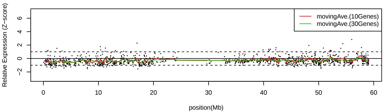
LC_S50 Chr19
