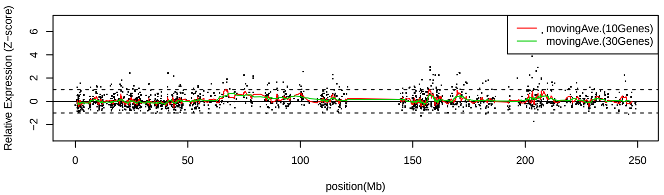
LC_S28 Chr1
