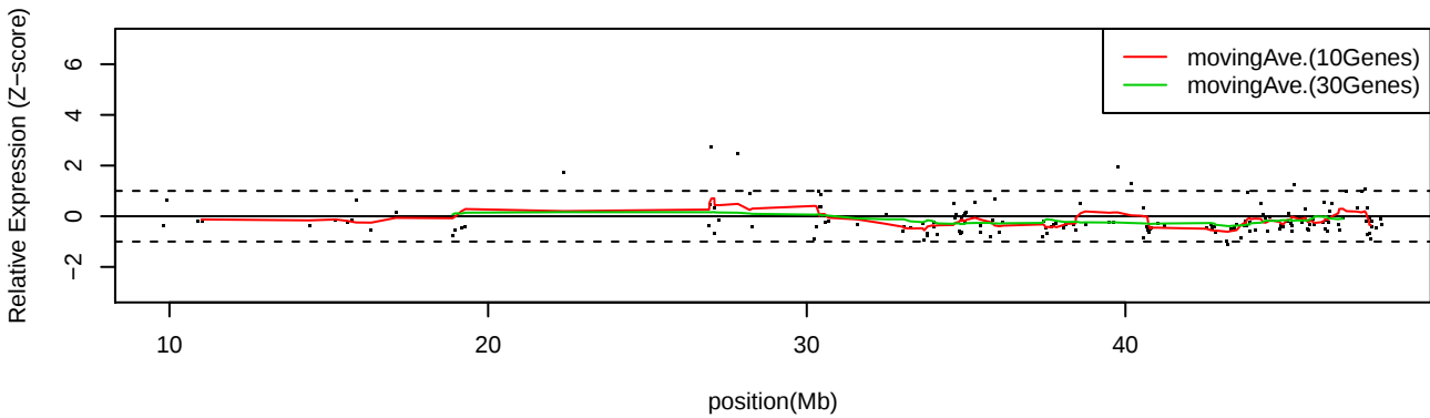
LC_S22 Chr21
