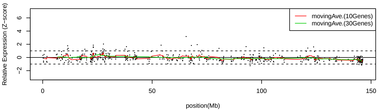
LC_S28 Chr8
