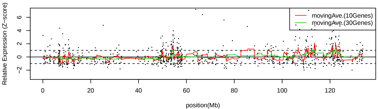
LC_S23 Chr12
