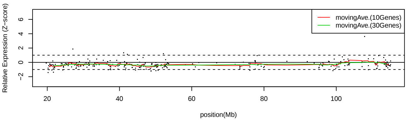
LC_S24 Chr13
