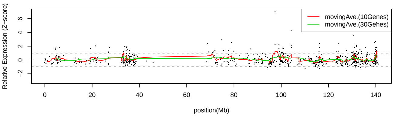
LC_S30 Chr9
