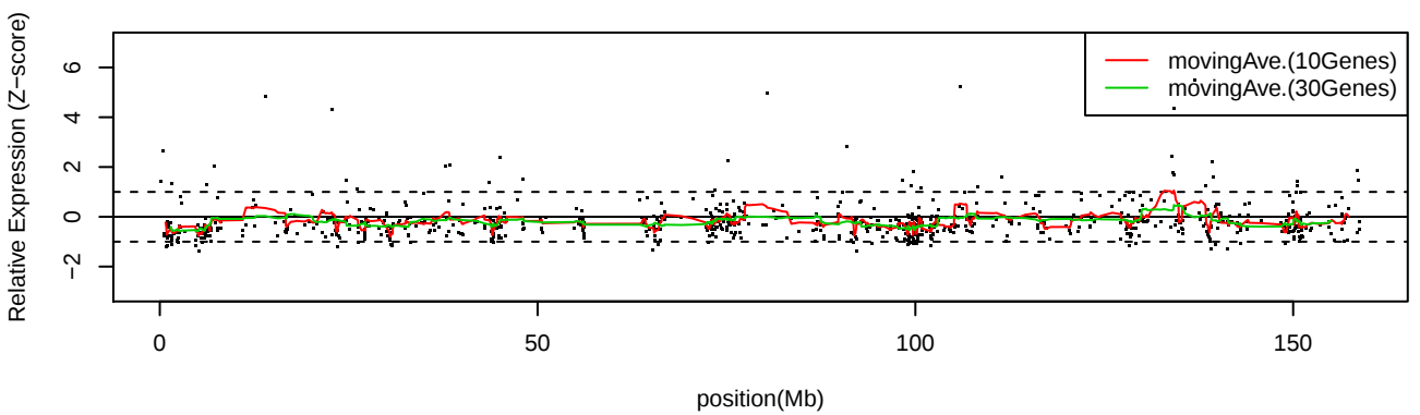
LC_S26 Chr7
