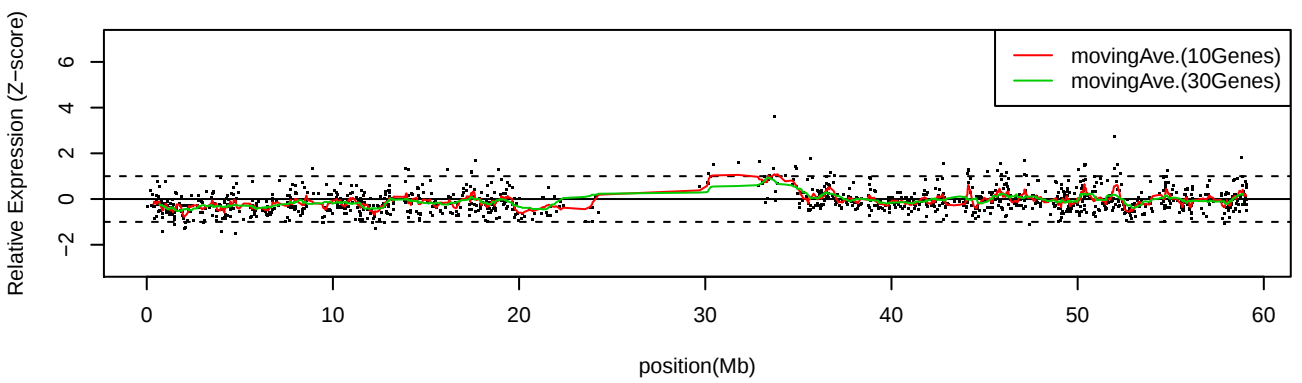
LC_S29 Chr19
