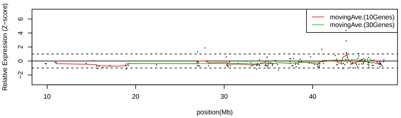
LC_S30 Chr21
