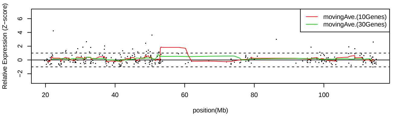
LC_S26 Chr13
