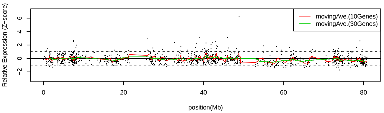
LC_S30 Chr17
