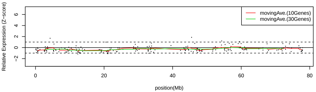
LC_S26 Chr18
