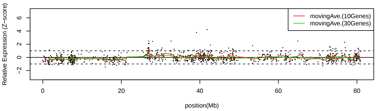
LC_S29 Chr17
