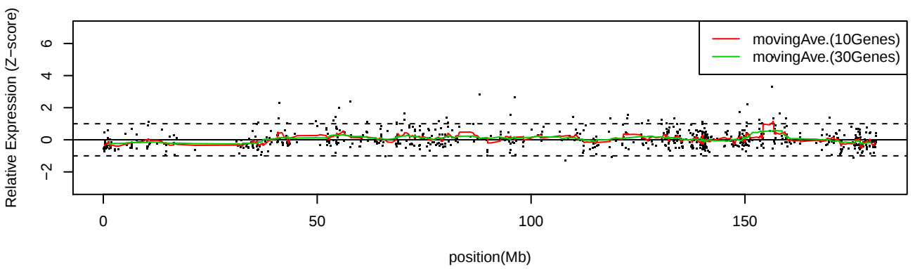
LC_S28 Chr5
