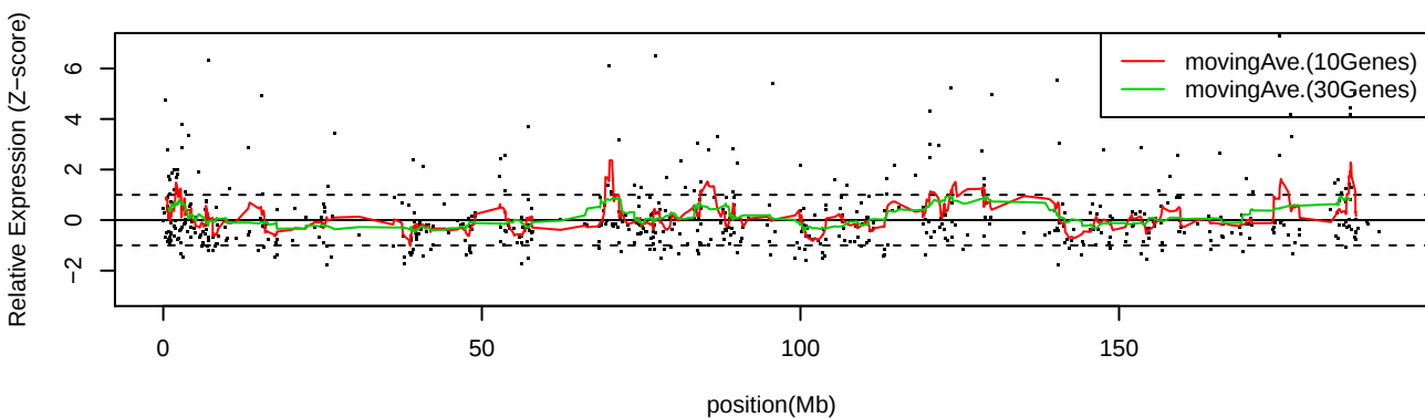
LC_S23 Chr4
