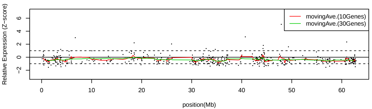
LC_S21 Chr20
