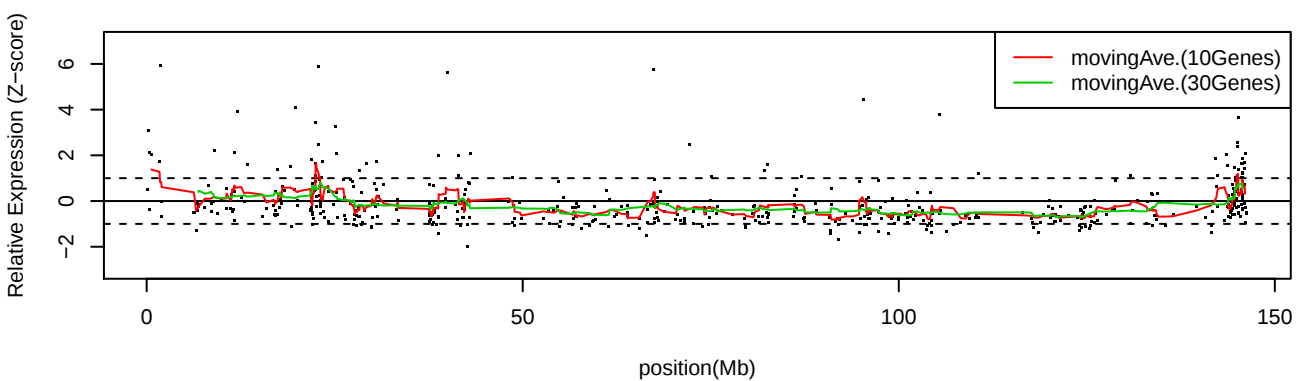
LC_S27 Chr8
