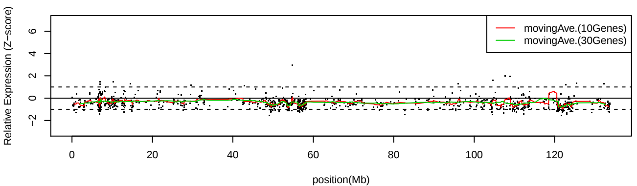
LC_S26 Chr12
