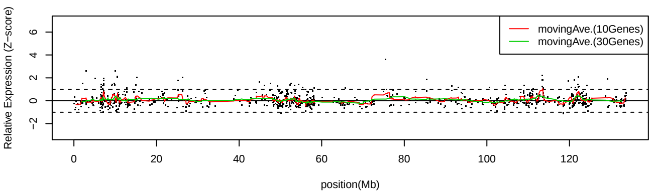
LC_S28 Chr12
