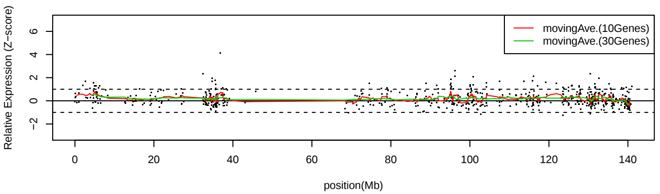
LC_S28 Chr9
