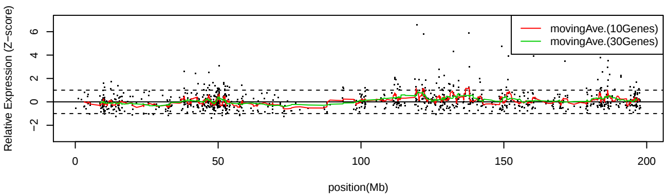
LC_S30 Chr3
