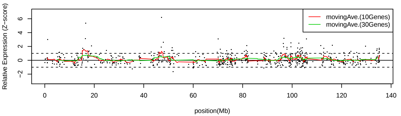
LC_S30 Chr10
