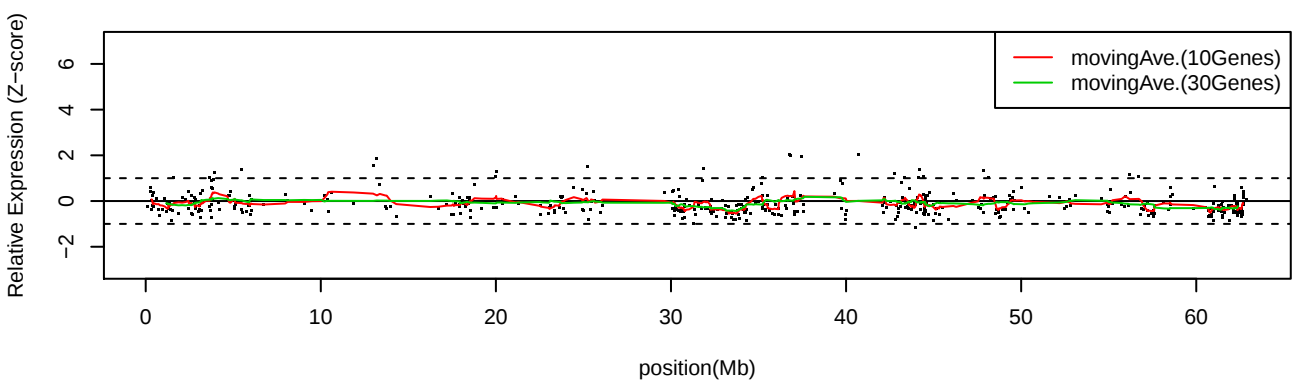
LC_S28 Chr20
