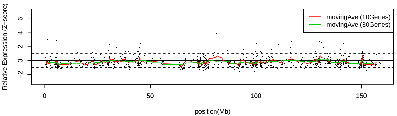
LC_S22 Chr7
