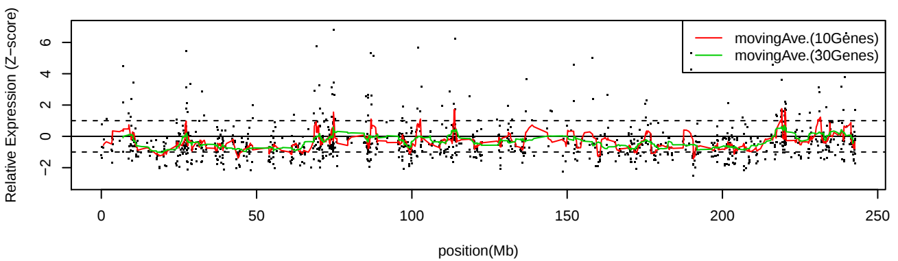
LC_S10 Chr2
