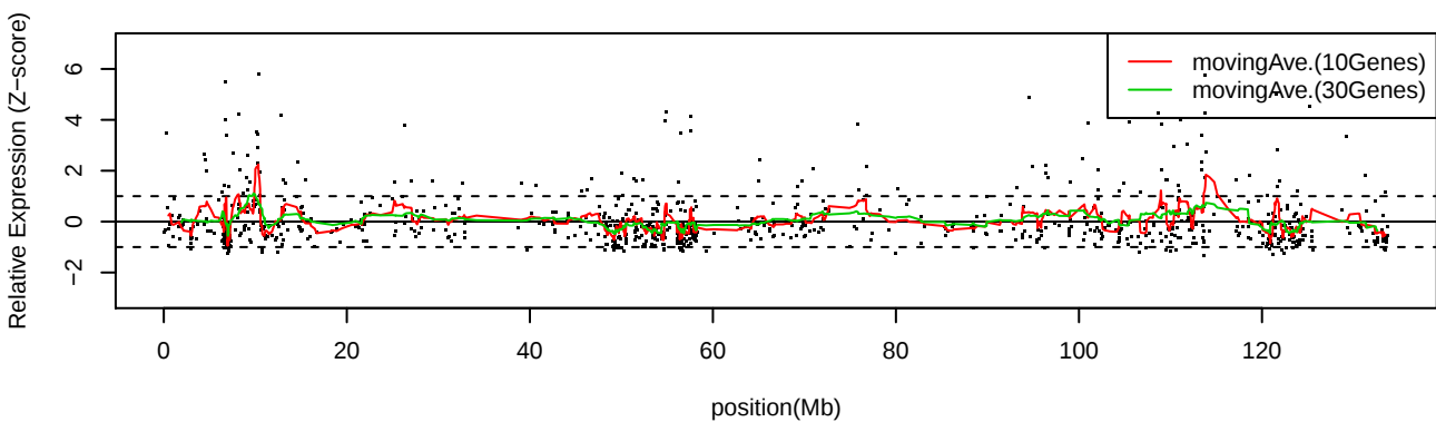
LC_C31 Chr12
