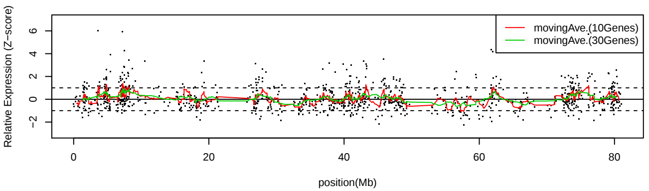
LC_S8 Chr17
