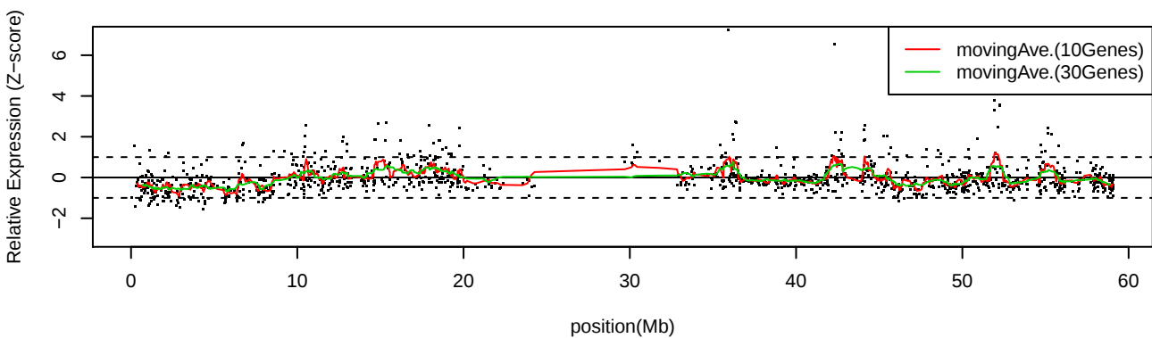
LC_C35 Chr19
