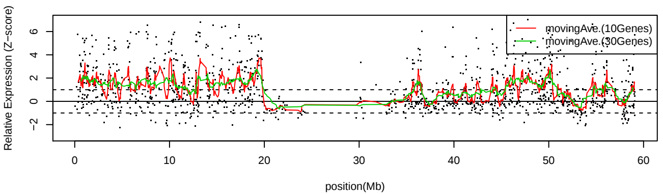
LC_S6 Chr19
