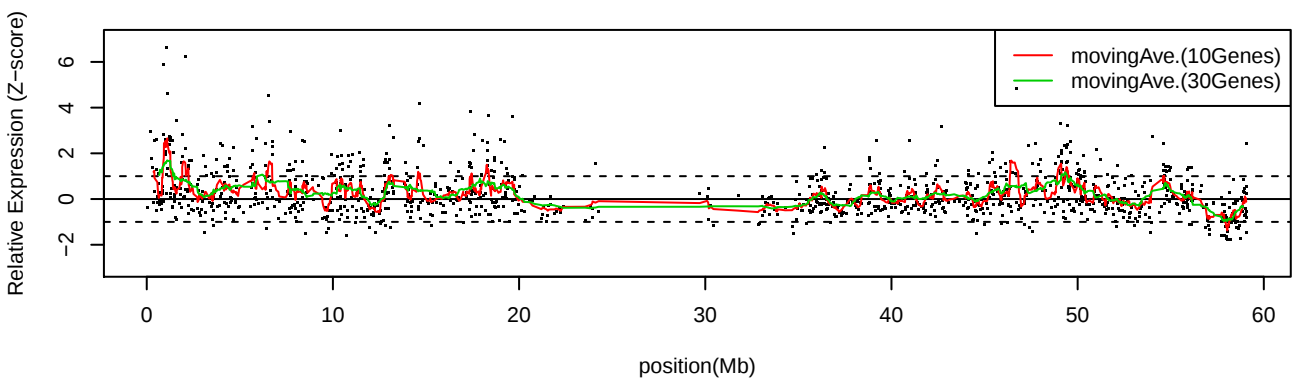
LC_S9 Chr19
