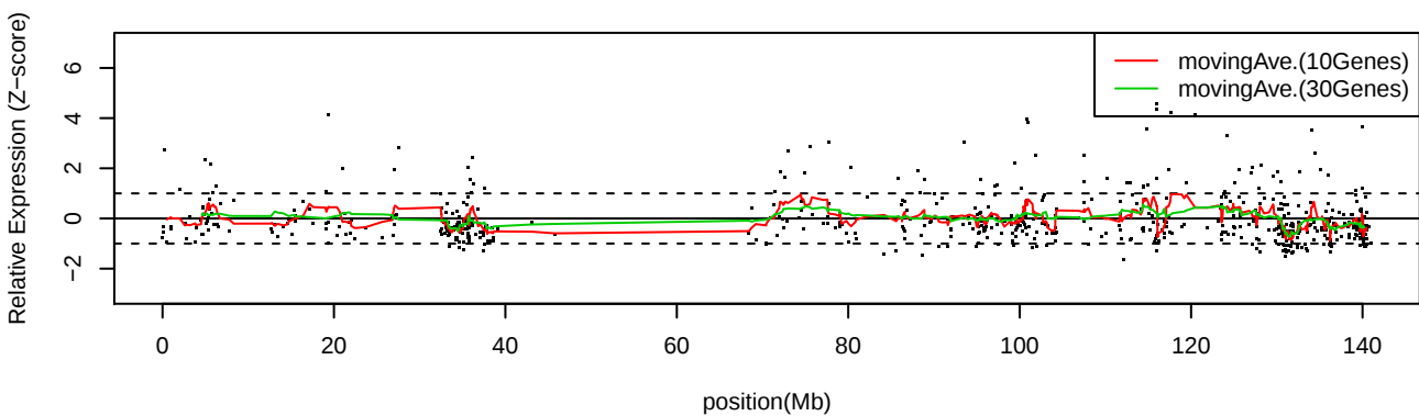
LC_C31 Chr9
