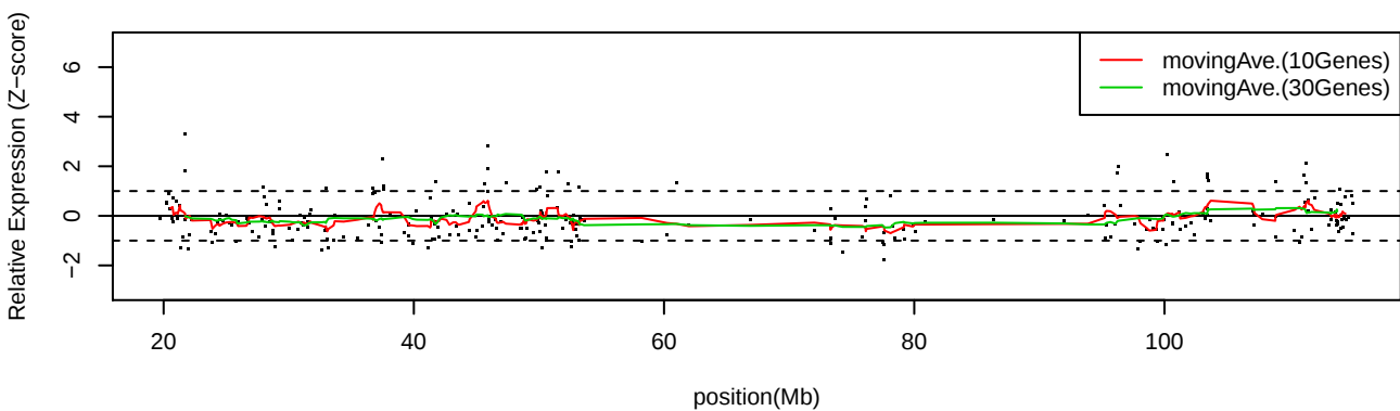
LC_S9 Chr13
