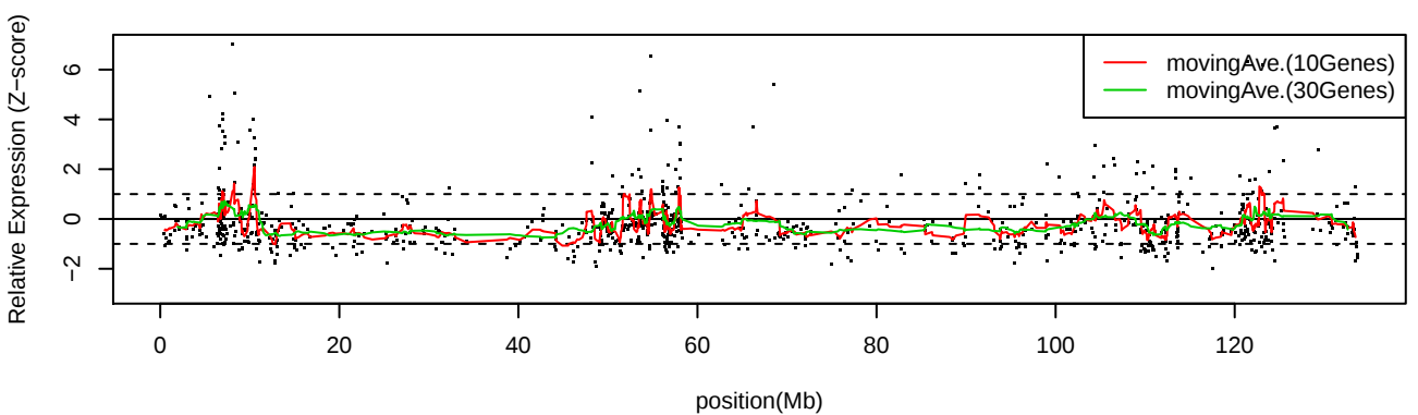
LC_S10 Chr12
