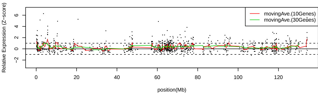
LC_C36 Chr11
