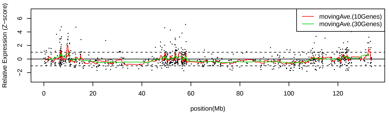
LC_S8 Chr12
