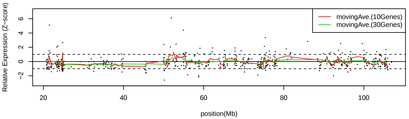
LC_C34 Chr14
