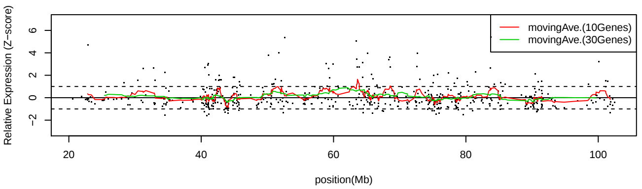
LC_C31 Chr15
