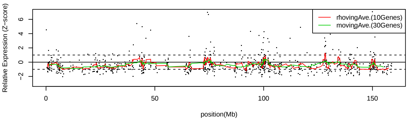
LC_S10 Chr7
