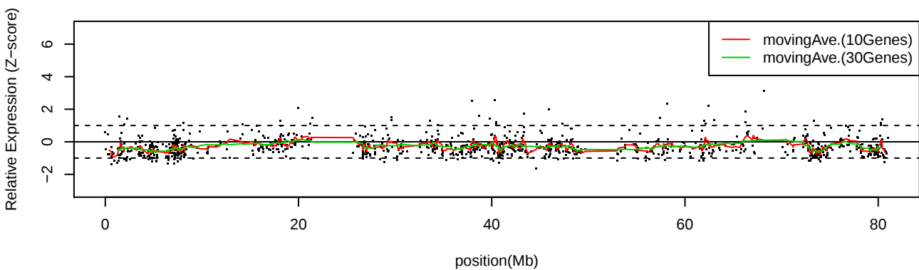
LC_C35 Chr17
