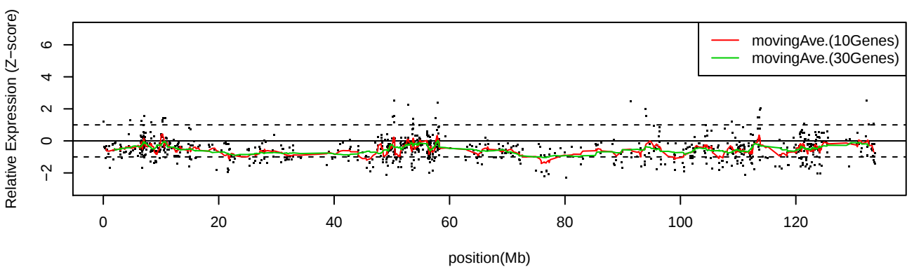
LC_S9 Chr12
