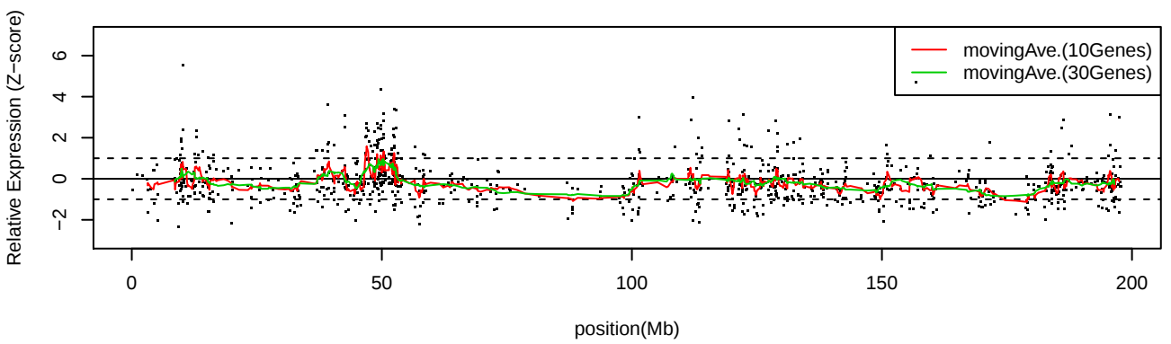
LC_S8 Chr3
