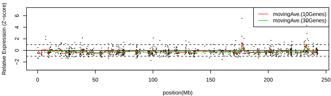
LC_C36 Chr2
