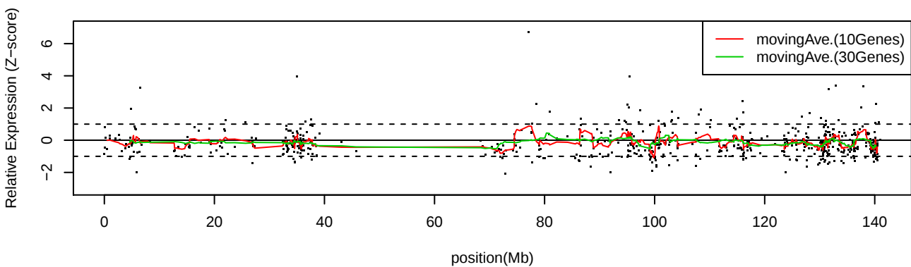
LC_C34 Chr9
