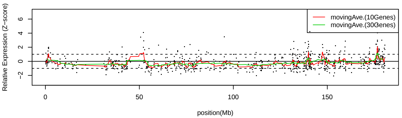
LC_S9 Chr5
