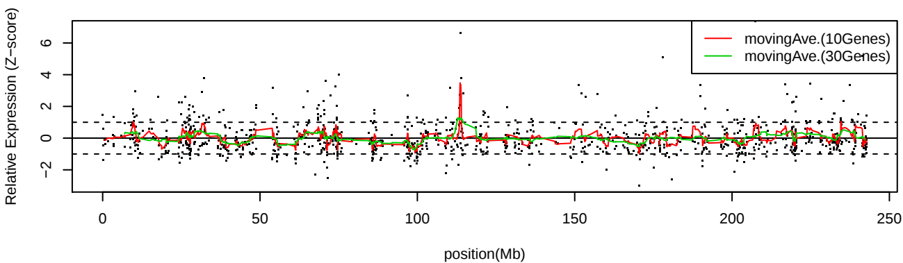
LC_C34 Chr2
