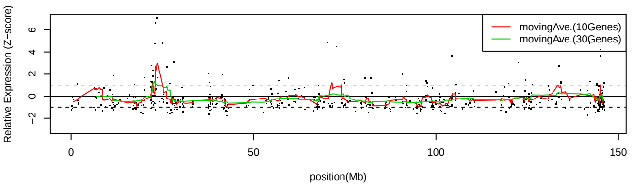
LC_S10 Chr8
