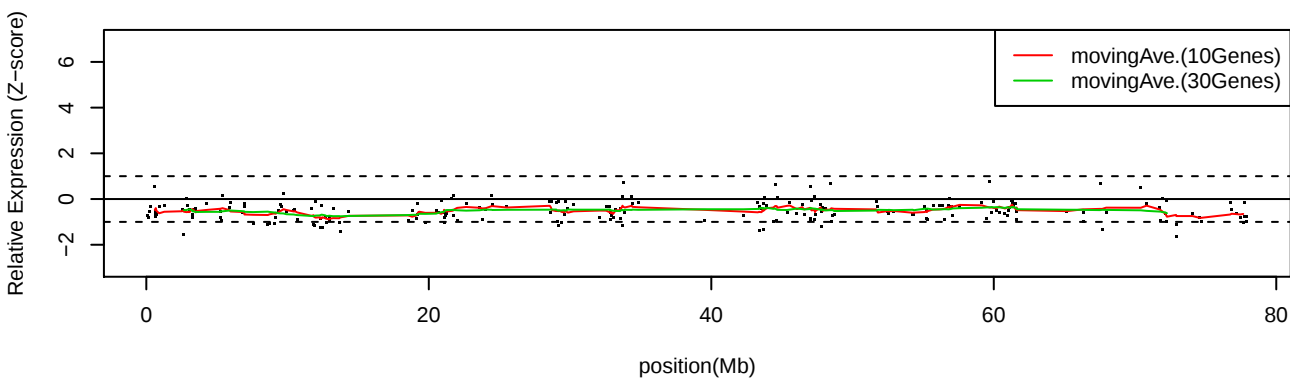
LC_C36 Chr18
