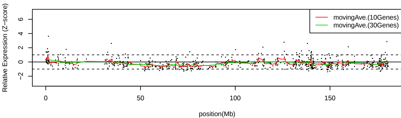
LC_C36 Chr5
