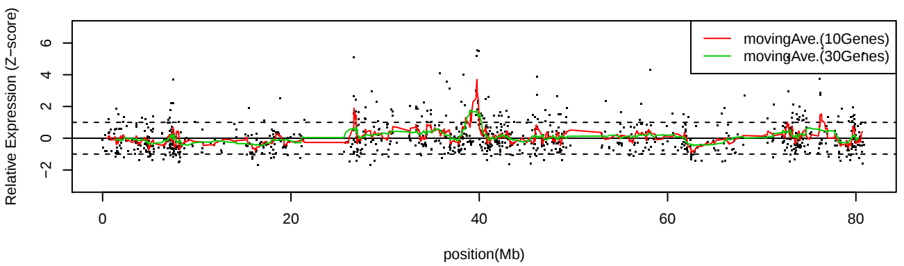
LC_C34 Chr17
