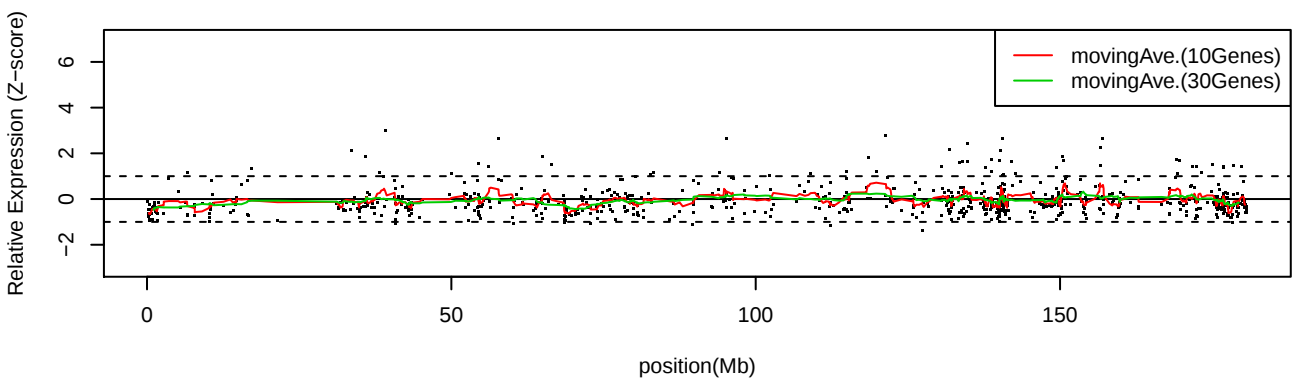
LC_C35 Chr5
