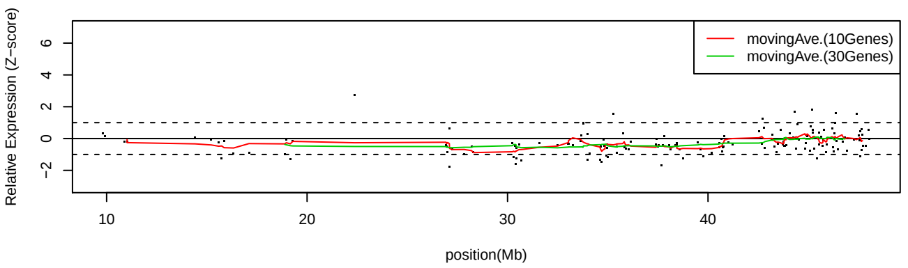
LC_S9 Chr21
