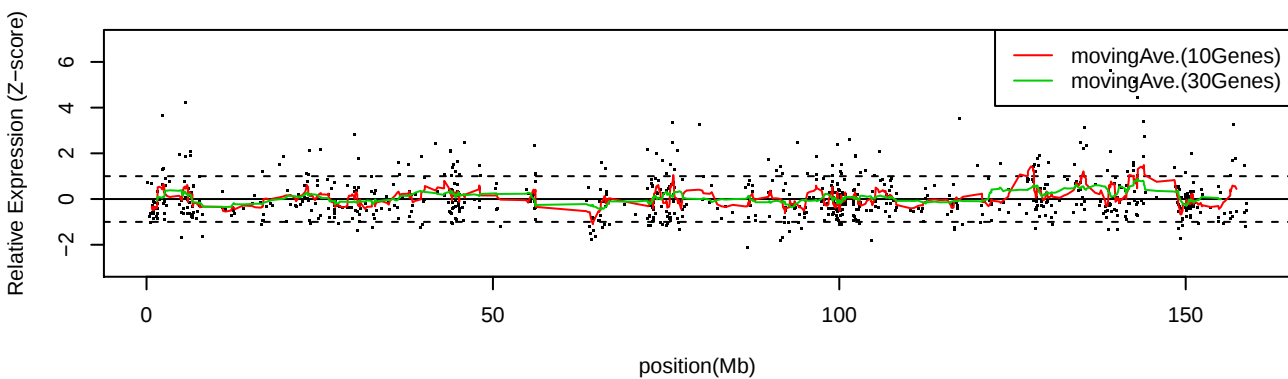
LC_C34 Chr7
