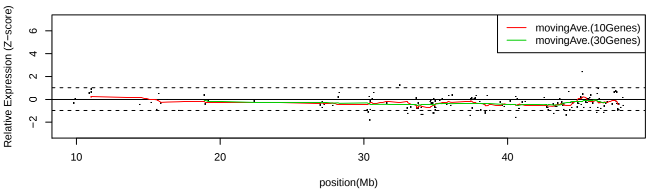
LC_C34 Chr21
