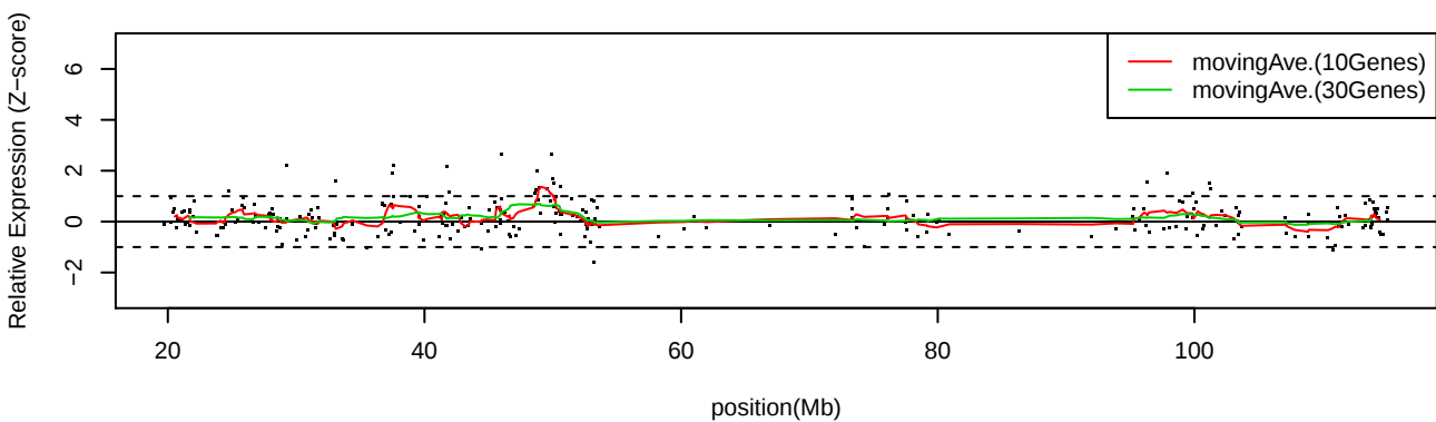
LC_C36 Chr13
