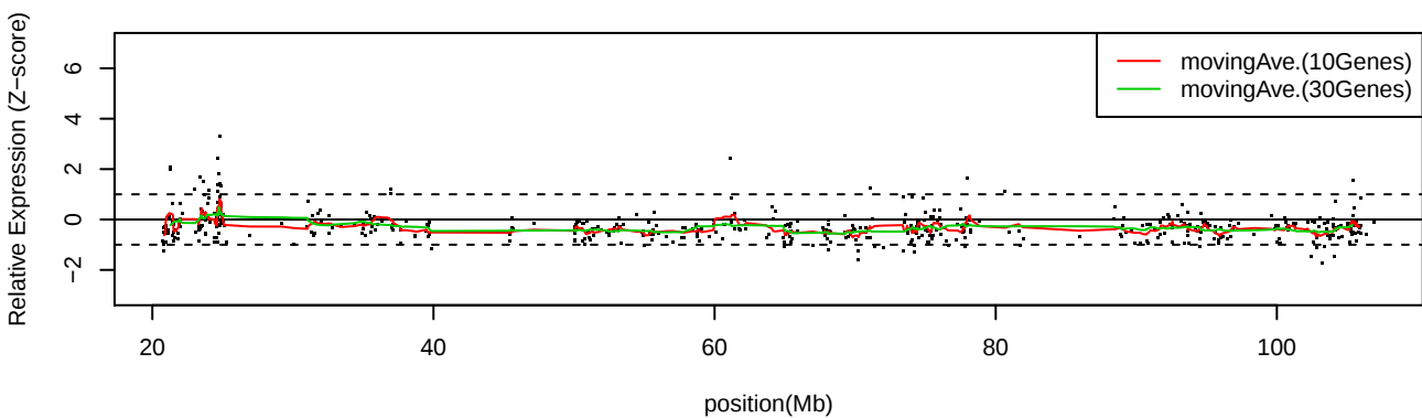
LC_C36 Chr14
