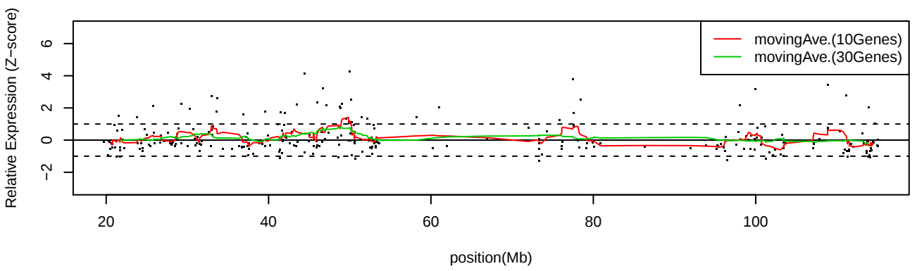
LC_C31 Chr13
