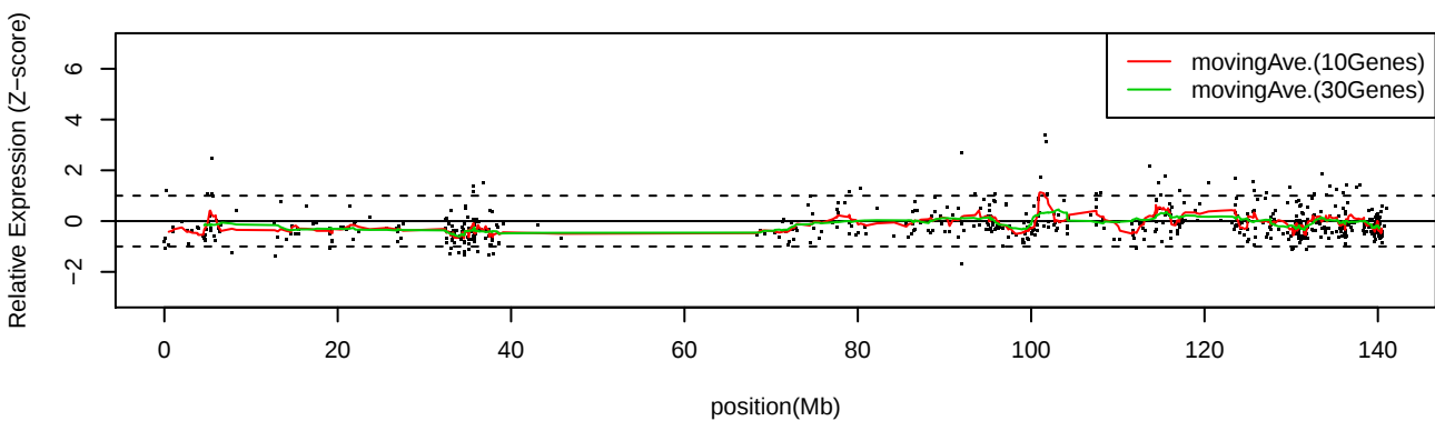
LC_C35 Chr9
