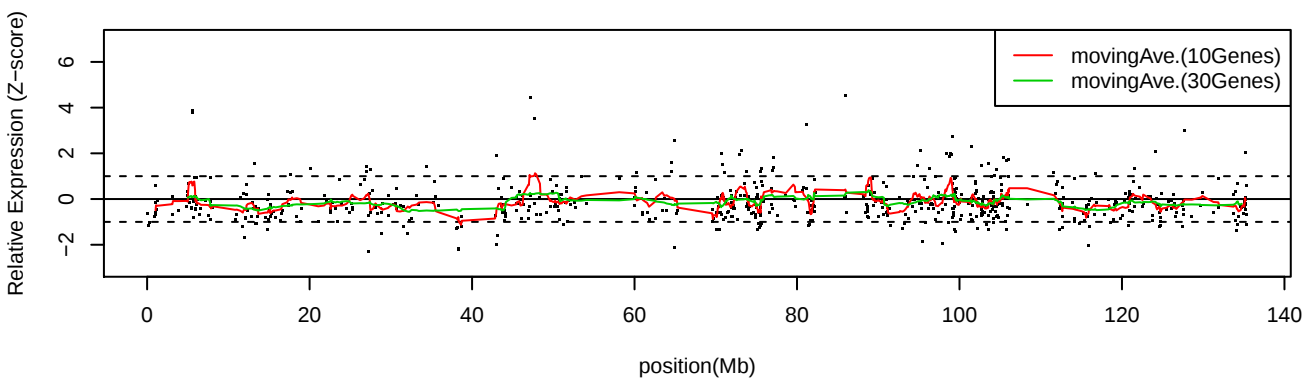
LC_C34 Chr10
