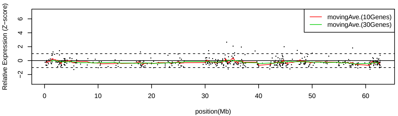
LC_C32 Chr20
