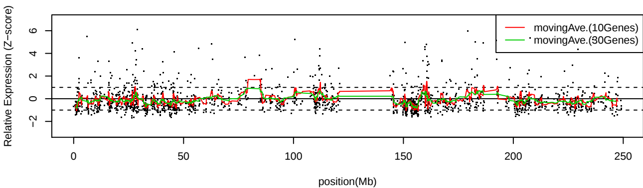
LC_C31 Chr1
