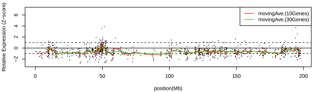
LC_S9 Chr3
