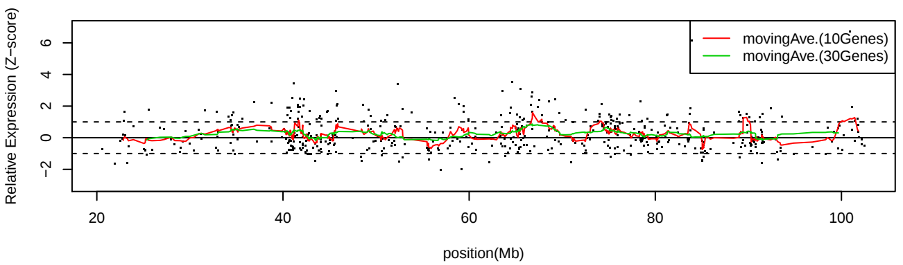
LC_C34 Chr15
