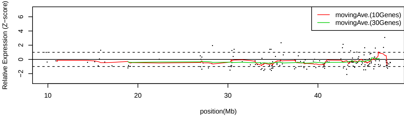
LC_S10 Chr21
