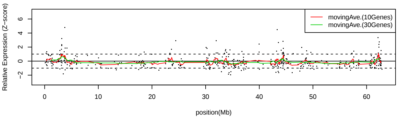
LC_S9 Chr20
