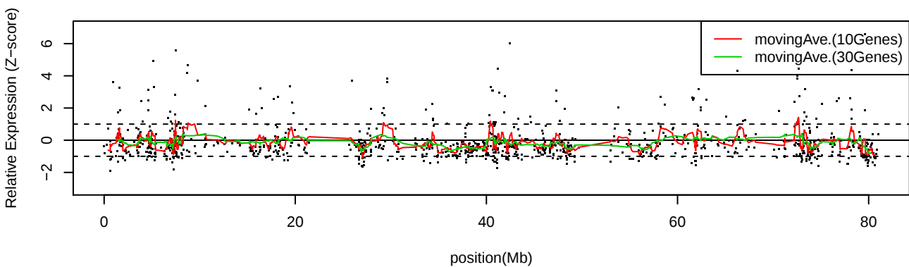
LC_C31 Chr17
