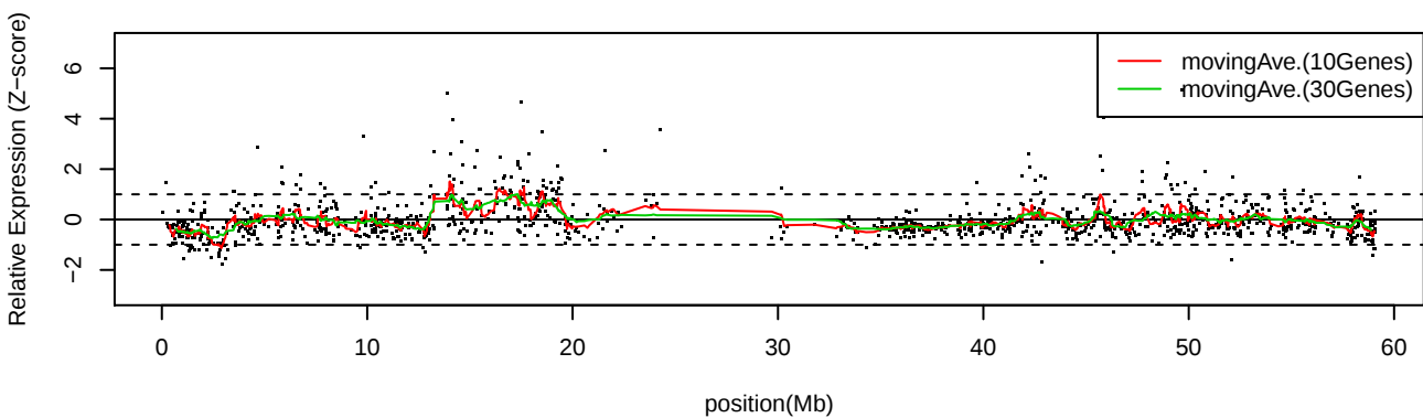
LC_C36 Chr19
