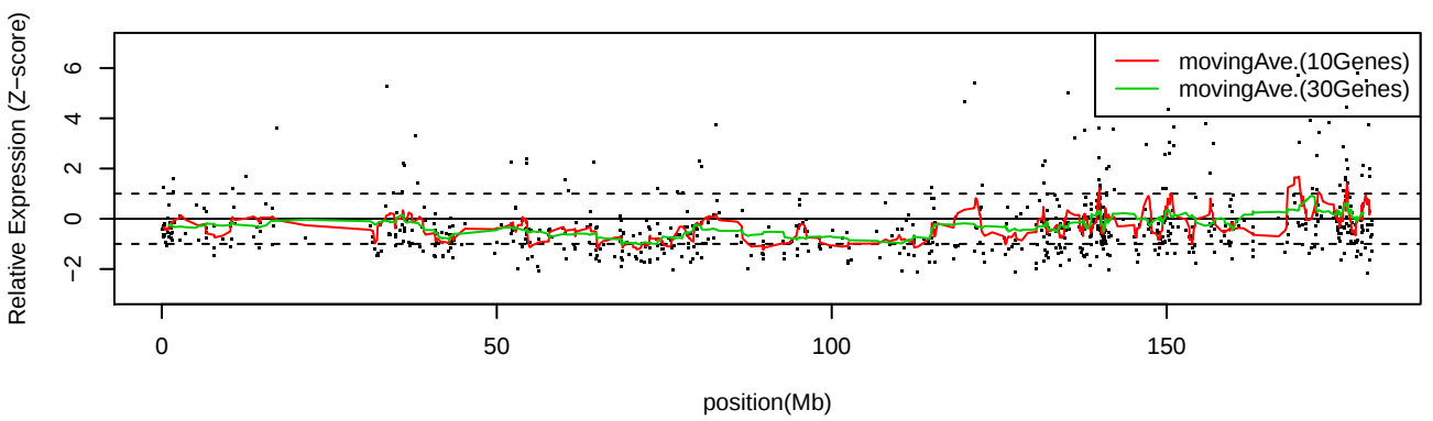
LC_S10 Chr5
