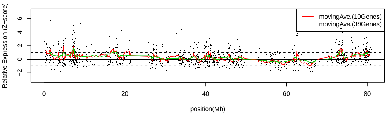
LC_S9 Chr17
