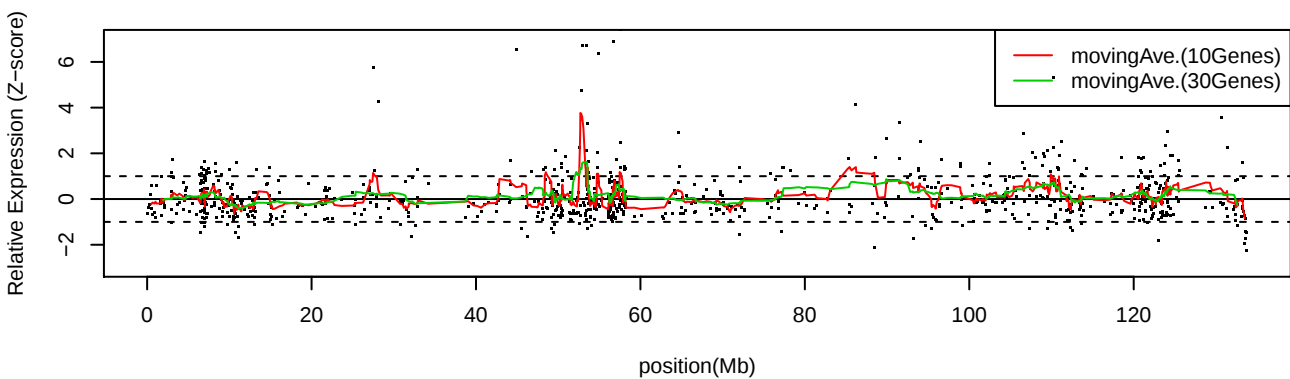
LC_C34 Chr12
