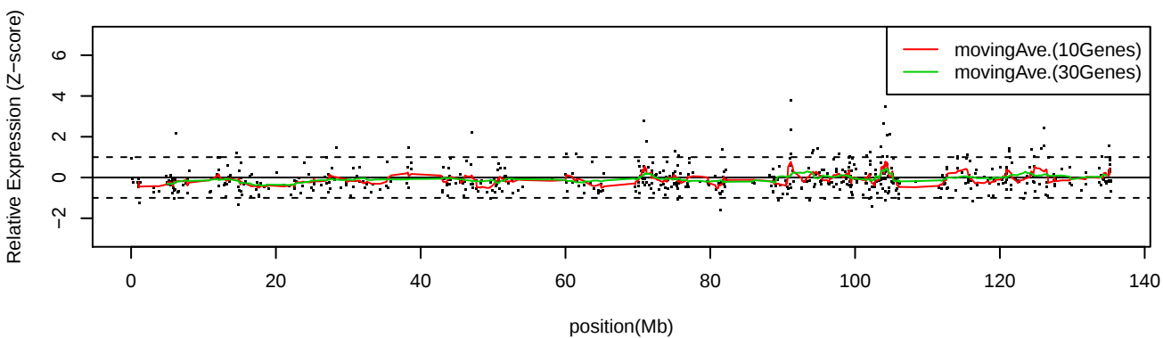
LC_C36 Chr10
