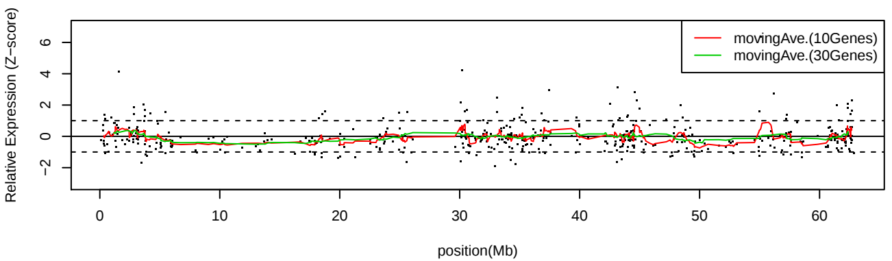
LC_S8 Chr20
