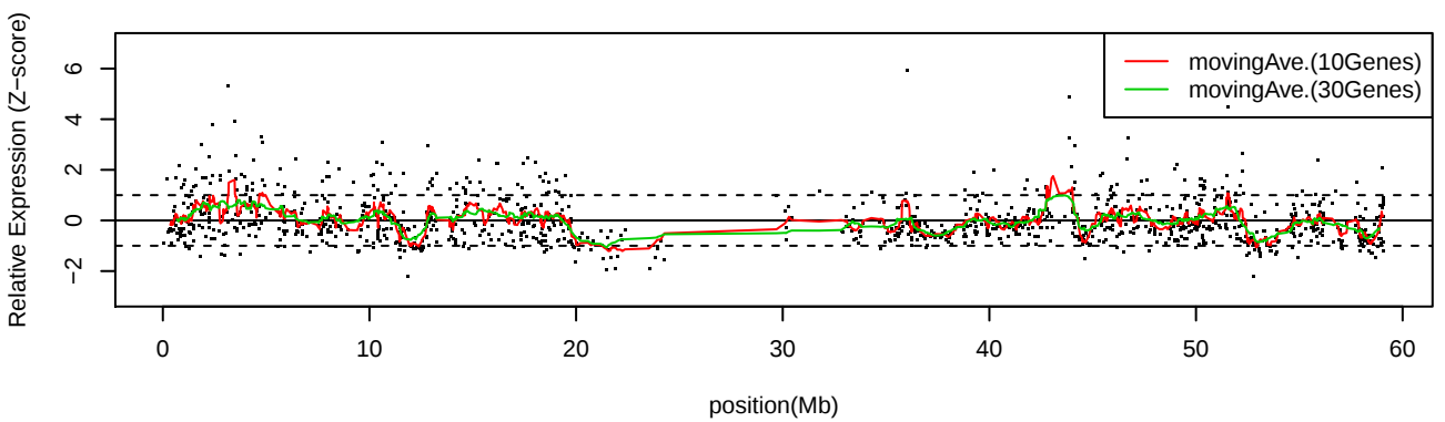
LC_C34 Chr19
