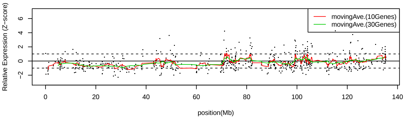
LC_S9 Chr10
