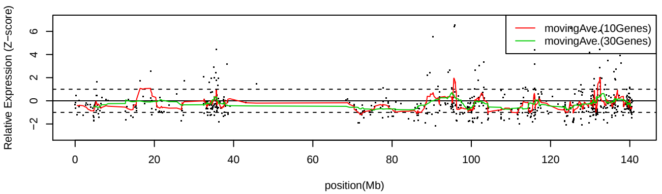
LC_S10 Chr9
