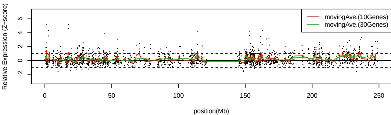
LC_C36 Chr1
