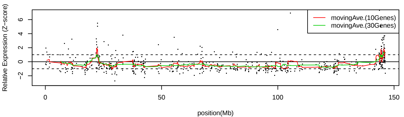
LC_S6 Chr8
