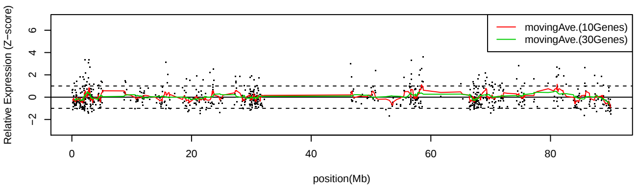
LC_C34 Chr16
