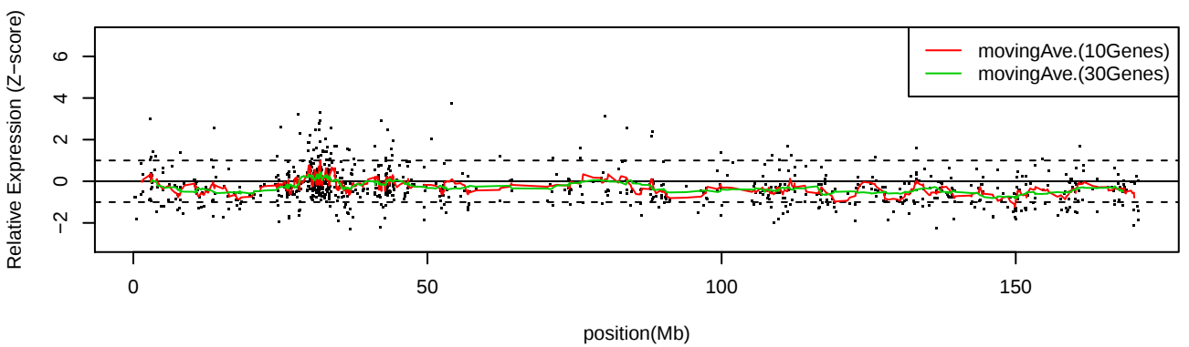
LC_S9 Chr6
