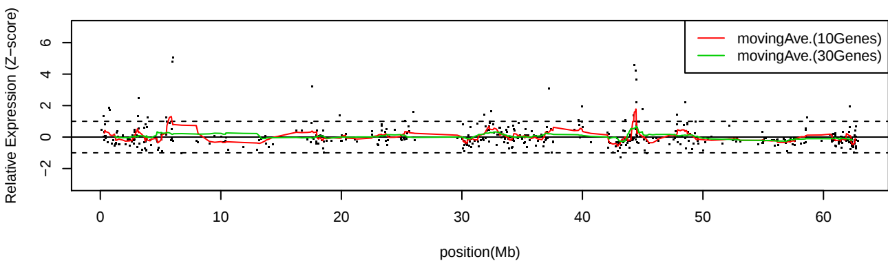
LC_C36 Chr20
