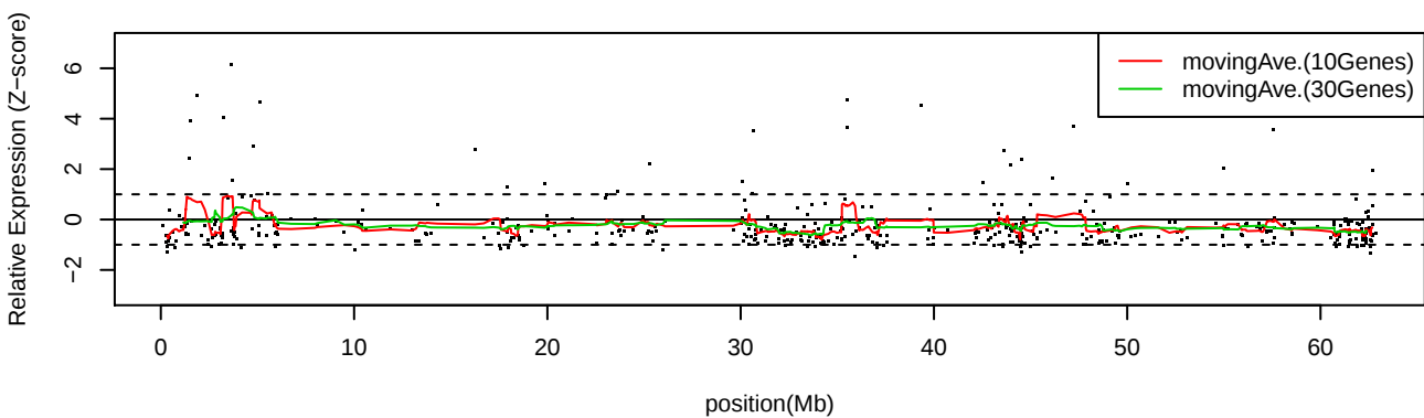
LC_C31 Chr20
