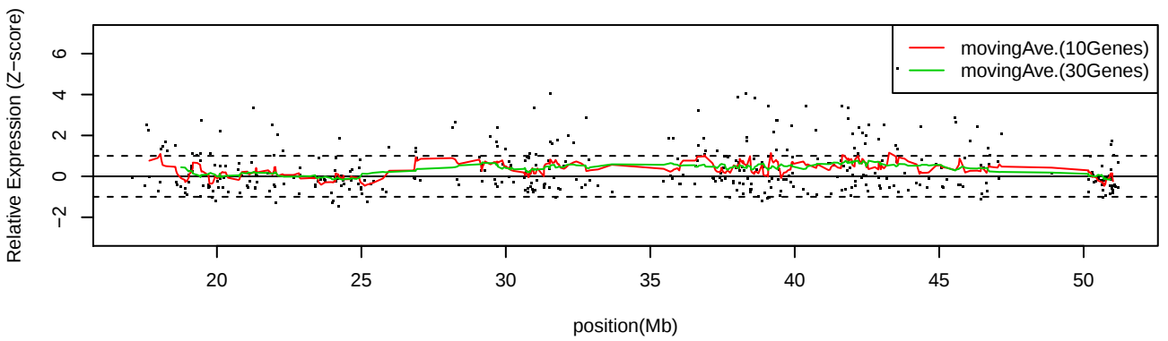
LC_C34 Chr22
