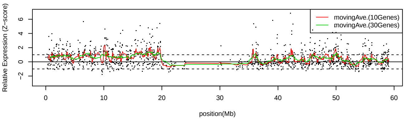
LC_S8 Chr19
