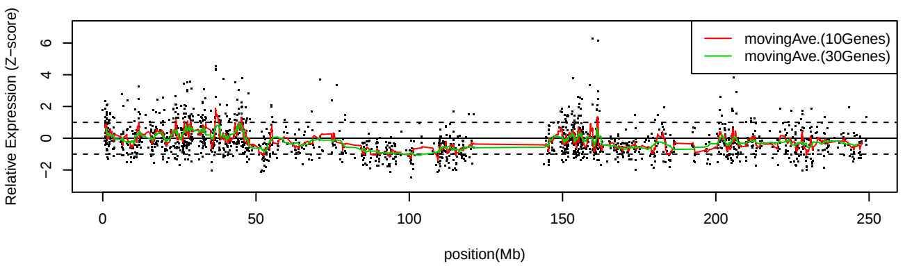
LC_S9 Chr1
