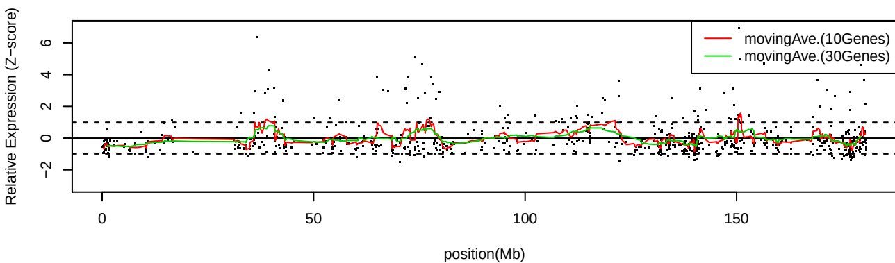
LC_C31 Chr5
