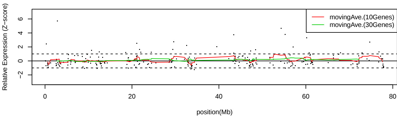
LC_C31 Chr18
