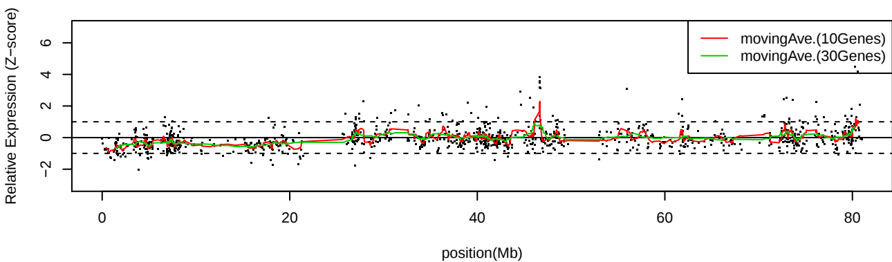
LC_C36 Chr17
