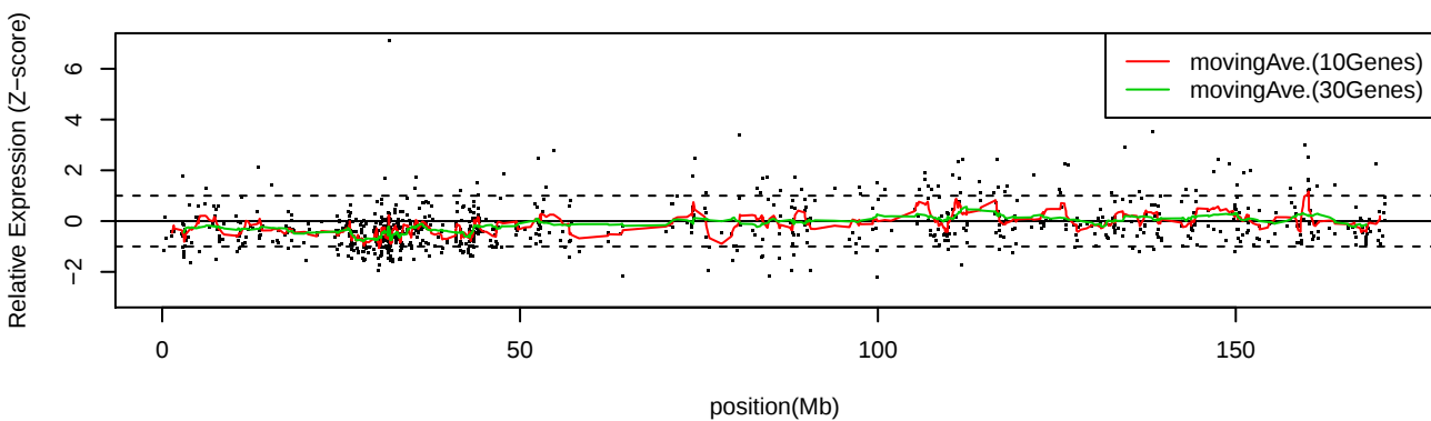
LC_C34 Chr6
