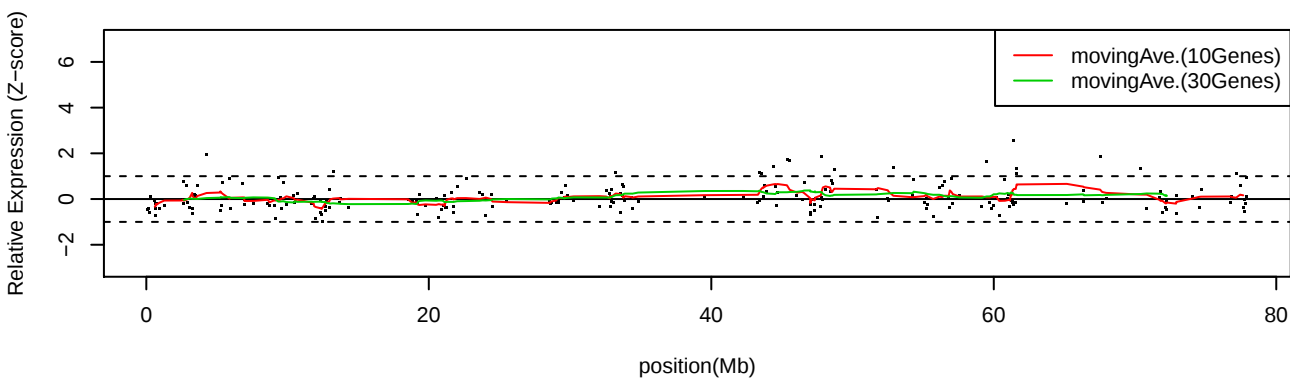
LC_C35 Chr18
