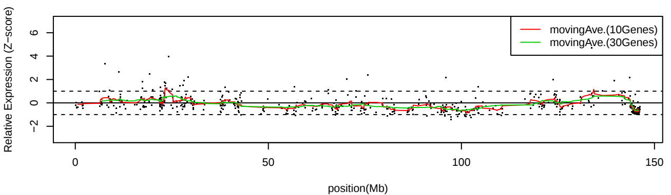
LC_C35 Chr8
