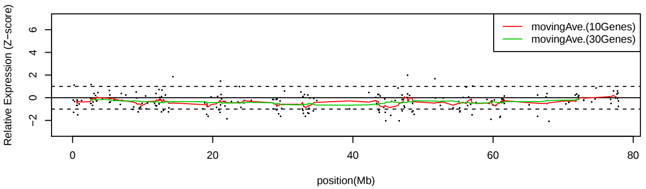
LC_S8 Chr18
