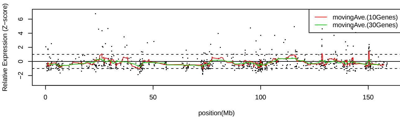
LC_C31 Chr7
