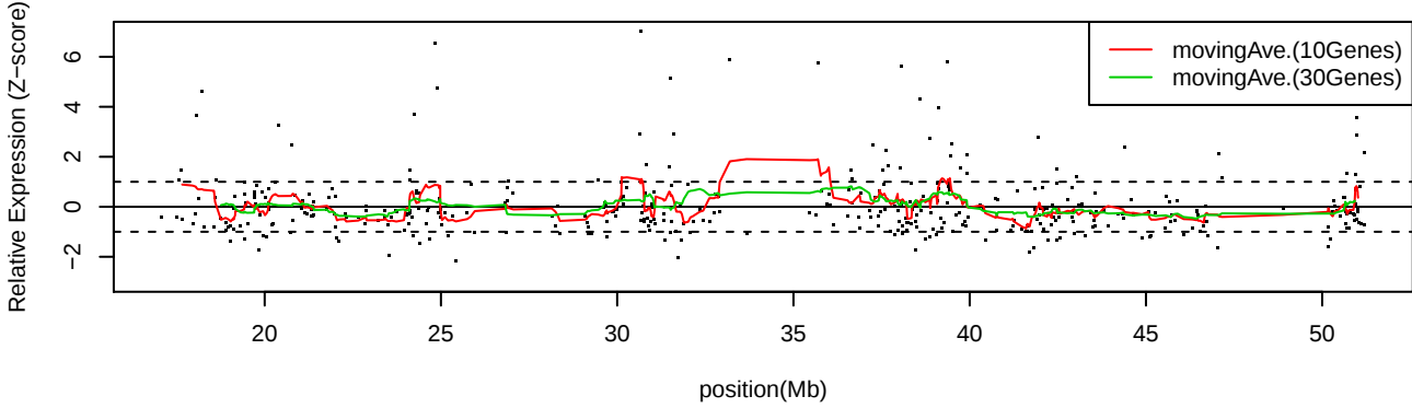
LC_S10 Chr22
