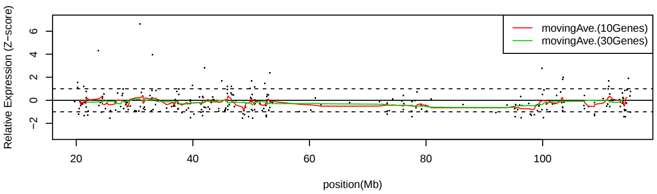
LC_S8 Chr13
