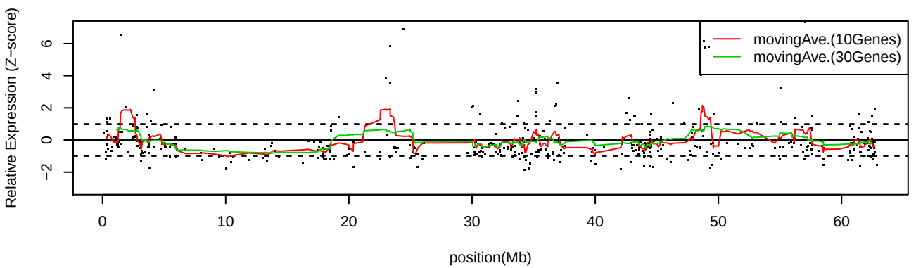
LC_S10 Chr20
