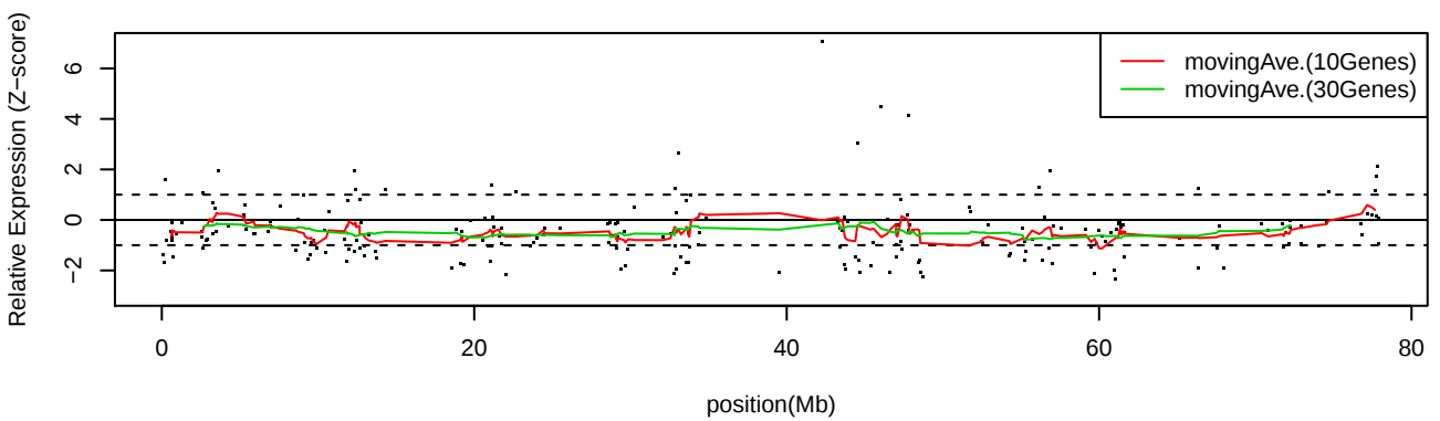
LC_S6 Chr18
