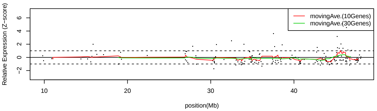
LC_C31 Chr21
