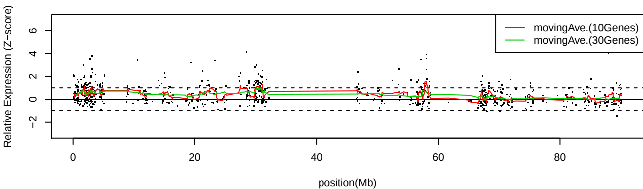
LC_C36 Chr16
