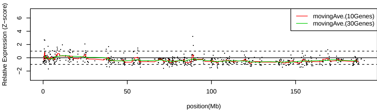
LC_C36 Chr4
