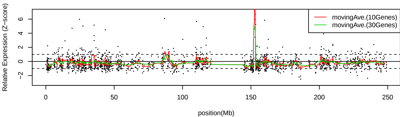
LC_C34 Chr1
