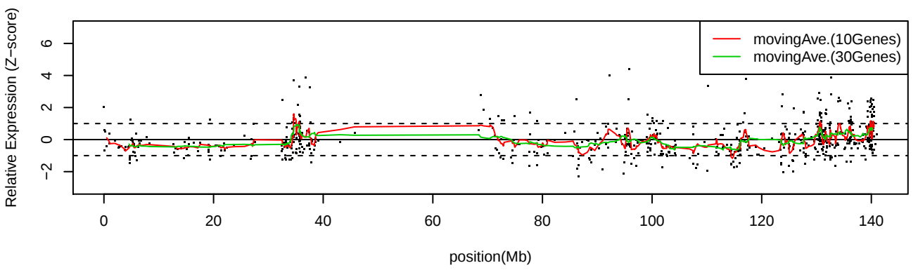
LC_S8 Chr9
