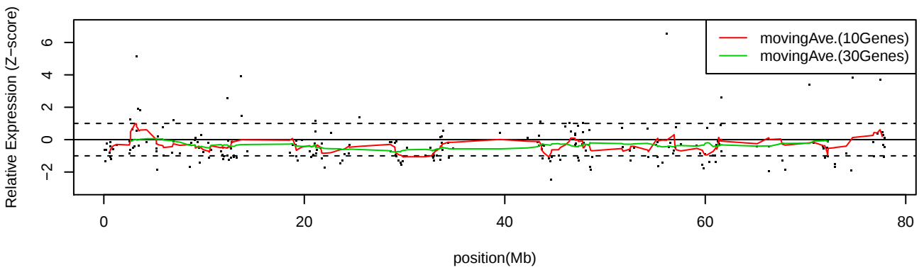
LC_S10 Chr18
