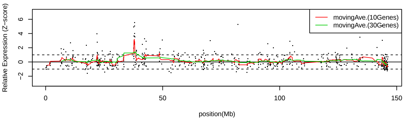
LC_C34 Chr8
