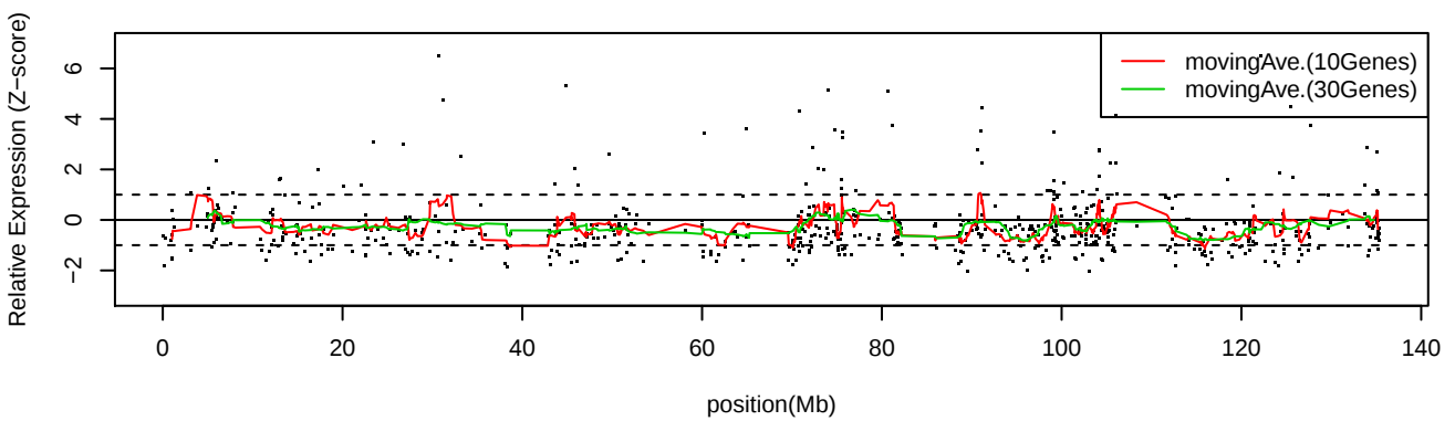
LC_S10 Chr10
