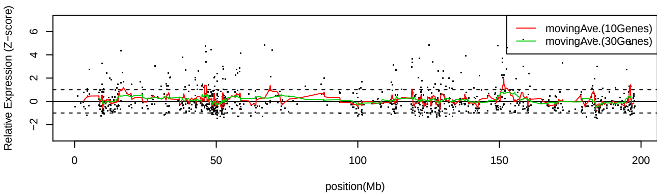
LC_C31 Chr3
