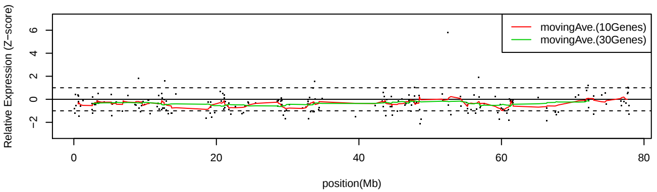
LC_S9 Chr18
