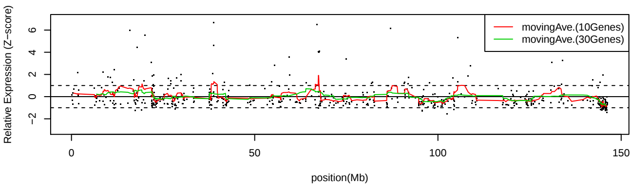
LC_C31 Chr8
