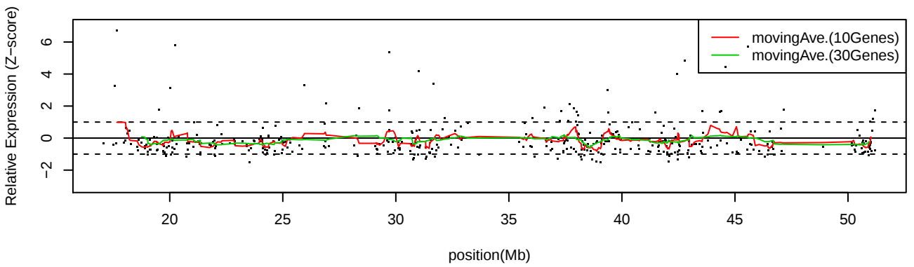
LC_C31 Chr22
