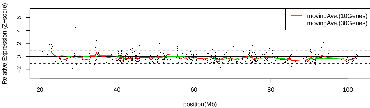
LC_C36 Chr15
