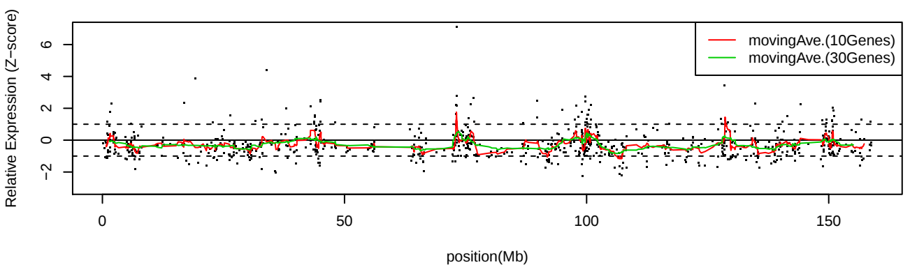
LC_S9 Chr7
