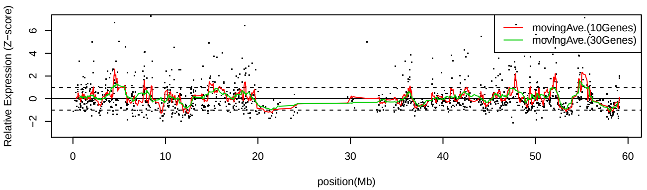
LC_S10 Chr19
