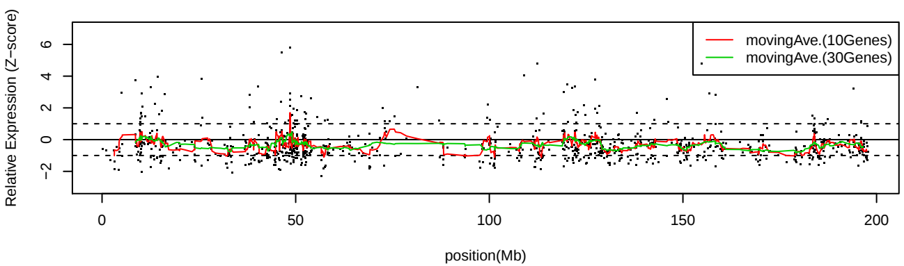
LC_S10 Chr3
