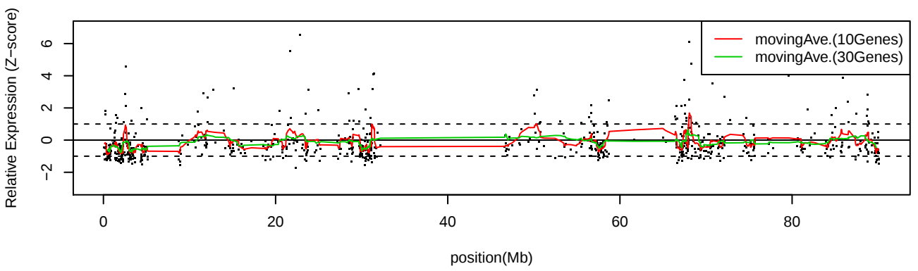
LC_C31 Chr16
