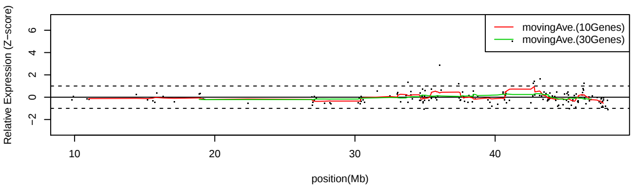
LC_C36 Chr21
