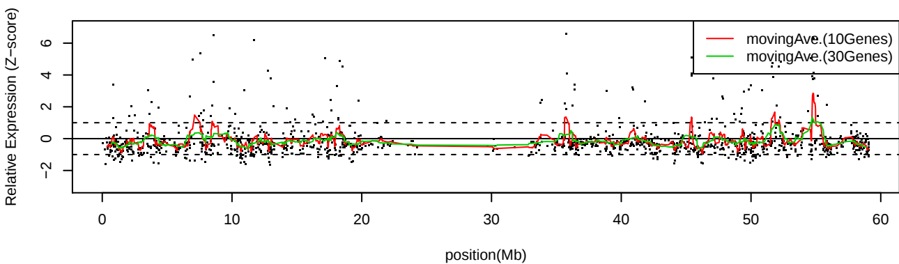
LC_C31 Chr19
