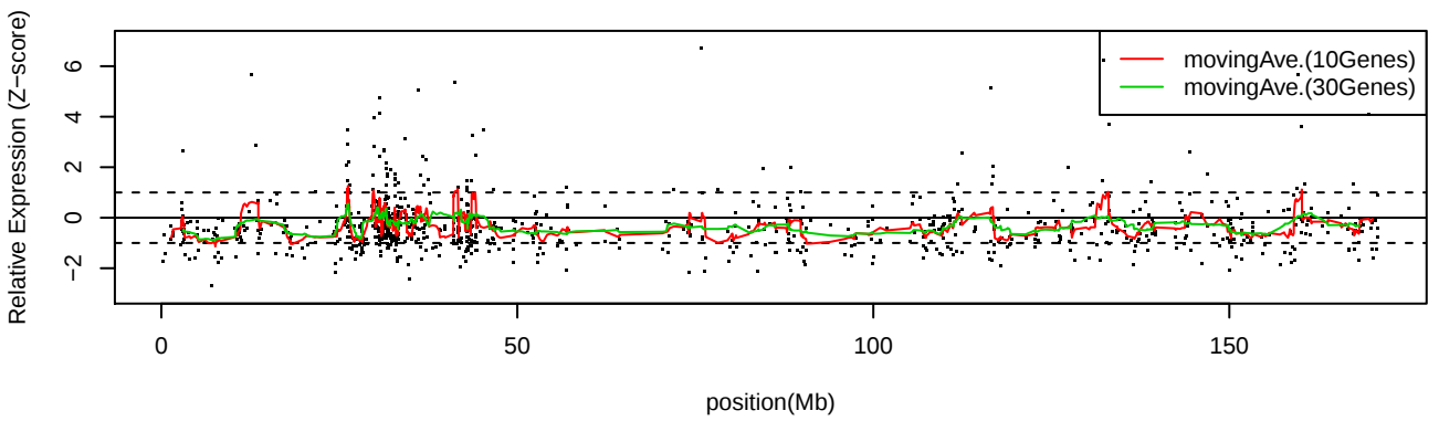
LC_S10 Chr6
