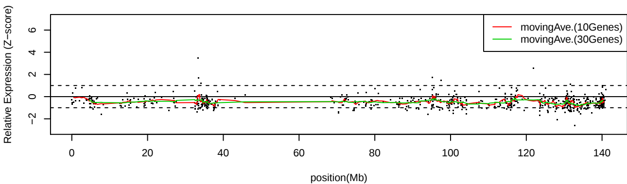
LC_C36 Chr9
