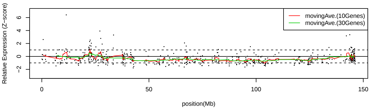
LC_S8 Chr8
