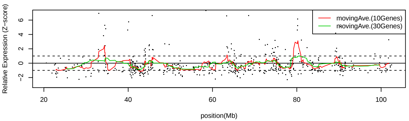
LC_S10 Chr15
