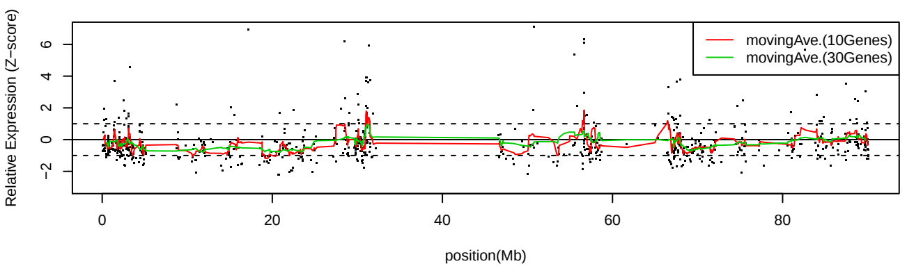
LC_S10 Chr16
