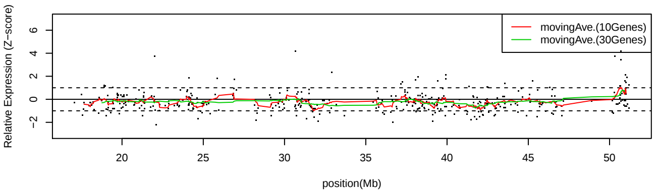
LC_S9 Chr22
