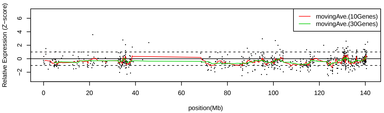
LC_S9 Chr9
