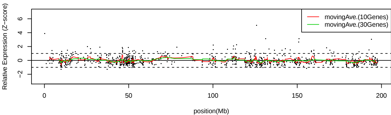
LC_C35 Chr3
