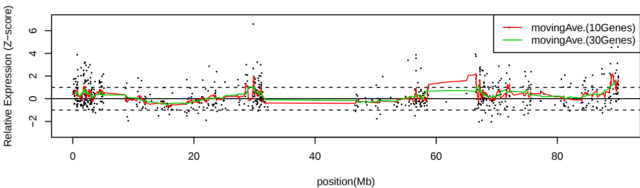
LC_S9 Chr16
