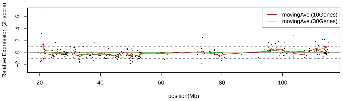
LC_C34 Chr13
